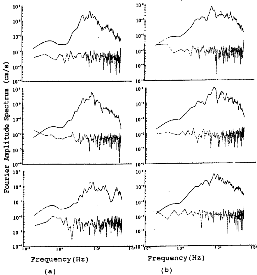
Fig. 8 Fourier amplitude spectra of Event 03, M_L=4.0 , Oct. 4, 1994; (a) surface; (b) downhole;
