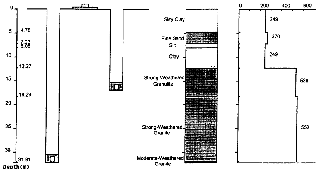
Fig. 4 Earthquake structure and S-wave velocity (m/s) in downhole
