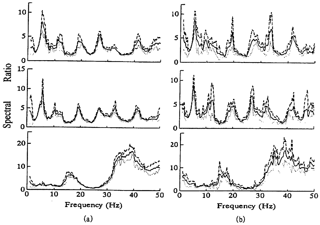
Fig. 11 The mean spectral ratio of 0m/16m: (a) Group one including Event 03, 16, 17, 22, 23, 25; (b) Group two including Event 13, 14, 18, 20, 21, 24. From the top to the bottom is the component R, T and V respectively
