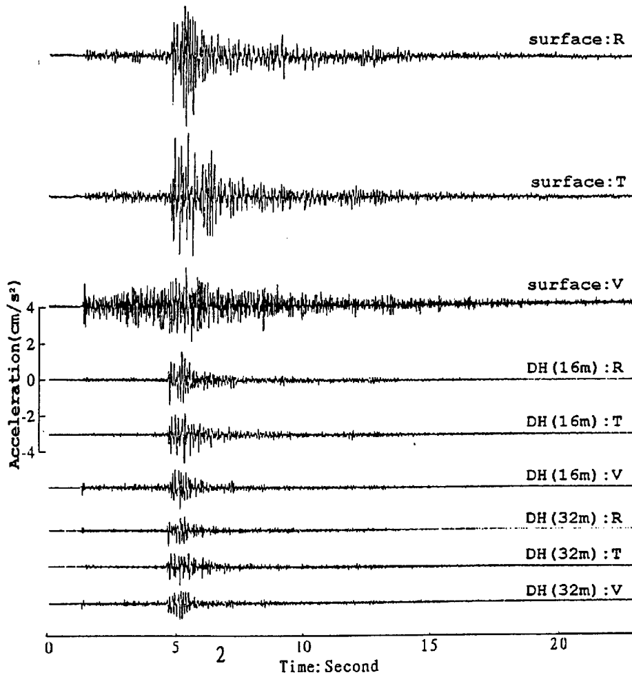
Fig. 7 Accelerograms generated by the Event 17, M_L=3.0 , June 27, 1995; Parameters of the earthquake are: origin time: 06/27/1995, 22:46:18.6 BT; focal depth: 13 km; epicenter location: 39^\circ 44'N , 118^\circ 27'E ; epicenter distance: 24.7 km; backazimuth 280^\circ .
