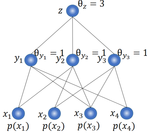
Figure 3: Reduction from a 3-SAT instance \{v_1 \vee v_3 \vee v_4, v_1 \vee v_2 \vee v_3, v_2 \vee v_3 \vee v_4\} to probabilistic rule extraction.
