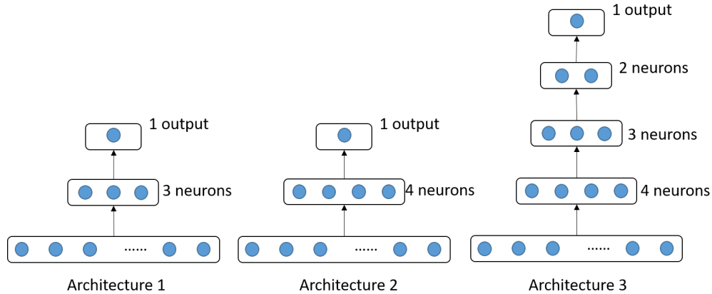
Figure 4: Architectures of the Neural Networks.
