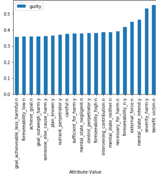
Figure 7: Rules with the Top 20 Highest Probabilities (Moral Reasoner)
