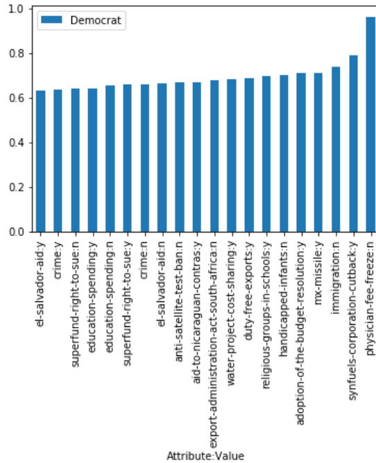
Figure 6: Rules with the Top 20 Highest Probabilities (Vote)
