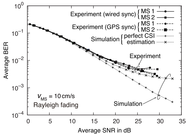
Fig. 10 BER versus SNR performance over the faster Rayleigh fading channel ( v_{MS} = 10 c/ms).
