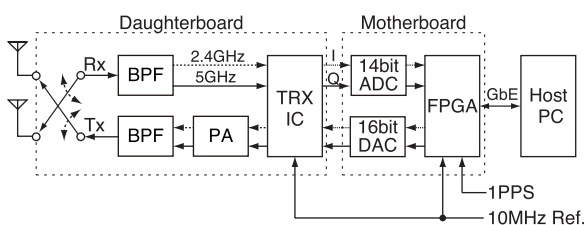
Fig. 4 Block diagram of the USRP.
