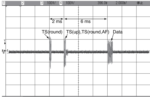
Fig. 7 Timing of packets observed using the oscilloscope.
