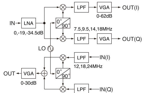
Fig. 5 Block diagram of the transceiver chip.
