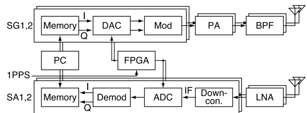
Fig. 1 Block diagram of the base station.
