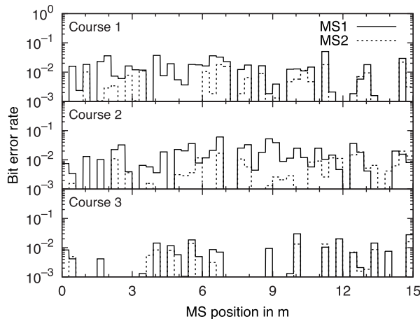
Fig. 14 BER performance for the three MS courses. BER is calculated every 30\text{ cm} \approx 5\lambda .
