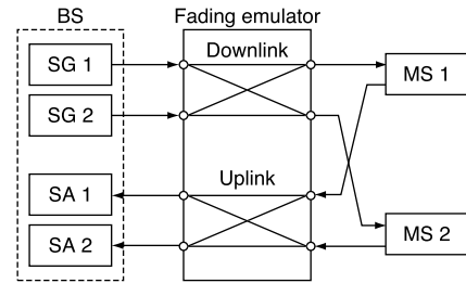
Fig. 8 Experimental setup for in-lab experiments. SGs and SAs of the BS equipment are directly connected with the fading emulator.
