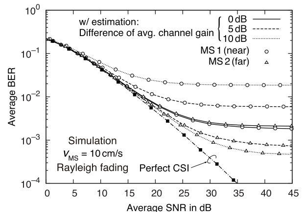
Fig. 17 SNR versus BER performance with channels from/to MS 2 attenuated by 0, 5, 10 dB.
