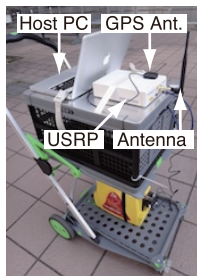
Fig. 3 Mobile station.
