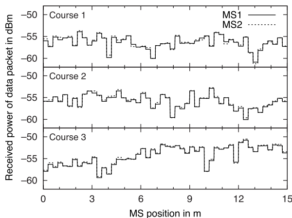
Fig. 15 Received power of precoded data packets for the three MS courses, averaged every 30\text{ cm} \approx 5\lambda .
