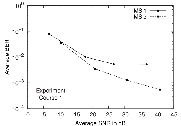
Fig. 16 BER versus SNR performance for Course 1. The horizontal axis shows the received SNR of the data packet averaged over the entire course, i.e., 15 m. The transmit power of the first training packet is fixed. The transmit power of the precoded data packet is attenuated by 0, 10, 20, and 30 dB.
