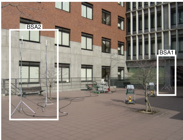
Fig. 11 Environment for the field experiments.
