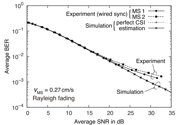
Fig. 9 BER versus SNR performance over the slow Rayleigh fading channel ( v_{MS} = 0.27 c/ms).
