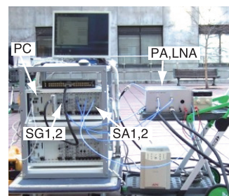
Fig. 2 Base station.
