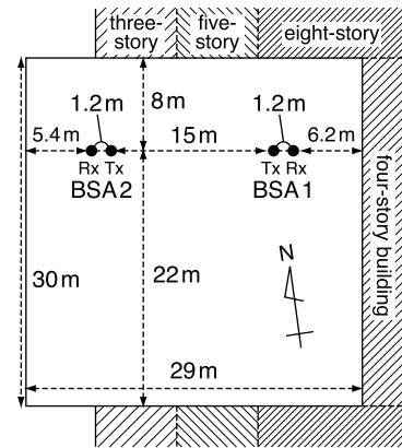
Fig. 12 Layout of the experimental location.
