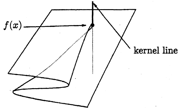
FIGURE 3. The kernel line at a cusp
