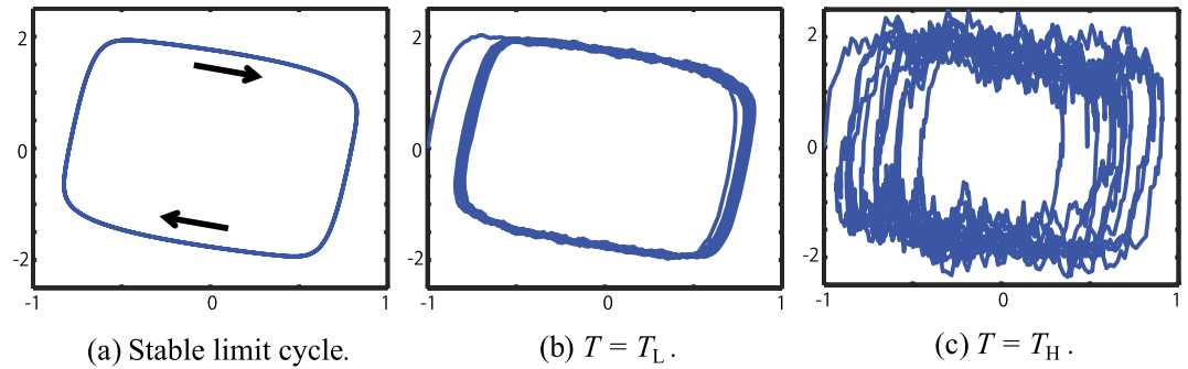
Figure 2. A phase portrait of the FitzHugh-Nagumo neuronal oscillator in the (v, w) -plane. (a) The stable limit cycle of the noise-free individual dynamics. (b) A sample path of v_i(t) for T = T_L . (c) A sample path of v_i(t) for T = T_H .
