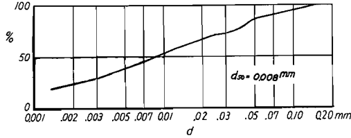
Fig. 6. Cumulative diagram of grain size distribution of sediment used.
