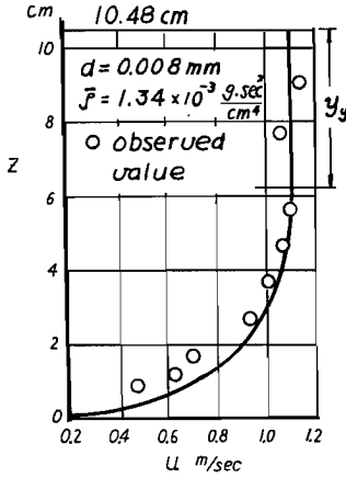
Fig. 8. Comparison of velocity profiles obtained by experiment and theory.
