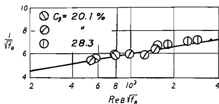
Fig. 12. Relation between 1/\sqrt{f_R} and Re_B/\sqrt{f_R} for Bingham flow in pipes.
