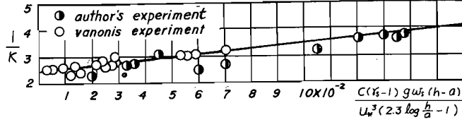
Fig. 14. Relation between 1/K and \frac{c(\tau_s-1)gw_s(h-a)}{u_*^3(2.3 \log \frac{h}{a}-1)}
