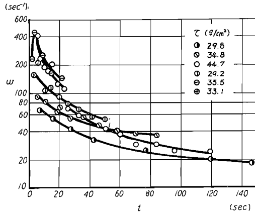
Fig. 3. Relations between angular velocity \omega and time t .
