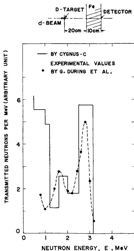
Fig. 8. Comparison between CYGNUS-C- calculated and measured spectrum 10) transmitted through iron slab. The spectrum has not been normalized.
