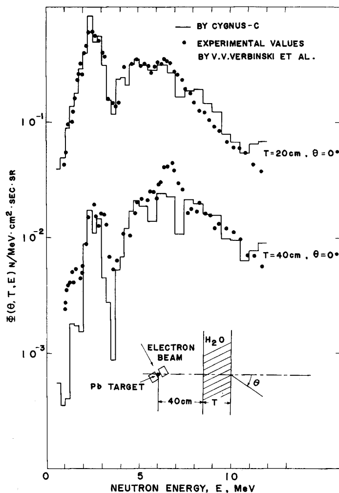
Fig. 7. Comparison between CYGNUS-C-calculated and measured spectra 9) transmitted through water slab. The CYGNUS-C-calculated spectra have been normalized to a single point at 5 MeV on the measured 20 cm spectrum.
