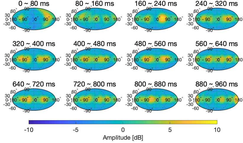
Figure 9: Condition F (Acoustic coefficient for the floor surface: 0.8, and that for the other surface: 0.2, Sound source position: S2)
