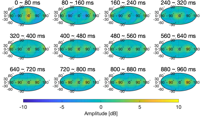
Figure 7: Condition D (Acoustic coefficient for all surface: 0.2, Sound source position: S1)
