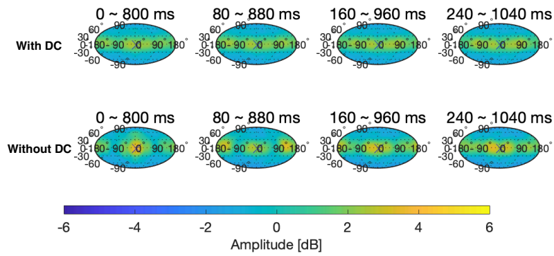
Figure 14: Condition A analyzed with (upper row) and without (lower row) decay cancellation (DC) (800 ms time window)
