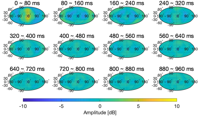
Figure 8: Condition E (Acoustic coefficient for all surface: 0, Sound source position: S1)
