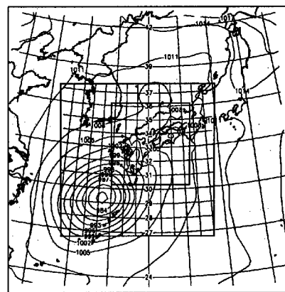
Fig.6. MM5 grid configuration for the 45km, 15km and 5km grids of domains in case Zeb, and sea level pressure field at initial time of the run.
