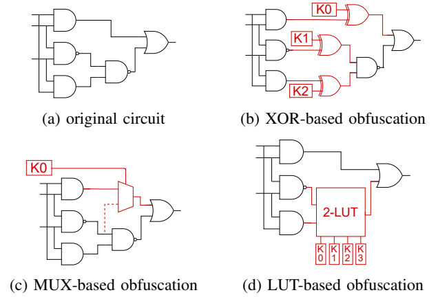
Fig. 2: Logic locking.
