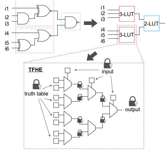
Fig. 1: Conceptual overview of the proposed LUT-based logic locking over TFHE. The inputs i1 to i6 and the logic locking keys, which are truth table values, are encrypted. The encrypted output value is obtained without decryption.
