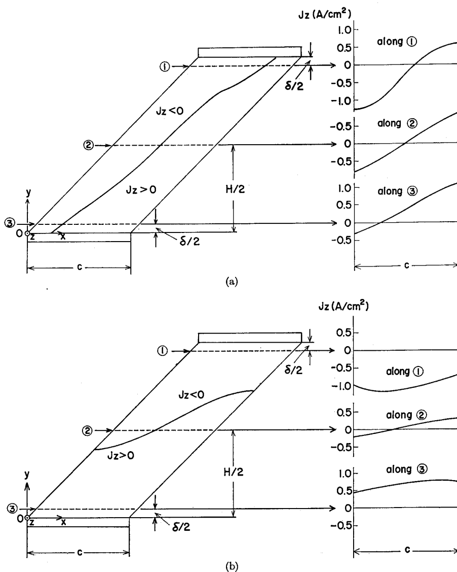
Fig. 10. Current distributions at z=\delta/2 near sidewall electrode of DCW generator.
