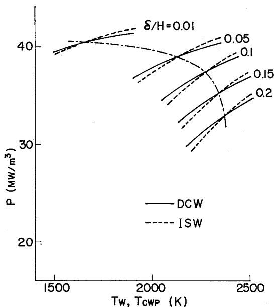
Fig. 8. Influence of \delta/H on P and T_{cwp} when s/H = 0.1 and \phi = 45^\circ .
