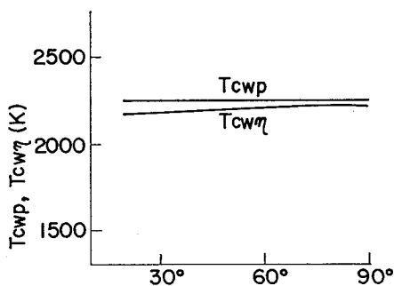
Fig. 7. Influence of \phi on T_{cwp} and T_{cw\eta} when s/H = \delta/H = 0.1 .
