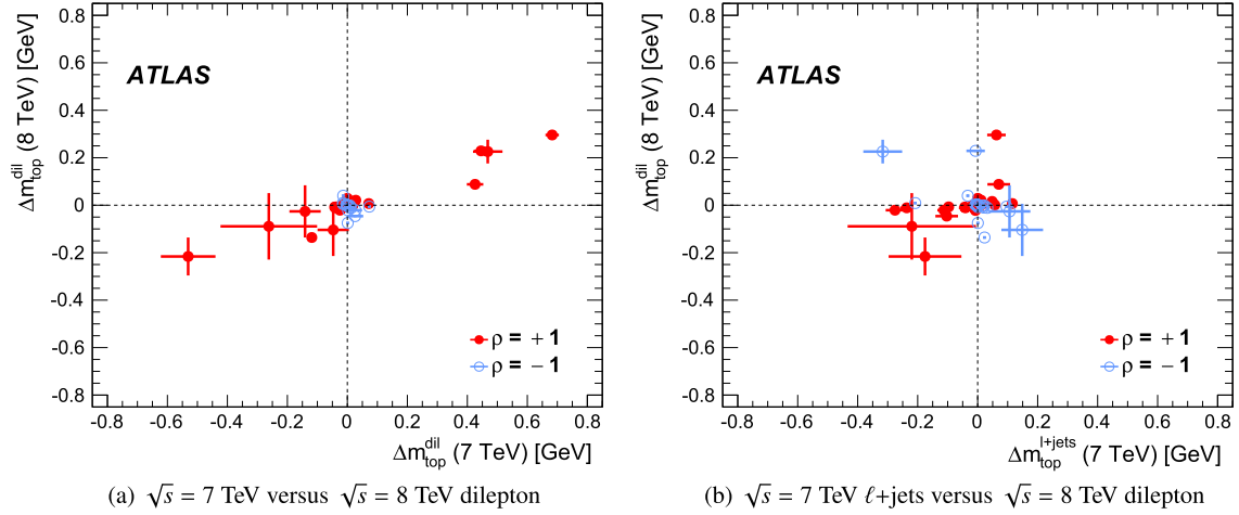
Fig. 3. The pairwise differences in m_{\text{top}} when simultaneously varying both analyses for a systematic uncertainty. Each cross indicates the statistical precisions of the systematic uncertainty. The red full points indicate \rho = 1 , the blue open points \rho = -1 .
