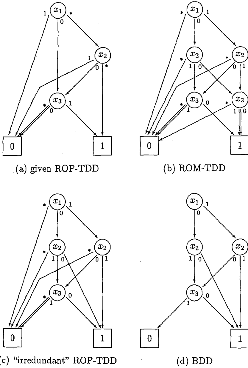
Figure 4.11: Convert ROP-TDD into BDD
