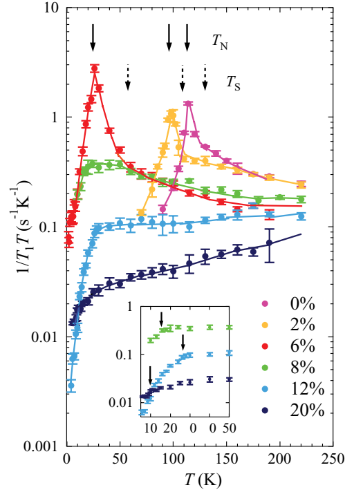
FIG. 4. (Color online) Temperature dependence of 1/T_1 T measured at the lower-field edge at 45 kOe in the main panel of Fig. 3. The arrows at peak positions and bending points represent antiferromagnetic ( T_N ) and structural ( T_S ) transition temperatures, respectively. The inset shows the expansion in the low-temperature range; the arrows indicate T_c .
