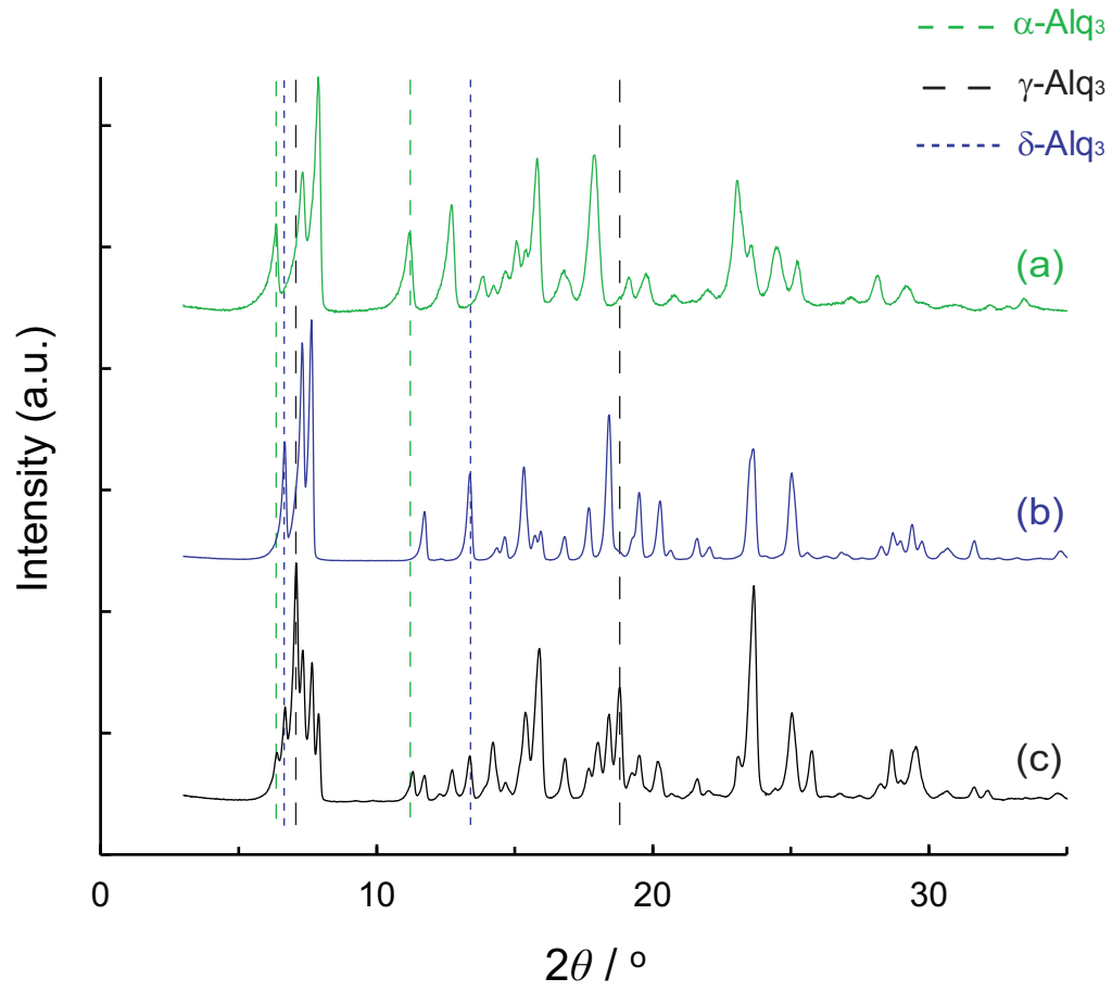
Fig. 3.2. X-ray diffraction profiles of (a) \alpha -Alq 3 , (b) \delta -Alq 3 , and (c) the mixture of \alpha -, \gamma -, and \delta -Alq 3 . Some diffraction peaks representative of \alpha -Alq 3 , \gamma -Alq 3 , and \delta -Alq 3 are indicated by vertical dashed lines in the figure.
