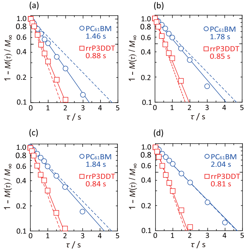
Fig. 7.9. T_{1H} relaxation behaviors of rrP3DDT (open squares) and PC 61 BM (open circles) components in rrP3DDT/PC 61 BM blends; (a) nonannealed, annealed at 150 °C for (b) 5 min, (c) 15 min, and (d) 30 min. T_{1H} values are written in each figures. T_{1H} relaxation behaviors of pure rrP3DDT and pure PC 61 BM with annealed 150°C for 60 min are also shown as broken lines for references.
