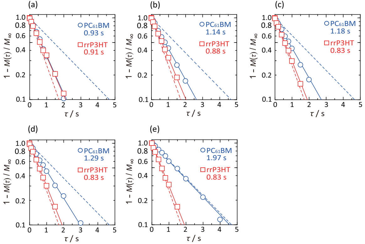
Fig. 7.8. T_{IH} relaxation behaviors of rrP3HT (open squares) and PC 61 BM (open circles) components in rrP3HT/PC 61 BM blends; (a) nonannealed, annealed at 150 °C for (b) 5 min, (c) 15 min, (d) 30 min, and (e) 45 min. T_{IH} values are written in each figures. T_{IH} relaxation behaviors of pure rrP3HT and pure PC 61 BM with annealed 150°C for 60 min are also shown as broken lines for references.
