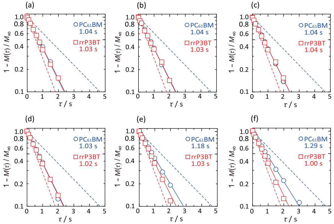
Fig. 7.7. T_{IH} relaxation behaviors of rrP3BT (open squares) and PC 61 BM (open circles) components in rrP3BT/PC 61 BM blends; (a) nonannealed, annealed at 150 °C for (b) 5 min, (c) 15 min, (d) 30 min, (e) 45 min, and (f) 60 min. T_{IH} values are written in each figures. T_{IH} relaxation behaviors of pure rrP3BT and pure PC 61 BM with annealed 150°C for 60 min are also shown as broken lines for references.
