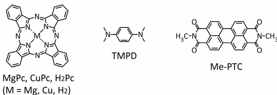
Fig. 1.3. Chemical structures of organic semiconductor materials: phthalocyanine derivatives (MgPc, CuPc, H 2 Pc), tetramethyl p -phenylenediamine (TMPD), and N -methyl-3,4,9,10-perylenetetracarboxyl-diimide (Me-PTC).
