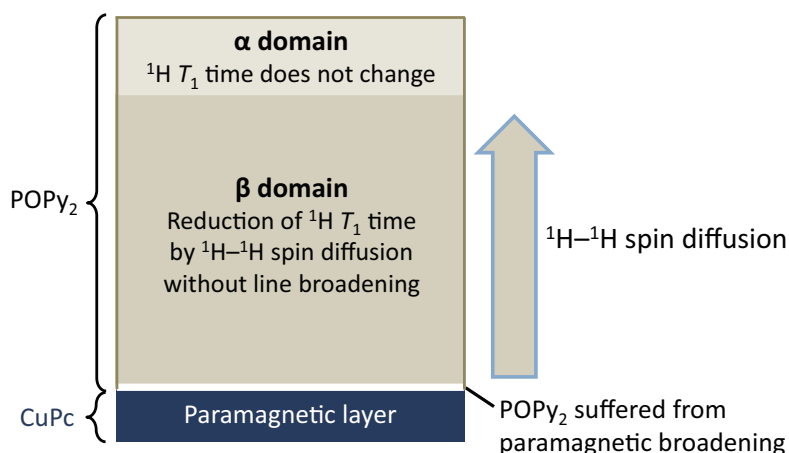
Fig. 4.1. Schematic representation of ^1\text{H} T_1 reduction in POPy 2 thin organic films with paramagnetic dopant (CuPc).
