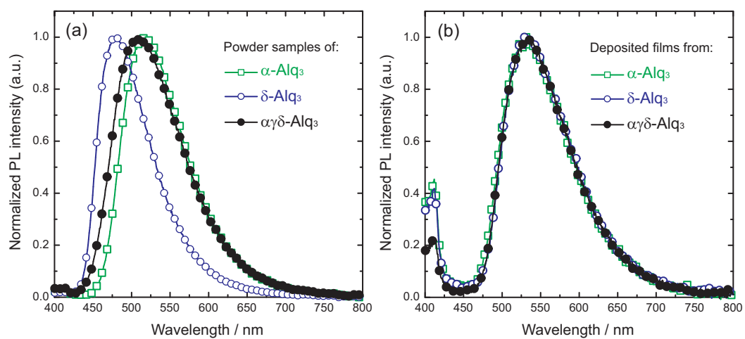
Fig. 3.5. Normalized PL spectra of (a) the three types of \text{Alq}_3 powder samples used in this study, \alpha\text{-Alq}_3 , \delta\text{-Alq}_3 , and the mixture of \alpha -, \gamma -, and \delta\text{-Alq}_3 , and (b) their deposited films. The excitation wavelength is 375 nm.
