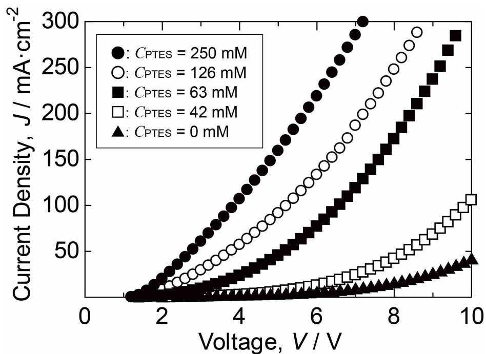
Fig. 5.6. Influence of C_{\text{PTES}} on J - V characteristics of HODs composed of ITO-SAM/NPD 100 nm/Al 100 nm; closed circles: 250 mM, open circles: 126 mM, closed squares: 63 mM, open squares: 42 mM, closed triangles: 0 mM. 0.01 M \text{HNO}_3 was used as a catalyst and r = 15 for all the devices.
