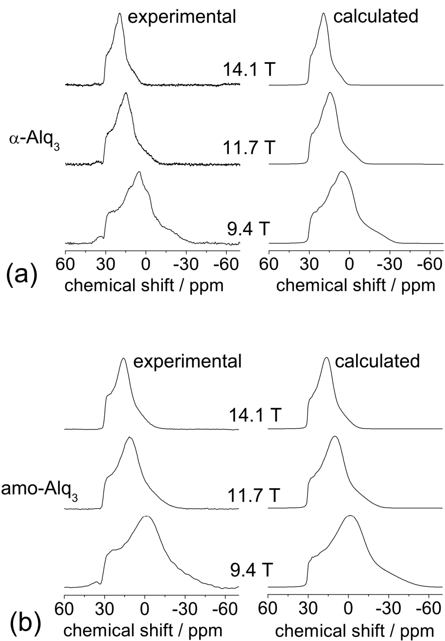
Fig. 2.5. Experimental (left) and calculated (right) ^1\text{H} decoupled ^{27}\text{Al} MAS NMR spectra of (a) \alpha\text{-Alq}_3 and (b) \text{amo-Alq}_3 .
