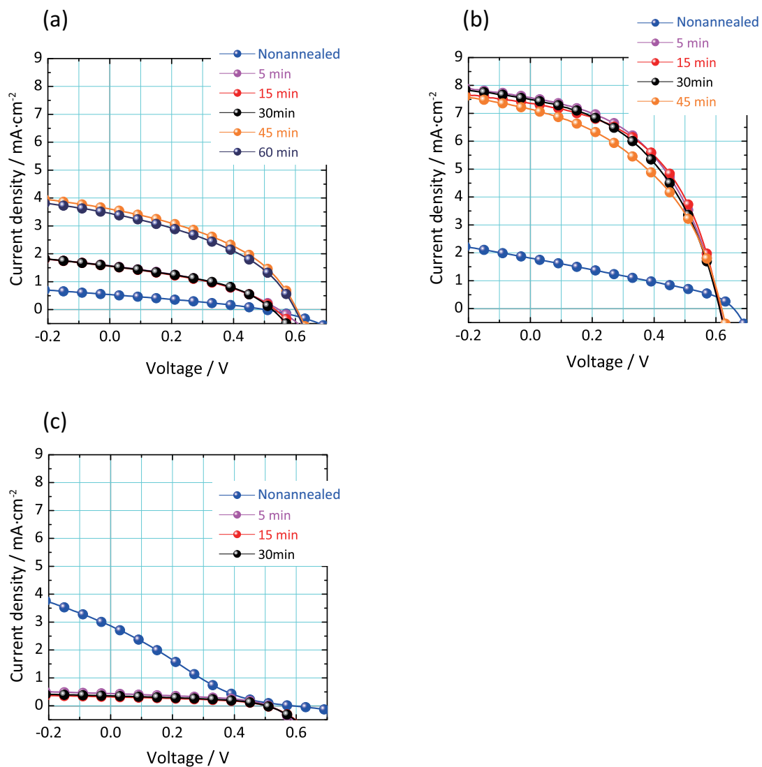
Fig. 7.2. Current density–voltage characteristics of polymer BHJ solar cells obtained from (a) rrP3BT/PC 61 BM, (b) rrP3HT/PC 61 BM, and (c) rrP3DDT/PC 61 BM mixtures under AM 1.5G illumination at an irradiation intensity of 100 \text{mW}/\text{cm}^2 . The annealing times are shown in the figure.
