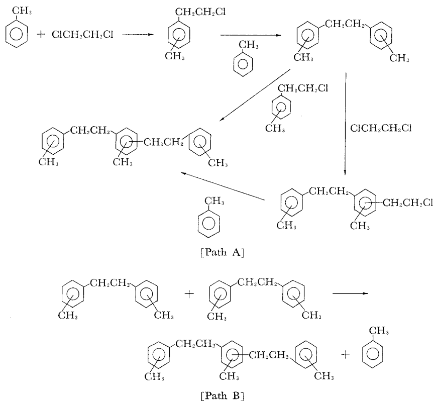
Fig. 3. Path of formation of polycondensation products.
