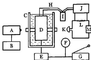
Fig. 1 Schematic diagram of apparatus.
