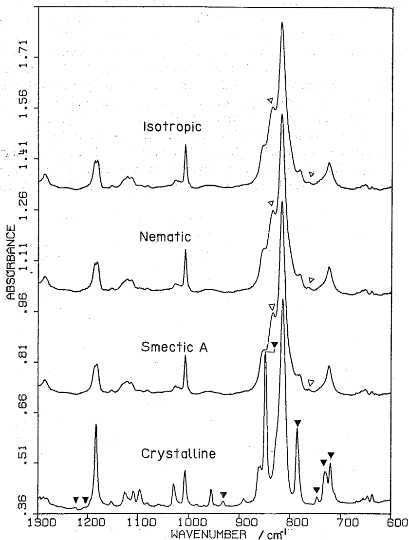
Fig. 5. The IR spectra in the range from 1300 to 600 \text{cm}^{-1} of 8CB in a KBr pellet in the crystalline, smectic A, nematic, and isotropic phases.
