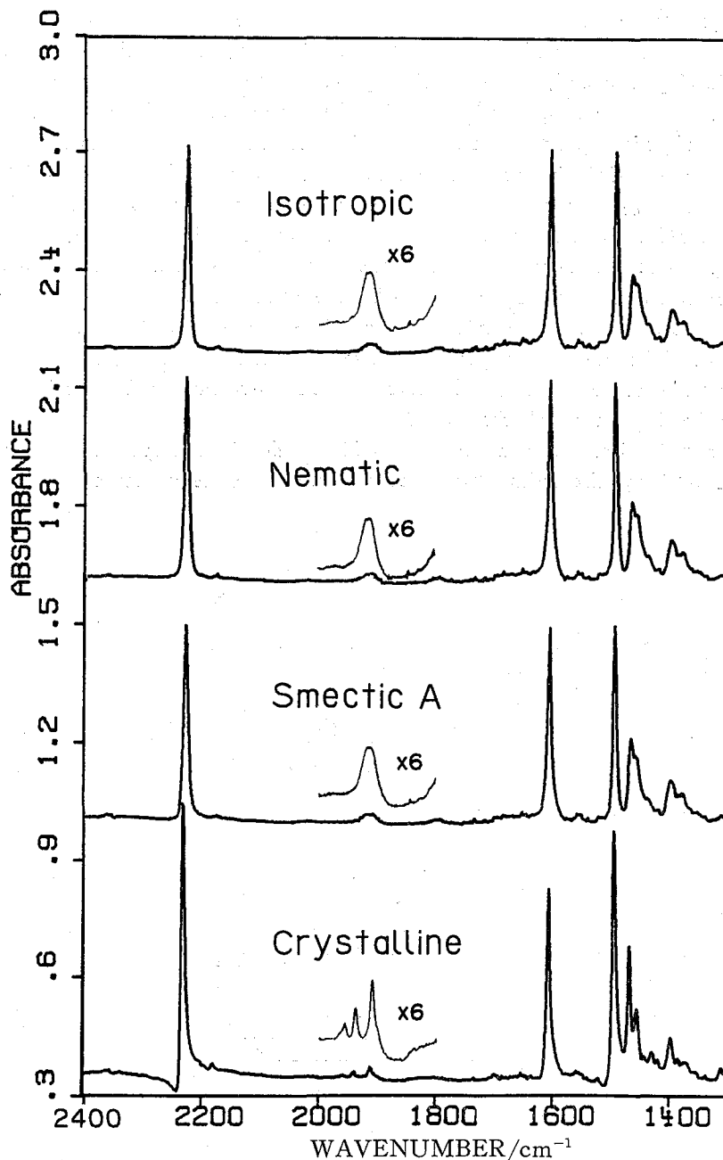
Fig. 4. The IR spectra in the range from 2400 to 1300 \text{cm}^{-1} of 8CB in a KBr pellet in the crystalline, smectic A, nematic, and isotropic phases.
