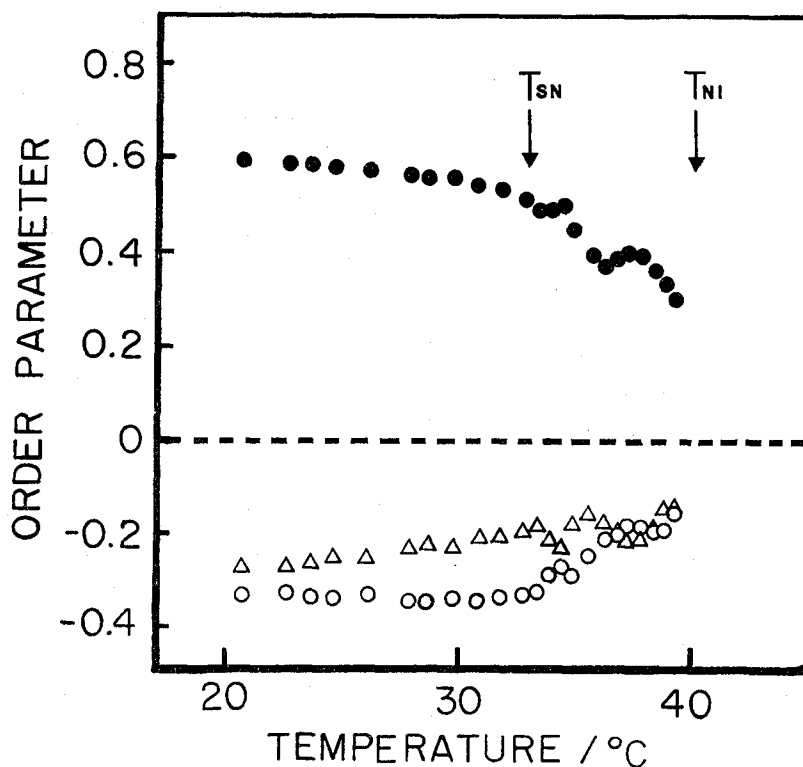
Fig. 16. Temperature dependence of the orientational order parameters with respect to the normal to the surface for the 2230 (●), 1915 (△), and 815 (○) \text{cm}^{-1} bands of Sample VIII.
