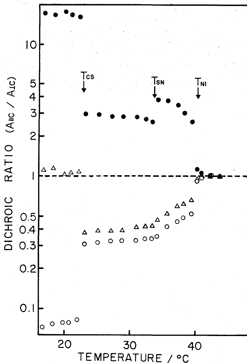
Fig. 9. Temperature dependence of the dichroic ratios for the 2230 (●), 1915 (Δ), and 815 \text{cm}^{-1} (○) bands of Sample II.
