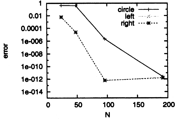
Figure 3: The error estimates of the presented method as functions of the total number of the nodes N = 3N_0 .
