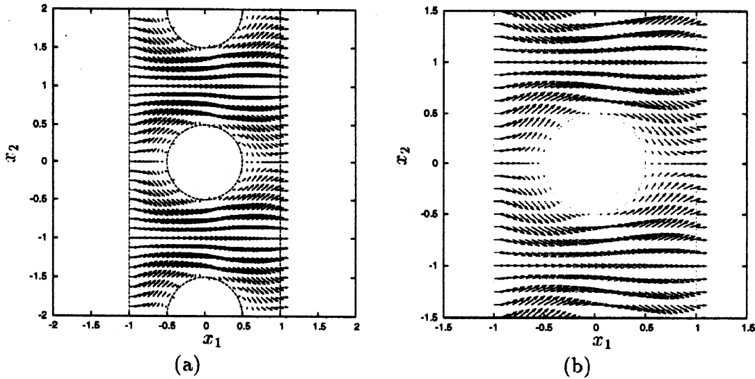
Figure 2: The velocity field of Stokes flow past a periodic array of circular cylinders computed by the presented method. The figure (b) is a magnification of the figure (a).
