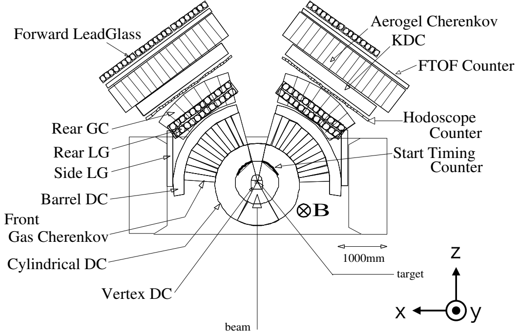
Figure 2.4: Top view of the spectrometer. Figure is adapted from Ref. [44].
