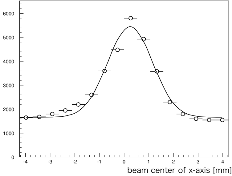
Figure 2.2: Beam-position dependence of the interaction rate in the horizontal direction. Circles represent the measured data. Solid curve shows the result of a Gaussian fit convoluted with the target width (1 mm). Figure is adapted from Ref. [44].
