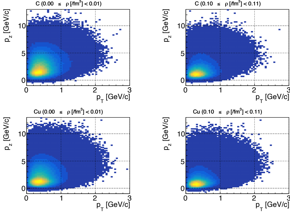
Figure 4.19: Samples of correlation between the transverse and longitudinal momenta of \phi mesons. The upper panels correspond to pC reactions, while the lower panels correspond to pCu reactions. The left panels show 0 \leq \rho < 0.01 \text{ fm}^{-3} , whereas the right panels show 0.1 \leq \rho < 0.11 \text{ fm}^{-3} .
