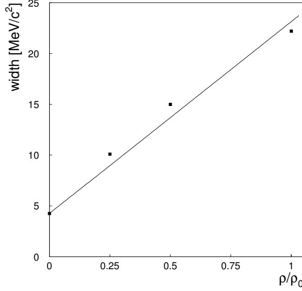
Figure 2.9: Width of the \phi meson in nuclear matter calculated in Ref. [50]. Points represent the calculated values, taken from Fig. 4 of Ref. [50]. Line shows the result of a linear fit that passes through the width at vacuum, with \Gamma_\phi(\rho)/\Gamma_\phi(0) = 1 + 4.4(\rho/\rho_0) Figure is adapted from Ref. [44].
