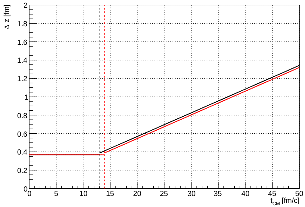
Figure 3.3: Time dependence of \Delta z for 12 GeV p^{12}\text{C} and p^{64}\text{Cu} reactions. Black (red) lines are for ^{12}\text{C} ( ^{64}\text{Cu} ). Dashed lines represent t_z . On the left-hand side of the figure, the black line overlaps with the red line.
