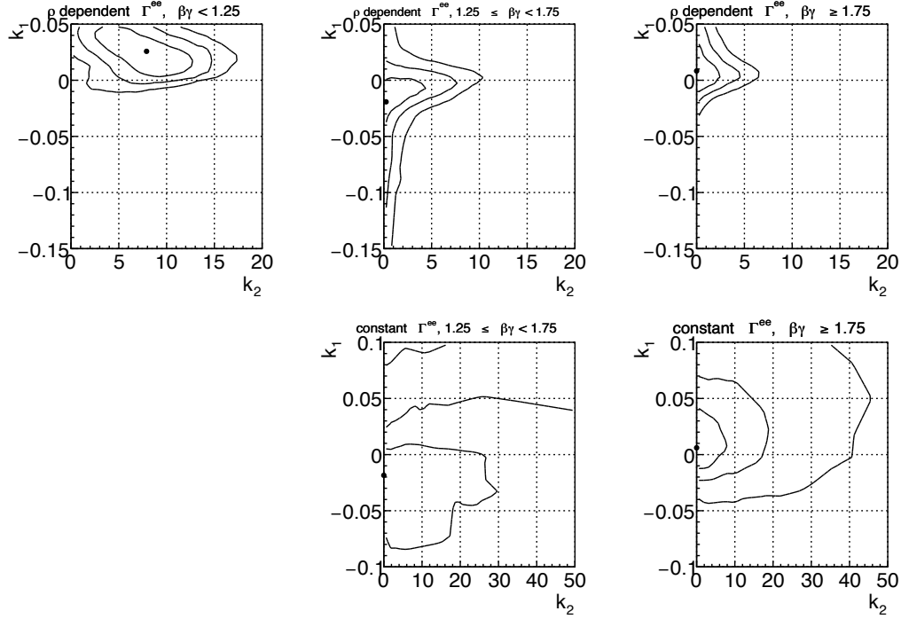
Figure 5.4: Dependence of the total \chi^2 on the shift and broadening parameters for each \beta\gamma region. Upper panels correspond to Model C-1 and lower panels to Model C-2, arranged from left to right as slow, middle, and fast regions. Black points indicate the parameters giving the minimum \chi^2 . The definitions of the contour lines, the evaluation method of the minimum \chi^2 , and the interpolation method are the same as in Figure 5.2. For the slowest \beta\gamma region in Model C-2, no minimum \chi^2 was found within the physically reasonable parameter range, so it is omitted.
