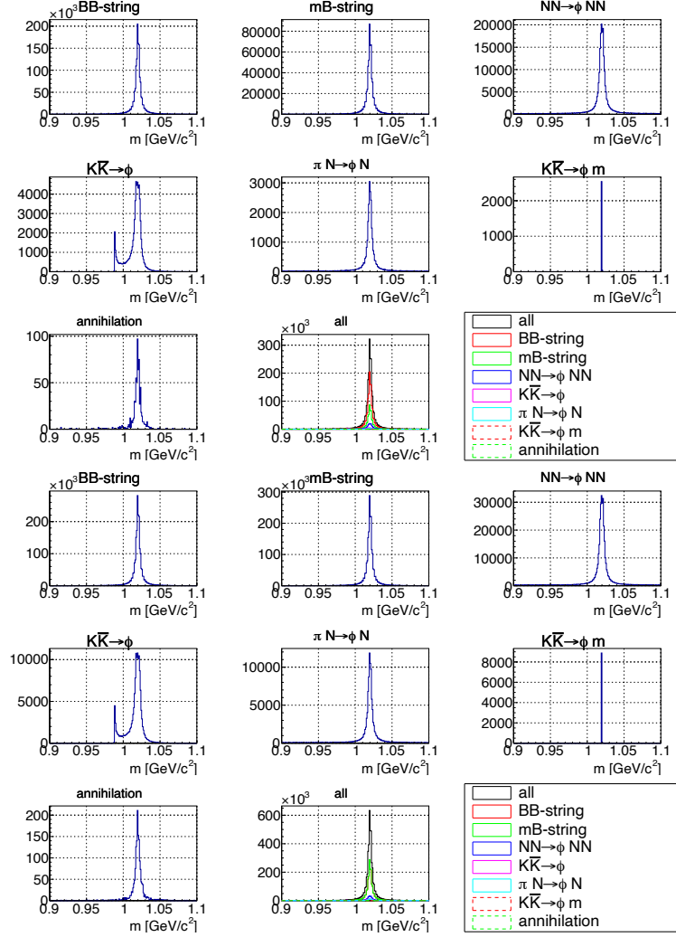
Figure 4.7: Mass spectra of \phi mesons at the time of production ( 0.9 \text{ GeV}/c^2 to 1.1 \text{ GeV}/c^2 ). The upper eight panes show the results for the pC reaction, and the lower eight panes show those for the pCu reaction. The line colors and styles correspond to the production processes as indicated in the legend.
