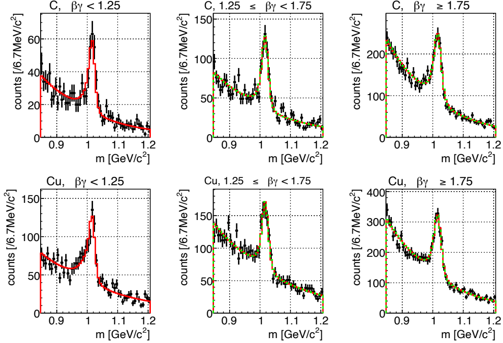
Figure 5.5: Fit results with momentum-dependent shift and broadening parameters. Black points and error bars represent the experimental data; red solid lines represent Model C-1, and green dashed lines represent Model C-2. The shift and broadening parameters used correspond to those simulated parameters closest to the best-fit ones, i.e., (k_1, k_2) = (0.03, 8), (-0.02, 0), (0.007, 0) for Model C-1 (slow, middle, and fast \beta\gamma region, respectively) and (-0.02, 0), (0.01, 0) for Model C-2 (middle and fast \beta\gamma region, respectively).
