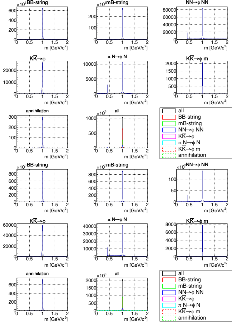
Figure 4.6: Mass spectra of \phi mesons at the time of production ( 0 \text{ GeV}/c^2 to 2 \text{ GeV}/c^2 ). The upper eight panes show the results for the pC reaction, and the lower eight panes show those for the pCu reaction. The line colors and styles correspond to the production processes as indicated in the legend.
