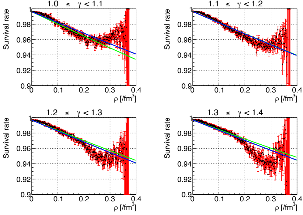
Figure 4.13: Density dependence of the survival probability of \phi mesons for several values of Lorentz factor ( \gamma ) obtained from PHSD. Black points with red error bars represent the data points. Green line shows the density dependence of the survival probability with k_2^{\text{PHSD}} = 7.18 . Blue line represents the fit results using only the data in each panel.
