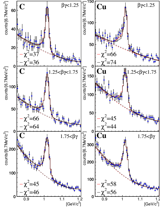
Figure 2.14: Fit results with spectral modification of Ref. [28]. Blue points represent the experimental data. Red solid and dashed curves correspond to the fit result and background component, respectively, for the density-dependent partial width (Eq. (2.4)). Black solid and dashed curves correspond to the same for the fixed partial width case. Figure is adapted from Ref. [44].
