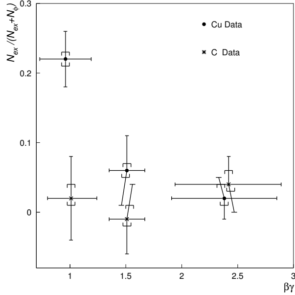
Figure 2.12: Dependence of the excess ratio on target nucleus and \beta\gamma . Vertical error bars indicate statistical uncertainties, while brackets represent systematic uncertainties. Horizontal error bars show the standard deviation of \beta\gamma for each spectrum. Figure is adapted from Ref. [44].
