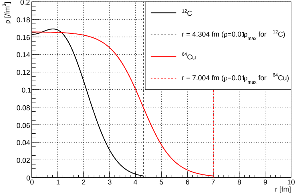
Figure 3.1: Spatial density distribution of ^{12}\text{C} and ^{64}\text{Cu} . Black (red) lines are about ^{12}\text{C} ( ^{64}\text{Cu} ). Dashed lines represent the radius at which the density is 1% of the maximum density of the nuclei.
