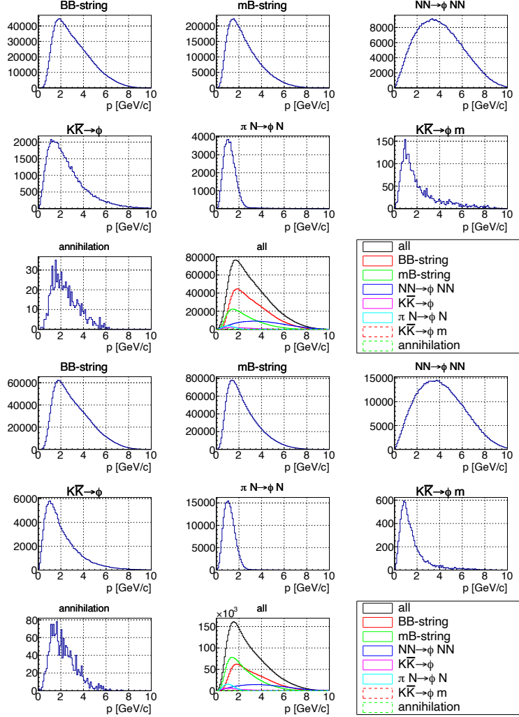
Figure 4.8: Distribution of momentum of \phi meson at production. The upper eight panes show the results for the pC reaction, and the lower eight panes show those for the pCu reaction. The line colors and styles correspond to the production processes as indicated in the legend.
