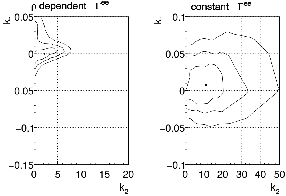
Figure 5.2: \chi^2 dependence on the shift and broadening parameters for the fit to all six spectra. Left panel shows Model B-1 and the right panel shows Model B-2. Black points indicate the parameter set yielding the minimum \chi^2 . Three contour lines correspond to differences from the minimum \chi^2 by 1\sigma ( \Delta\chi^2 = 2.30 ), 2\sigma ( \Delta\chi^2 = 6.18 ), and 3\sigma ( \Delta\chi^2 = 11.83 ), respectively. The position and value of the minimum \chi^2 were determined by fitting the points with low \chi^2 using a paraboloid. The contour map was interpolated from simulated points.
