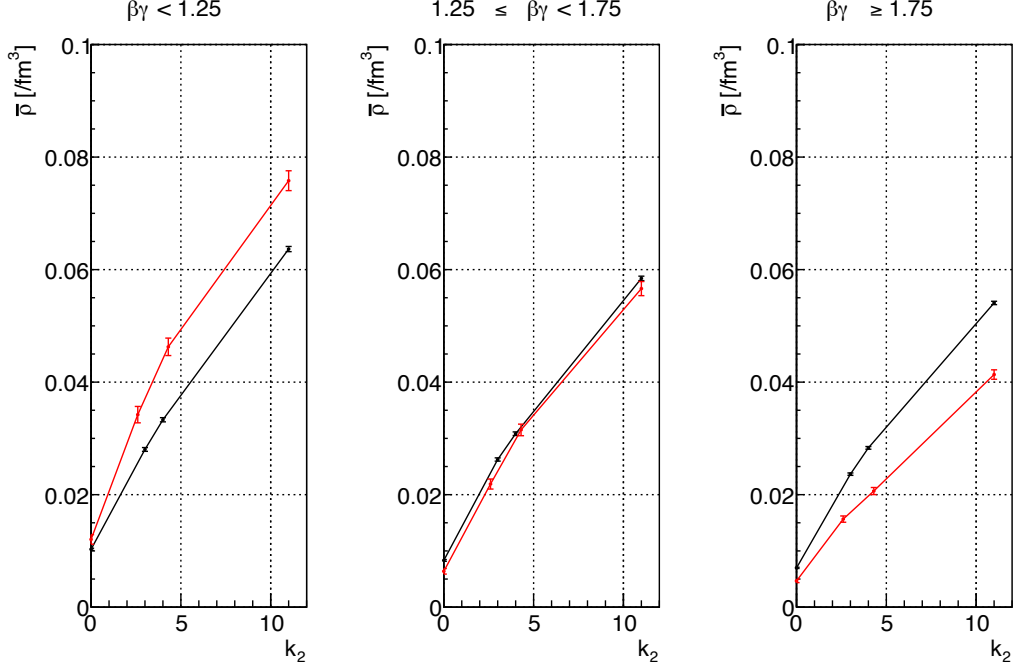
Figure 5.8: Dependence of the average decay-time density on the broadening parameter for each \beta\gamma region for pCu reaction. The values are obtained using the density-dependent partial width model. Black points and lines represent the results from the present analysis, while red points and lines are from Ref. [44]. The effects of spectrometer acceptance and detection efficiency are taken into account.
