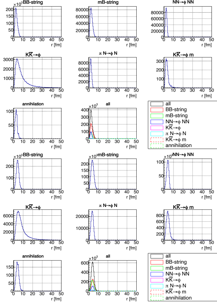
Figure 4.2: Radial distance of \phi -meson production points from the center of the target nucleus for each production channel. The upper eight panes show the results for the pC reaction, and the lower eight panes show those for the pCu reaction. The line colors and styles correspond to the production processes as indicated in the legend.
