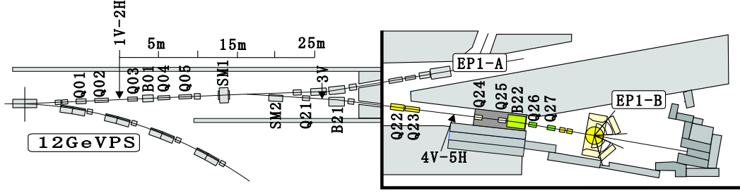
Figure 2.1: Top view of the KEK-PS EP1-B beam line. Figure is adapted from Ref. [44].
