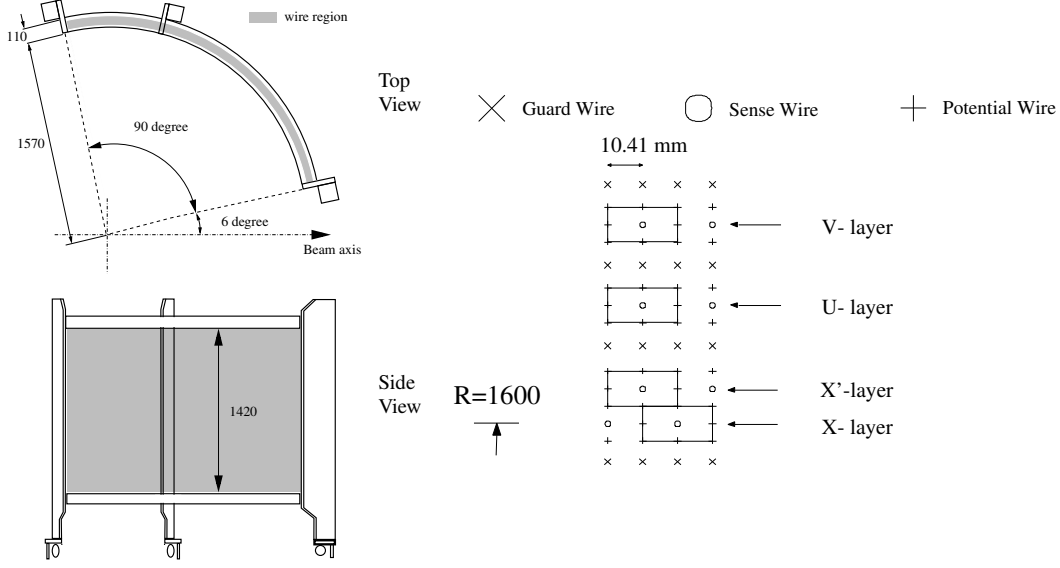
Figure 2.7: Schematic view and cell structures of BDC. Figure is adapted from Ref. [44].
