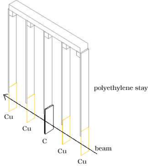
Figure 2.3: Schematic view of the targets and jigs (2002 configuration). Figure is adapted from Ref. [44].
