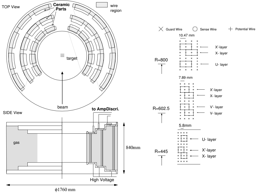
Figure 2.6: Schematic view and cell structures of CDC. Figure is adapted from Ref. [44].
