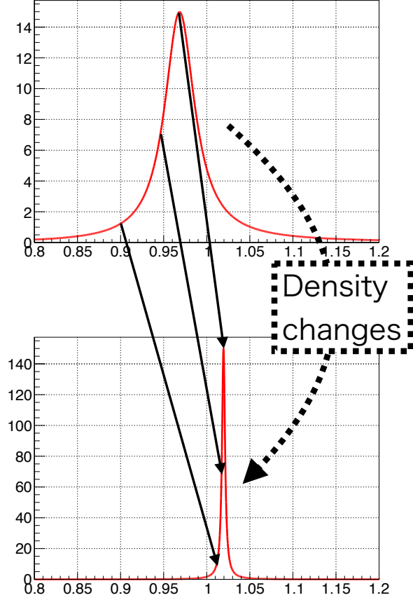
Figure 3.4: Conceptual diagram of mass updating. The upper panel shows the spectrum calculated using the density at the position before time evolution, while the lower panel shows the spectrum calculated using the density at the position after time evolution. The arrows indicate the correspondence between the mass before and after time evolution. Since the update is performed so as to conserve the cumulative probability, masses smaller than the peak remain below the peak, whereas masses larger than the peak remain above the peak after updating.
