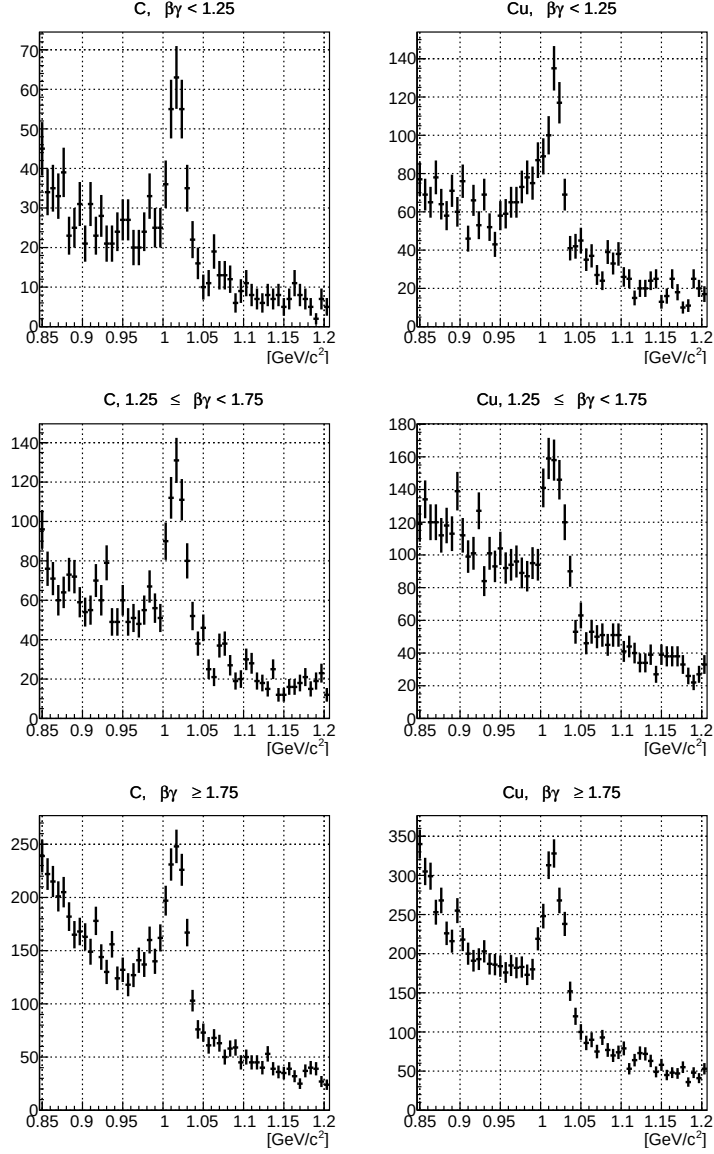
Figure 2.8: e^+e^- invariant mass spectra obtained in the experiment. The classification of spectra is described in the main text. The bin width is 1/150 \text{ GeV}/c^2 .
