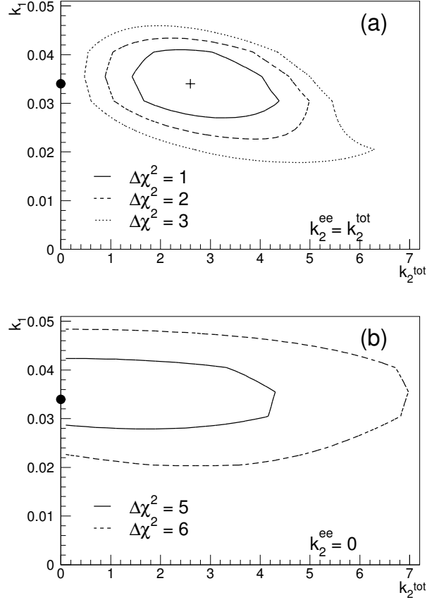
Figure 2.13: \chi^2 dependence on k_1 and k_2 for the combined fit of all six spectra (Ref. [28]). Top: assuming density-dependent partial width (Eq. (2.4)). Bottom: assuming constant partial width. The cross and black dot indicate the best-fit points in each case. Contour lines represent constant \Delta\chi^2 values from the minimum. Figure is adapted from Ref. [44].
