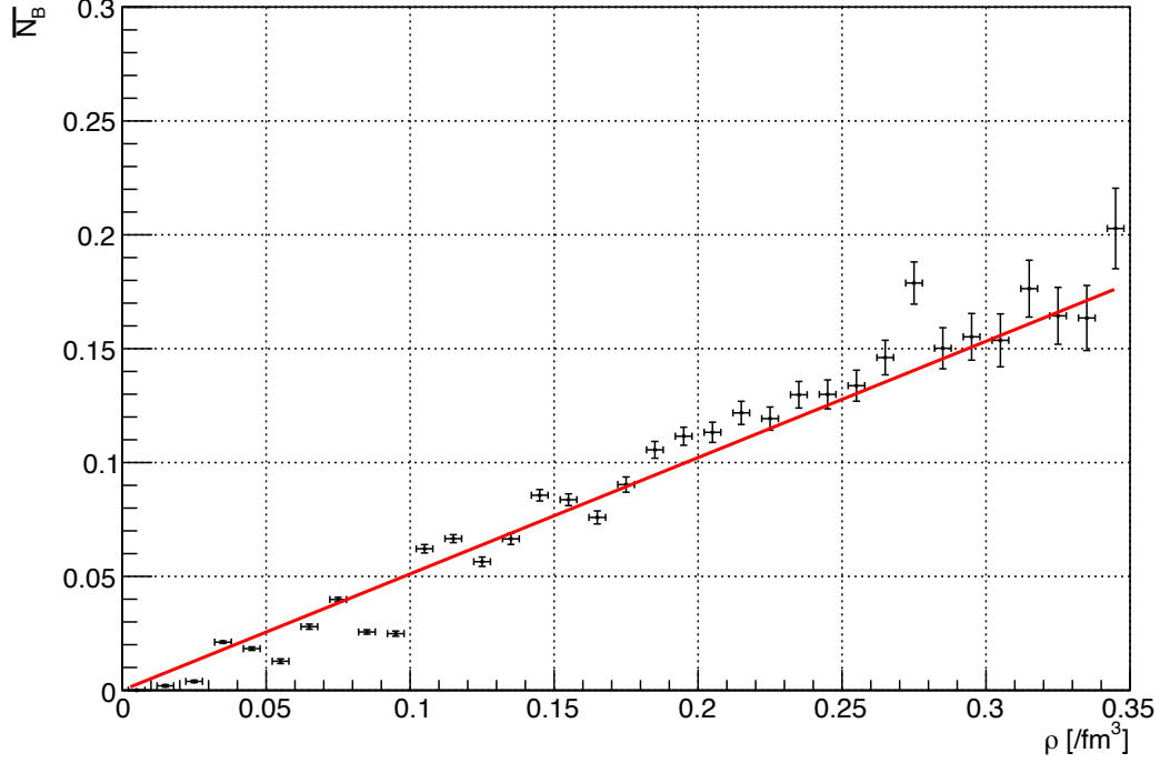
Figure 4.17: Density dependence of the number of baryons capable of undergoing \phi B reactions. The baryon number is counted only in events containing the \phi meson, not averaged over the ensemble. Black points represent the data, and red line shows the fit assuming a proportional relation.
