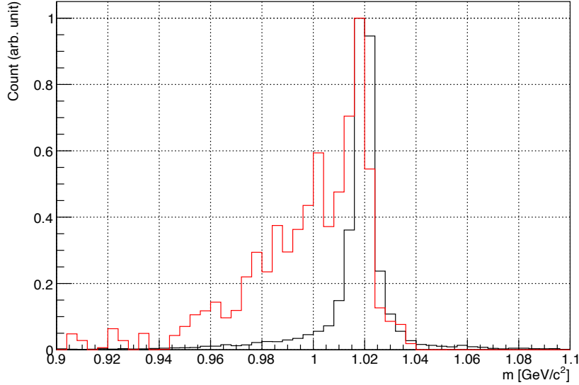
Figure 4.10: Mass distribution of \phi mesons with \beta\gamma > 2.5 . Black line represents those with CM-frame momentum above 0.2 \text{ GeV}/c , while red line corresponds to the rest. The counts are scaled so that the maximum value becomes 1, and no weighting is applied.
