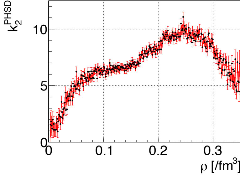
Figure 4.14: Density dependence of k_2^{\text{PHSD}} obtained from PHSD. Black points with red error bars represent the data points.
