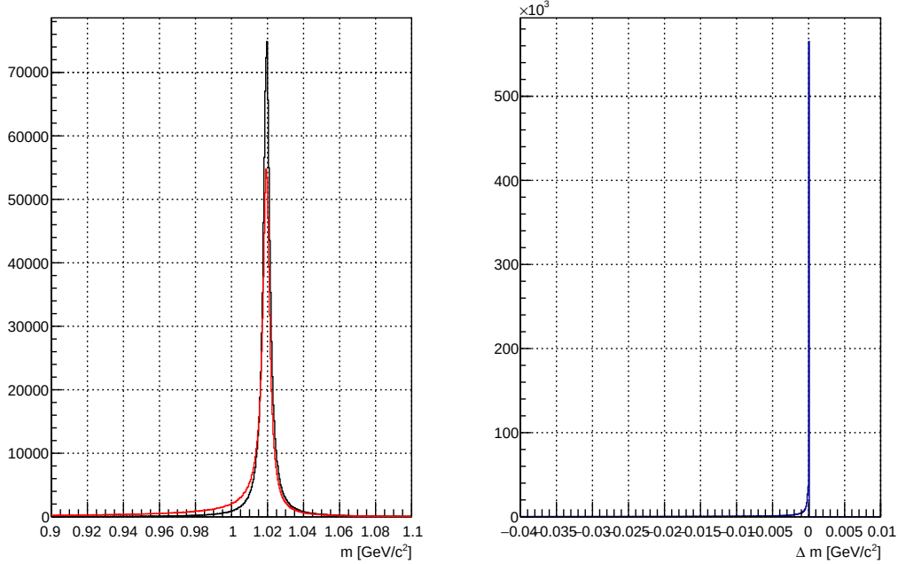
Figure 4.21: Effect of internal bremsstrahlung on the mass spectrum. In the left panel, the black line represents masses randomly sampled from a Breit–Wigner distribution using the resonance mass and width of the \phi meson [1], while the red line shows the result after applying internal bremsstrahlung. The right panel shows the mass shifts of individual \phi mesons due to internal bremsstrahlung.
