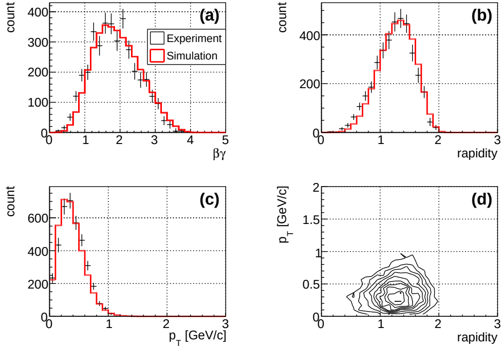
Figure 4.23: Momentum distributions obtained from the experiment and the present simulation. The panels show the \beta\gamma distribution (upper left), rapidity (upper right), transverse momentum (lower left), and the correlation between rapidity and transverse momentum (lower right). Black points represent the experimental data, while red lines represent the simulation. The simulation is fitted to the experimental data with the vertical-axis scale treated as a free parameter.
