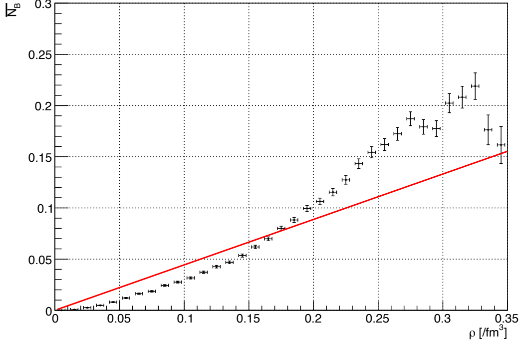
Figure 4.16: Density dependence of the number of baryons capable of undergoing \phi B reactions. The baryon number is averaged over all events in the ensemble. Black points represent the data, and red line shows the fit assuming a proportional relation.
