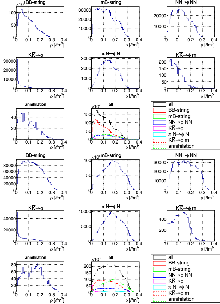
Figure 4.5: Distribution of baryon density at the \phi -meson production points. The upper eight panes show the results for the pC reaction, and the lower eight panes show those for the pCu reaction. The line colors and styles correspond to the production processes as indicated in the legend.
