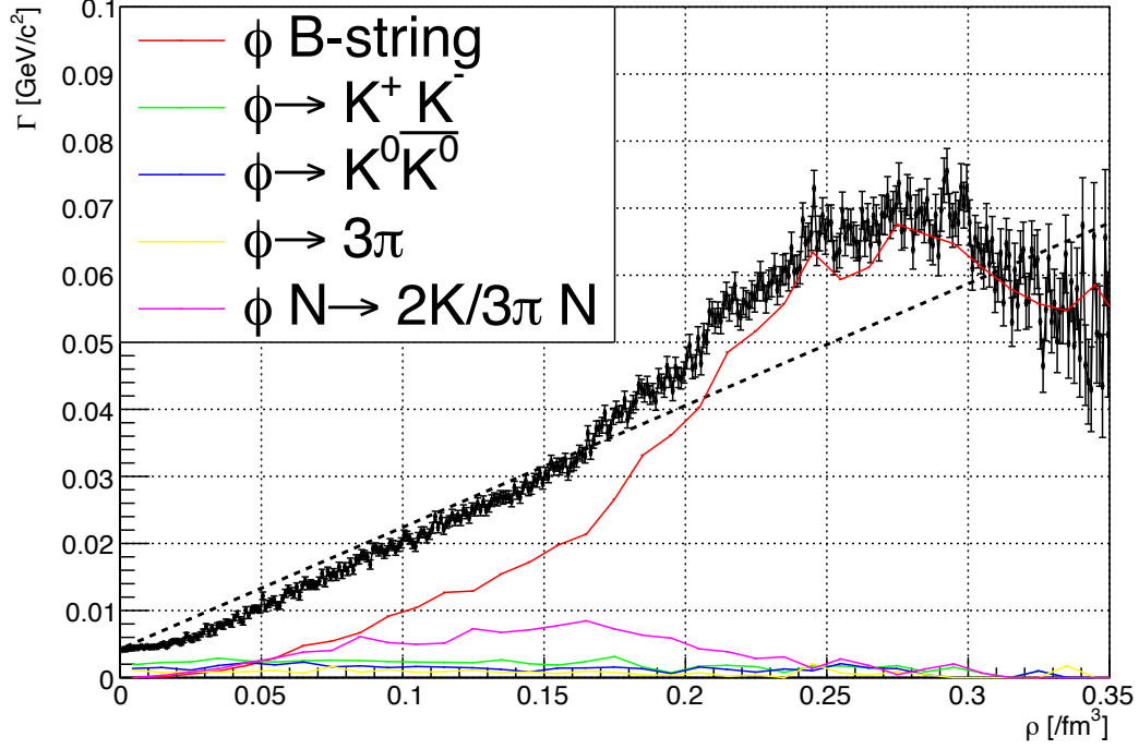
Figure 4.15: Density dependence of the \phi -meson decay width contributions from each absorption and decay channel, calculated with PHSD. Black points represent the total width. Black dashed line corresponds to the case where k_2^{\text{PHSD}} = 7.18 is substituted into Eq. (4.4). Red, green, blue, yellow, and purple lines represent \phi B -string, \phi \rightarrow K^+ K^- , \phi \rightarrow K^0 \bar{K}^0 , \phi \rightarrow 3\pi , \phi N \rightarrow 2K/3\pi N , respectively. Uncertainties are omitted for each individual absorption and decay channel, and processes with negligible contributions are omitted.
