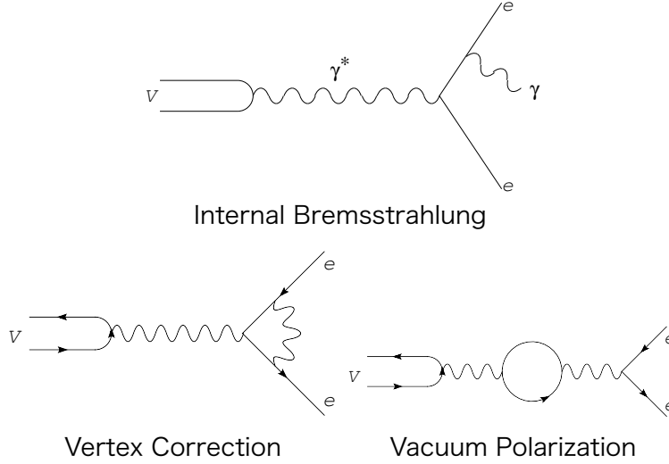
Figure 4.20: Feynman diagrams of internal bremsstrahlung, vertex correction, and vacuum polarization. Figure is adapted from Ref. [44].
