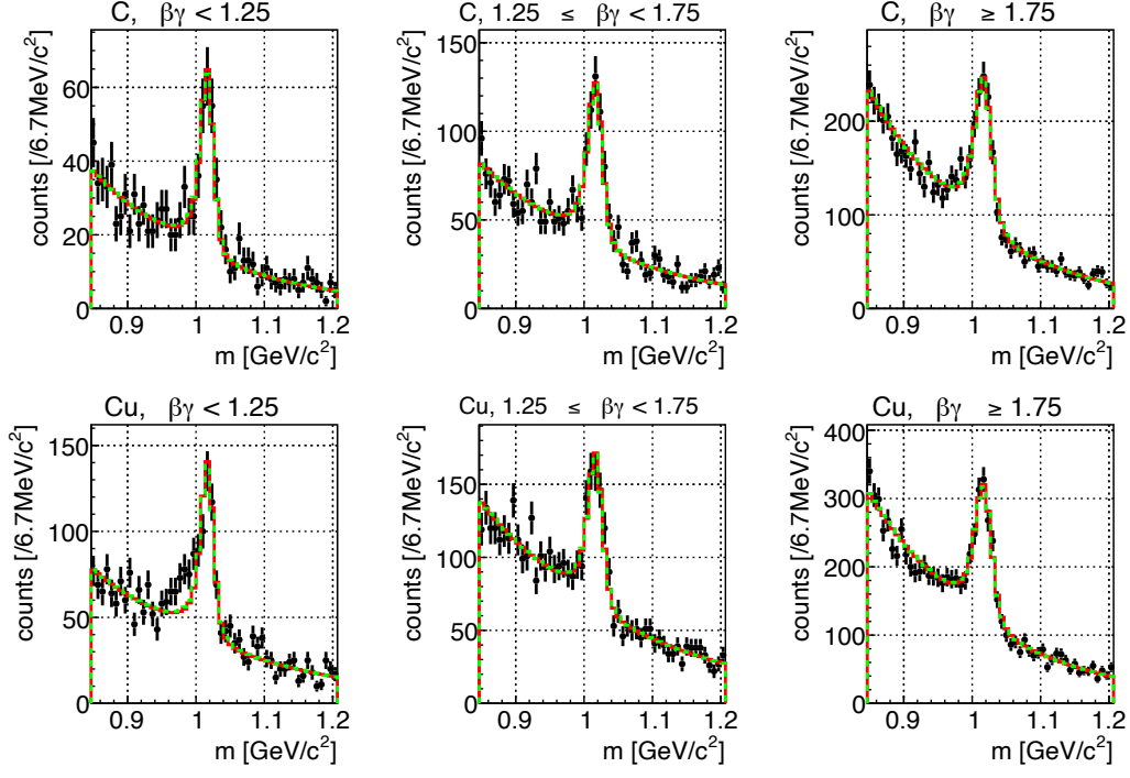
Figure 5.3: Fit results for the momentum-independent case. Black points and error bars indicate experimental data, red solid lines represent Model B-1, and green dashed lines represent Model B-2. The exact parameter values corresponding to the minimum \chi^2 were not simulated. Instead, the closest simulated parameter sets were used: (k_1, k_2) = (0, 2) for Model B-1 and (0.01, 10) for Model B-2.
