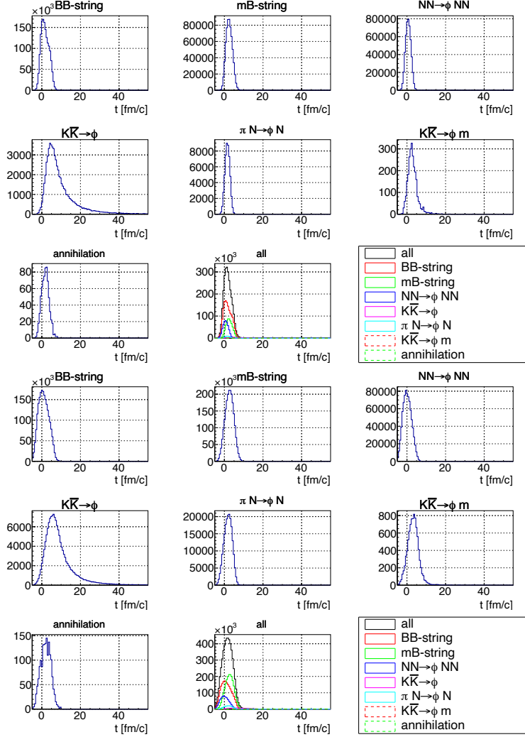
Figure 4.4: Distribution of \phi -meson production times in the laboratory frame. The upper eight panes show the results for the pC reaction, and the lower eight panes show those for the pCu reaction. The line colors and styles correspond to the production processes as indicated in the legend.
