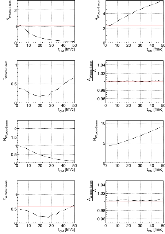
Figure 4.12: Results of fitting the nucleon distributions in the target nucleus at each time step in PHSD with the Woods–Saxon distribution (Eq. (2.5)). The upper four panes correspond to the ^{12}\text{C} target, and the lower four panes to the ^{64}\text{Cu} target. The top-left, top-right, and bottom-left panels show N , R , and \tau of Eq. (2.5), respectively, while the bottom-right panel shows the ratio of the nucleon number calculated from these parameters to the original nucleon number. For the carbon target, PHSD employs the shell model for initialization, however, since the model contains only a small number of parameters and cannot describe the time evolution well, the Woods–Saxon distribution was used for the evaluation. Red lines represent the parameters used for initialization in PHSD. Red line values of R and \tau for the carbon target were obtained by fitting the initial distribution in Fig. 3.1 with the Woods–Saxon distribution. Red line values of N for each target were determined such that the number of nucleons calculated with the obtained R and \tau agrees with that of the corresponding nucleus, using A = \int_0^\infty 4\pi r^2 \rho(r) dr \simeq (4\pi/3)N\rho_0(R^3 + \pi^2\tau^2 R) .
