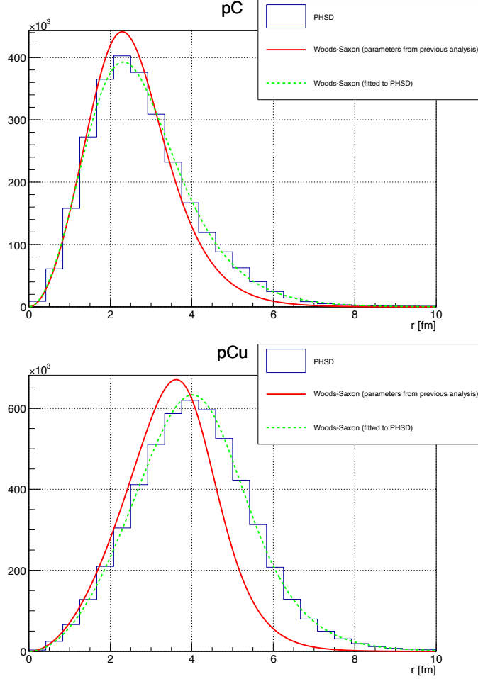
Figure 4.3: Distribution of the distance of the \phi -meson production points from the target center, together with the fit based on the Woods–Saxon distribution. Red lines represent the fitted function, with only the scale being a free parameter. Green dashed lines represent the fitted function, with the R , \tau in Eq. 2.5, and scale being free parameters. The upper panel shows the results for the pC reaction, and the lower panel shows those for the pCu reaction.
