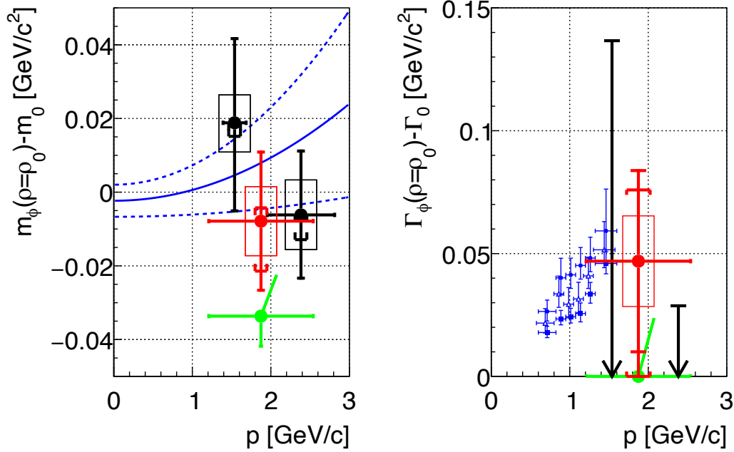
Figure 5.7: Momentum dependence of the difference in resonance mass and decay width between normal nuclear density and vacuum in Models B-2 and C-2. Definitions of the symbols are the same as in Fig. 5.6.
