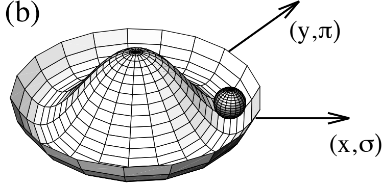
Figure 1.1: Example of the potential which cause spontaneous break of symmetry. Figure is adapted from Ref. [3].
