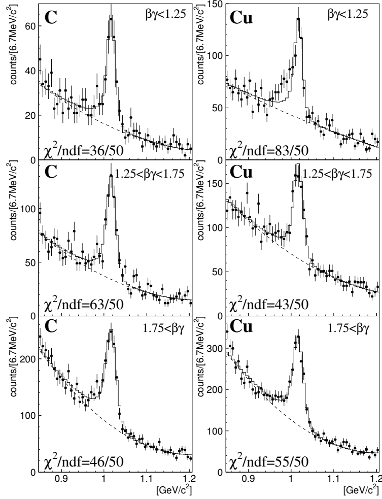
Figure 2.11: Fit result from Ref. [44] without assuming spectral modifications. Data points with error bars represent the experimental data, and the solid curve shows the fit result. Figure is adapted from Ref. [44].
