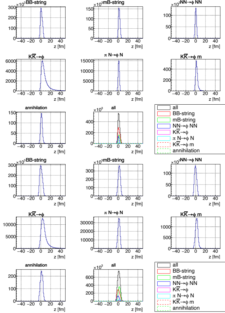
Figure 4.1: Distribution of the z -coordinates of the production points in the lab frame. The upper eight panes show the results for the pC reaction, and the lower eight panes show those for the pCu reaction. The line colors and styles correspond to the production processes as indicated in the legend.
