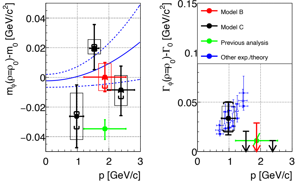
Figure 5.6: Momentum dependence of the difference in resonance mass and decay width between normal nuclear density and vacuum in Models B-1 and C-1. Left (right) panel shows the result for the resonance mass (width). Black, red, and green points correspond to Model C, Model B, and the values from Ref. [28], respectively. Vertical error bars represent statistical uncertainties (lines), systematic uncertainties due to PHSD (squares), and those due to background modeling (brackets). Horizontal error bars represent the RMS of the momentum distributions in each \beta\gamma region. Blue solid line in the left panel is the theoretical prediction from the QCD sum rule and lattice QCD, and the dashed line represents its uncertainty band. Blue points in the right panel are the results of COSY-ANKE experiment extracted from Fig. 4(a) of Ref. [30], using different theoretical models (indicated by different markers) as described in Ref. [68–70]. To improve visual clarity, certain error bars are displayed at an angle.
