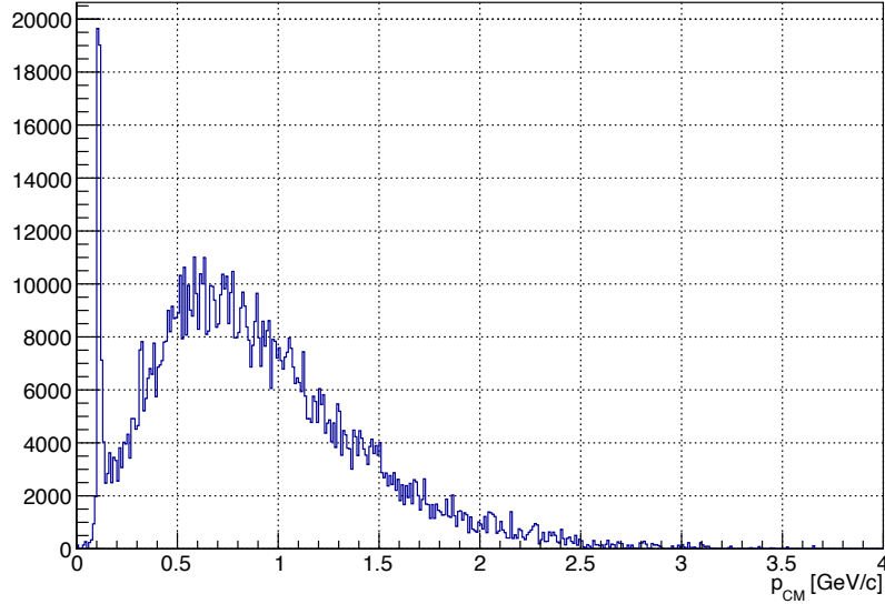
Figure 4.9: CM-frame momentum distribution of \phi mesons obtained from PHSD. The momentum over all time steps is filled, without any weighting applied.
