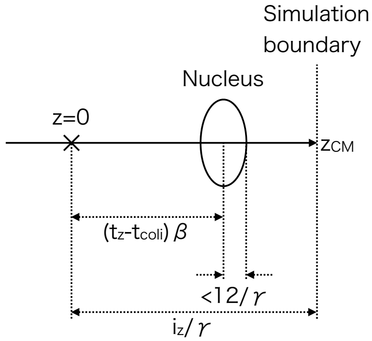
Figure 3.2: Schematic illustration of the concept represented by Eq. (3.4).
