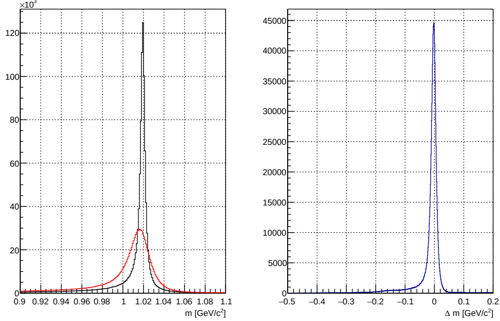
Figure 4.22: Impact of experimental effects on the mass spectrum. Black line in the left panel represents the spectrum of \phi mesons with IRC, generated using the method described up to Sect. 4.3.2. Red line is obtained from the decay of the black-line \phi mesons into e^+e^- pairs, with additional effects of energy loss, hit-position smearing, and tracking applied. \phi mesons that were not detected due to tracking inefficiencies have been excluded from the black line. Neither the black nor the red line includes the effects of cut conditions or efficiency. Furthermore, the corrections discussed in Sect. 4.3.4 and Sect. 4.3.5 have not been applied. The right panel shows the difference in mass before and after the application of experimental effects for each \phi meson.
