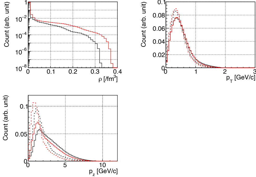
Figure 4.18: Density distribution at the \phi meson position (upper left), transverse momentum distribution (upper right), and longitudinal momentum distribution (lower left). The distributions are normalized to unity. Black lines correspond to pC reactions, and red lines to pCu reactions. Solid lines indicate 0 \leq \rho < 0.01 \text{ fm}^{-3} , while dashed lines indicate 0.1 \leq \rho < 0.11 \text{ fm}^{-3} .
