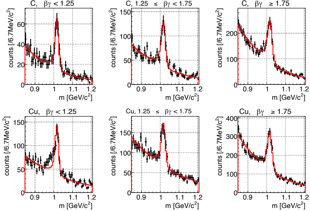
Figure 5.1: Invariant mass distributions of e^+e^- pairs classified by target nucleus and the \beta\gamma of the parent particle, along with the fit results assuming no spectral modification of the \phi meson. Black points with error bars represent the experimental data. Red lines indicate the fit functions.
