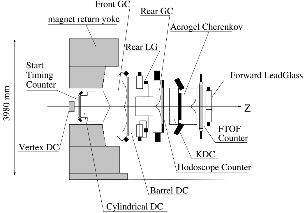
Figure 2.5: Side view of the spectrometer. Figure is adapted from Ref. [44].
