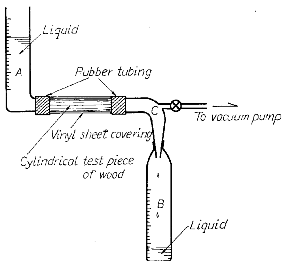
Fig. 1. Experimental apparatus.
