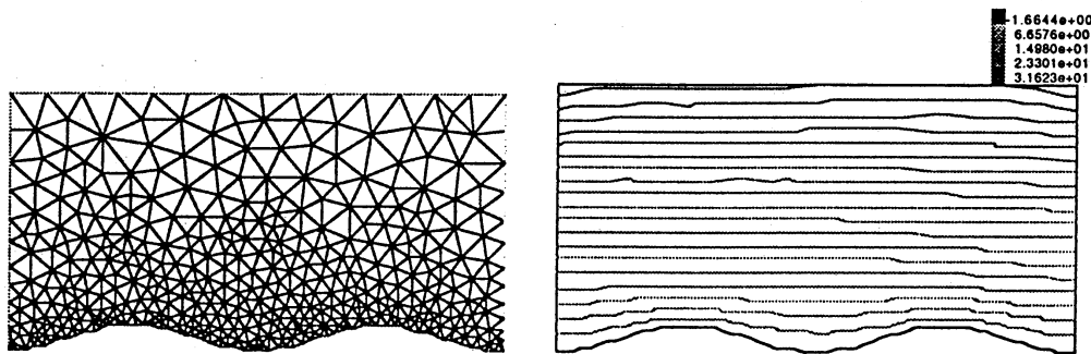
Figure 2 : The cell problem 2D Navier-Stokes eqs at Re = \nu^{-1} = 50 (Gfem(1995)).
