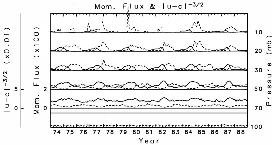
Fig. 4. Time series of the two terms, momentum flux (solid line) and |u-c|^{-3/2} (dashed line) calculated from the observed monthly-mean zonal wind for the six levels, 100, 70, 50, 30, 20, and 10 mb.
