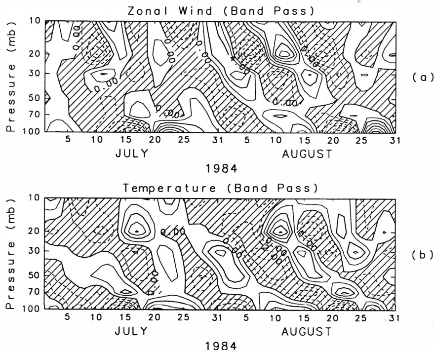
Fig. 1. Time-height sections of the band-pass filtered fields for (a) the zonal wind (contour interval 2 \text{ ms}^{-1} ) and (b) the temperature (contour interval 1 K) during the period of July to August 1984. Negative values are hatched.
