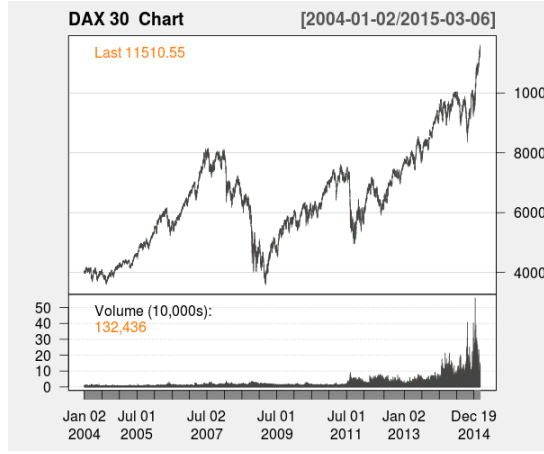
Fig. 1 DAX 30 index-level chart
