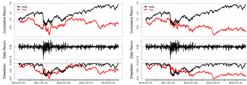
(e) Bagging SVM, 1600 window length, 160 OOS, DAX 30 daily data (f) Standard SVM, 1600 window length, 160 OOS, DAX 30 daily data
