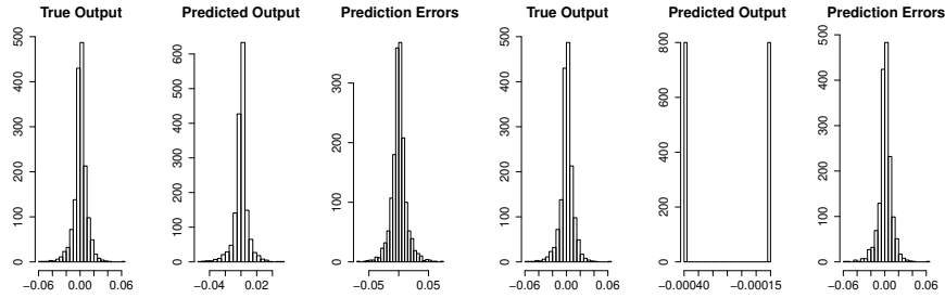
(c) Negative Example: SVM before KPCA (RMSE = 0.0128) (d) Negative Example: SVM with KPCA (RMSE = 0.0095)
