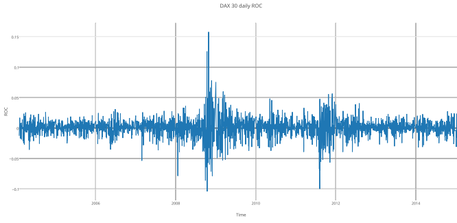
Fig. 3 The rate of changes (ROC) of the DAX 30 daily data, of which we aim at predicting the time series
