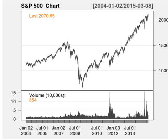
Fig. 2 S&amp;P 500 index-level chart
