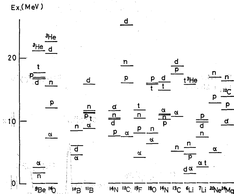
Fig. 1. Particle-decay threshold energies of some light nuclei.
