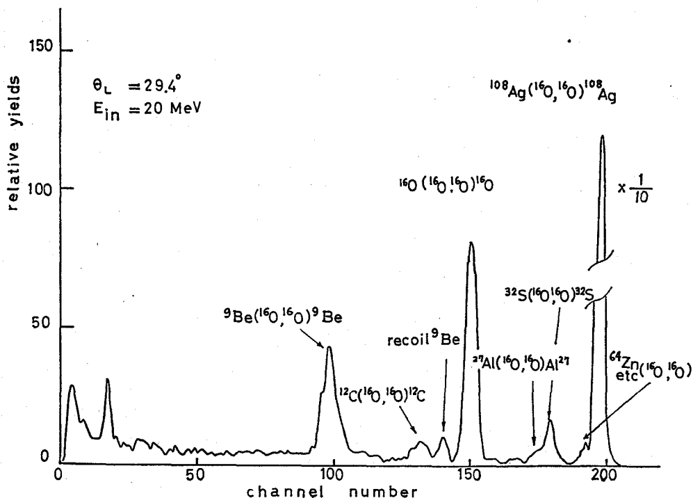
Fig. 2. An example of the energy spectrum of ^{16}\text{O} scattering on ^9\text{Be} .
