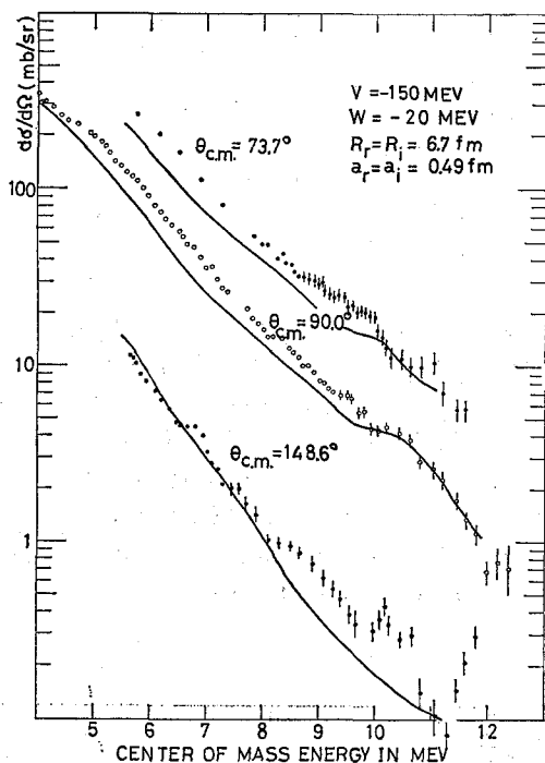
Fig. 5. Excitation functions of {}^9\text{Be} + {}^{16}\text{O} elastic scattering at 73.7^\circ , 90.0^\circ and 148.6^\circ in C.M. system. Comparison between the experimental values and the optical model calculation using the deeper potential.
