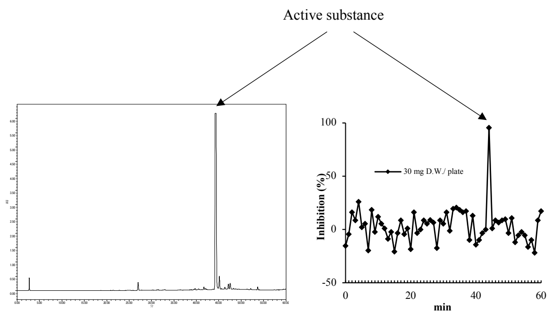
Figure 17 HPLC chromatogram of crude extract from G. andersonii bark
