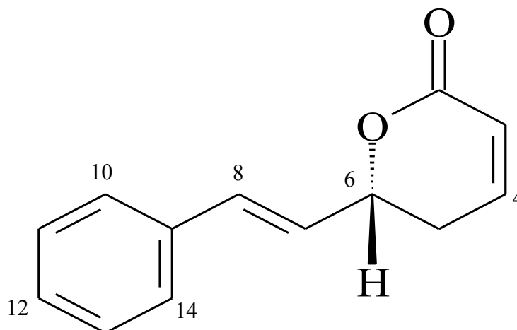
Figure 19 Chemical structure of the active substance, ( R )-(+)-goniothalamine
