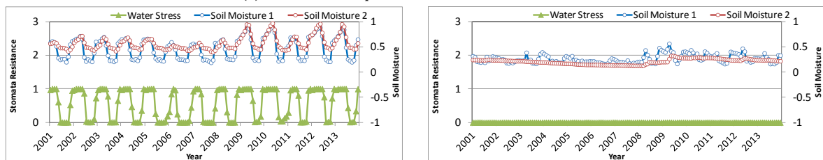
(f) Soil moisture and stomata water stress
