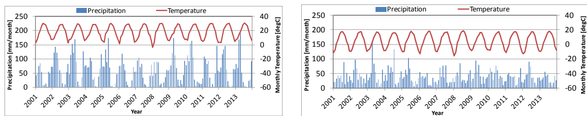
(a) Averaged monthly precipitation and monthly averaged temperature
