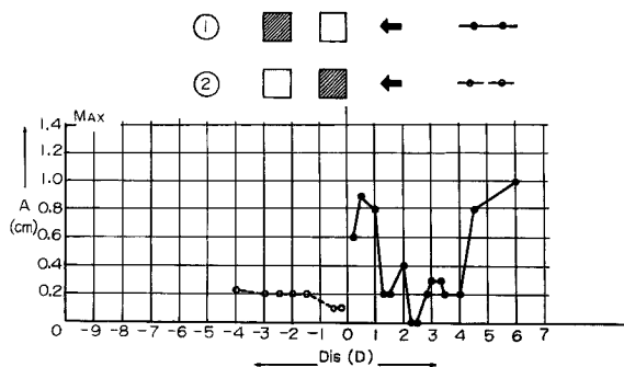
Fig. 3 Displacement of an oscillating cylinder versus the distance between cylinders.
