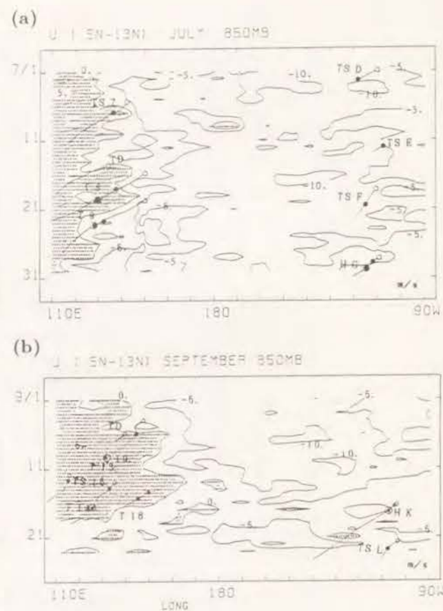
Fig. 13. As in Fig. 12 except at the 850 mb level.
