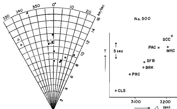
Fig. 4. Computed results and time-distance graph for earthquake No. 500.
