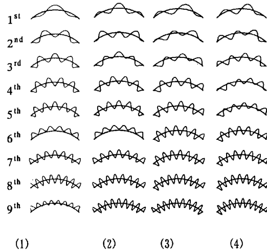
Fig.4 Examples of eigen mode Ly/Lx=0.5 , a/h=500 , \phi_0=90^\circ
