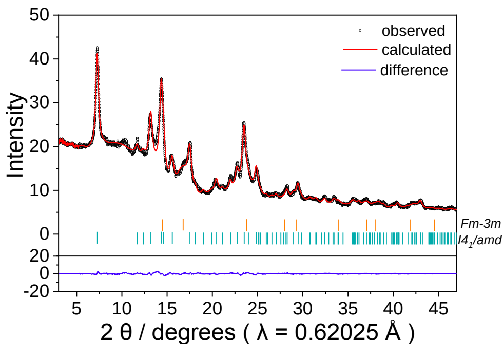
Figure 5-8. XRD pattern and Rietveld analytical fitting profile of the \text{Mg}_{1.24}\text{Mn}_2\text{O}_4 cathode sample.
