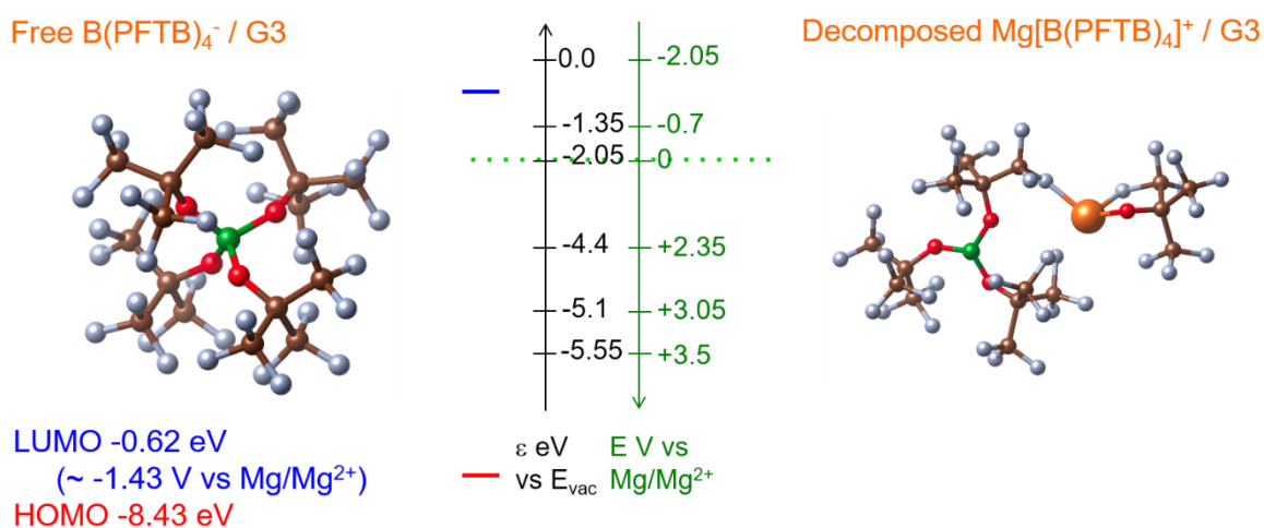
Figure 4-8. DFT cluster calculations of free [B(\text{PFTB})_4]^- and in contact [B(\text{PFTB})_4]^- .
