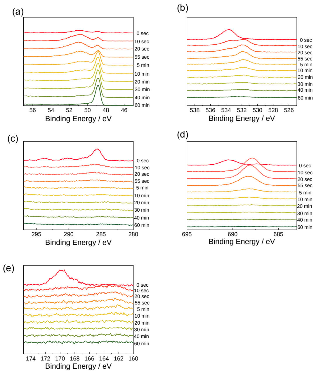
Figure 2-14. XPS spectra for the Mg metal immersed in the 0.5 M Mg(TFSA) 2 /triglyme; (a) Mg 2p, (b) O 1s, (c) C 1s, (d) F 1s and (e) S 2p. The Ar ion beam sputtering times are marked at the right side of the graph.
