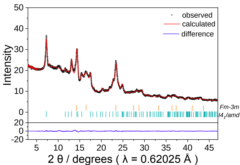
Figure 5-10. XRD pattern and Rietveld analytical fitting profile of the \text{Mg}_{1.44}\text{Mn}_2\text{O}_4 cathode sample.
