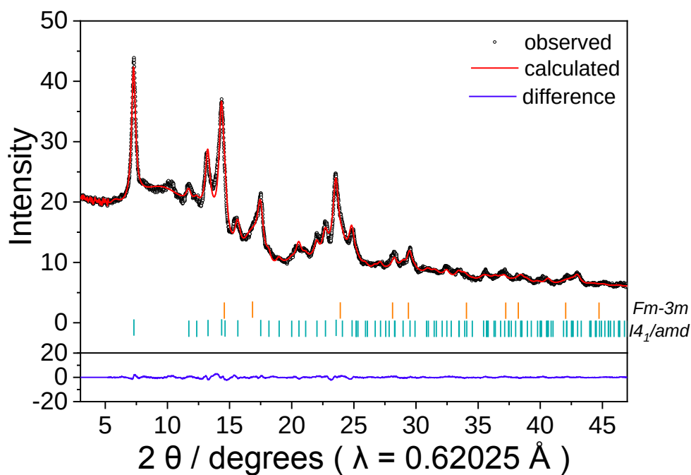
Figure 5-7. XRD pattern and Rietveld analytical fitting profile of the \text{Mg}_{1.14}\text{Mn}_2\text{O}_4 cathode sample.
