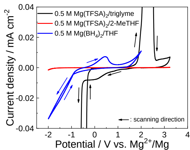
Figure 2-1. (a) Cyclic voltammograms of the 0.5 M \text{Mg}(\text{TFSA})_2/\text{triglyme} , 0.5 M \text{Mg}(\text{TFSA})_2/2\text{-MeTHF} , and 0.5 M \text{Mg}(\text{BH}_4)_2/\text{THF} at a sweeping rate of 5 mV/s. (b) Enlarged figure of (a) between -2.5 and 2.5 V (vs. \text{Mg}^{2+}/\text{Mg} )
