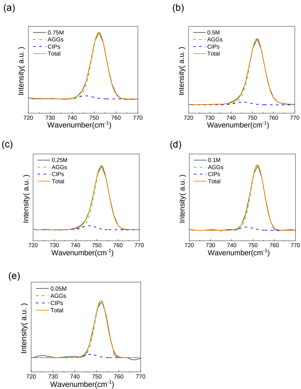
Figure 2-8. Raman spectra and Voigt function fitting results of \text{Mg}(\text{TFSA})_2/2\text{-MeTHF} in several concentrations (a) 0.75 M (b) 0.5 M (c) 0.25 M (d) 0.1 M and (e) 0.05 M in the wave number between 720 and 770 \text{cm}^{-1} .
