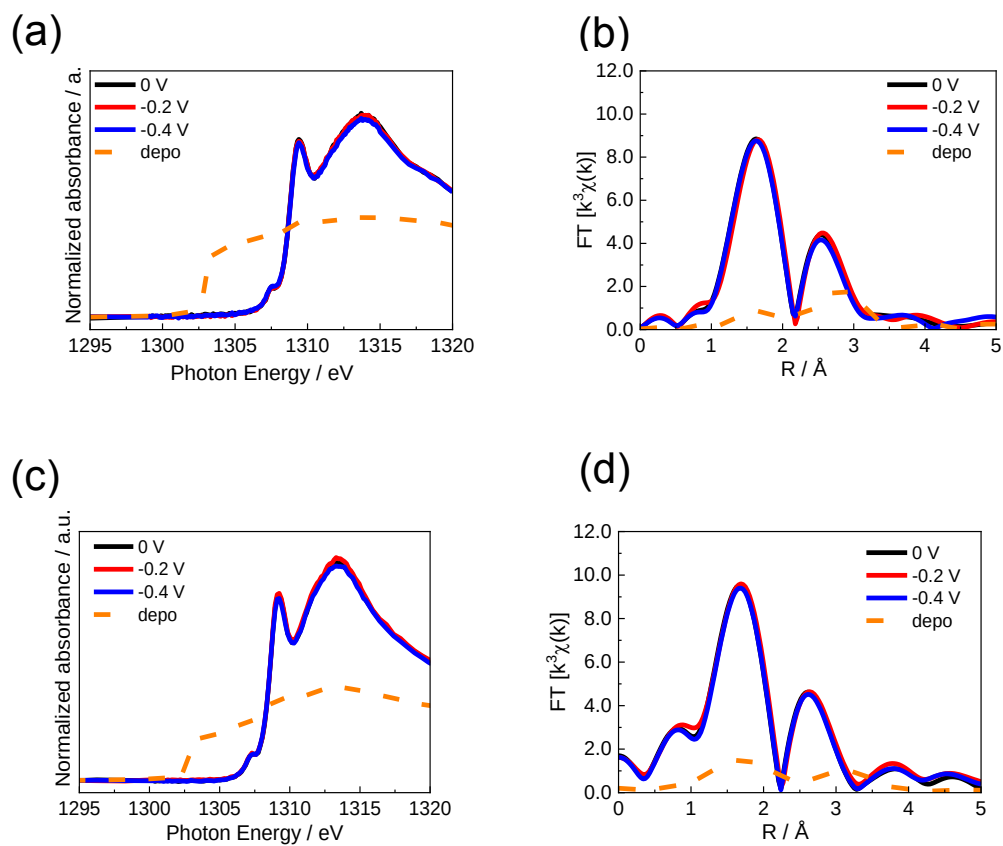
Figure 3-12. Mg K -edge (a) XANES spectra (b) Fourier-transformed EXAFS spectra obtained from operando XAS measurements 0.3 M Mg[B(HFIP) 4 ] 2 /triglyme and (c) XANES spectra (d) Fourier-transformed EXAFS spectra obtained from operando XAS measurements 0.3 M Mg[B(HFIP) 4 ] 2 /2-MeTHF.
