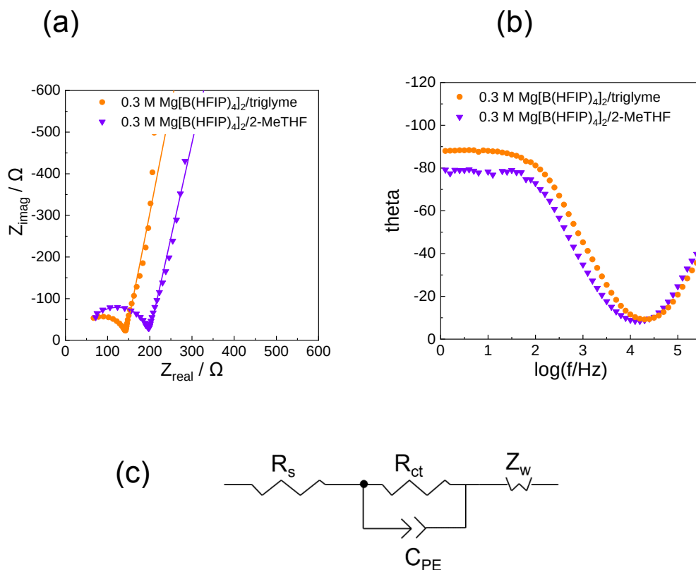
Figure 3-16. (a) Nyquist plots of Mg electrode immersed in 0.3 M \text{Mg}[\text{B}(\text{HFIP})_4]_2/\text{triglyme} , and 0.3 M \text{Mg}[\text{B}(\text{HFIP})_4]_2/2\text{-MeTHF} electrolytes. Fitted impedance spectra shown in solid line. (b) Bode phase shift plot that donates the capacitive responses. (c) Equivalent circuit model, in which electrolyte solution resistance is R_s , charge transfer resistance is R_{ct} , constant phase element is C_{PE} and the Warburg impedance is Z_w .
