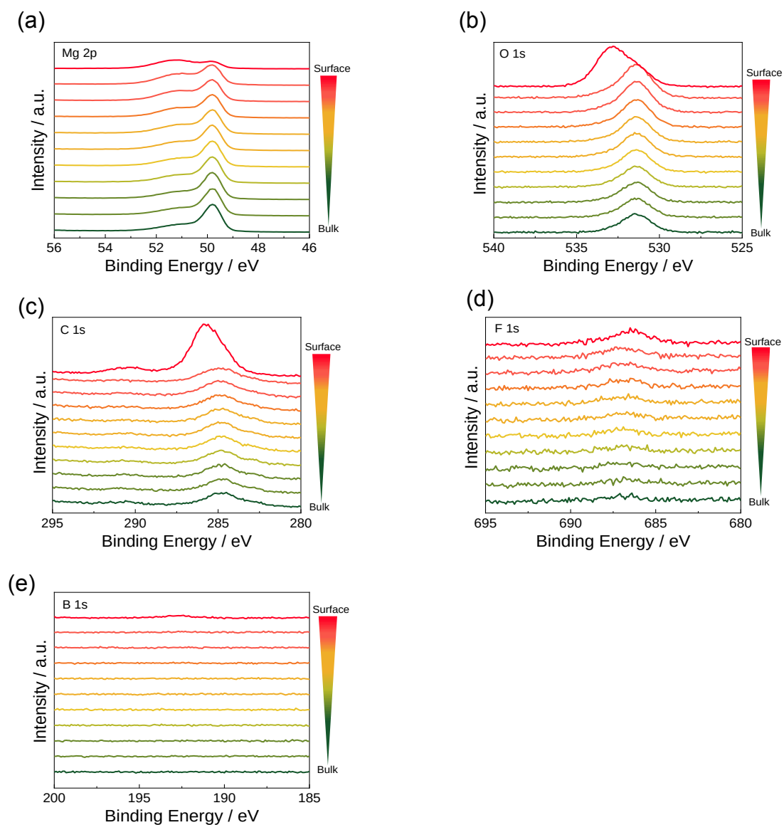
Figure 3-15. XPS spectra for the Mg metal immersed in the 0.3 M \text{Mg}[\text{B}(\text{HFIP})_4]_2/2\text{-MeTHF} ; (a) Mg 2p, (b) O 1s, (c) C 1s, (d) F 1s and (e) B 1s. The Ar ion beam sputtering times are marked at the right side of the graph.
