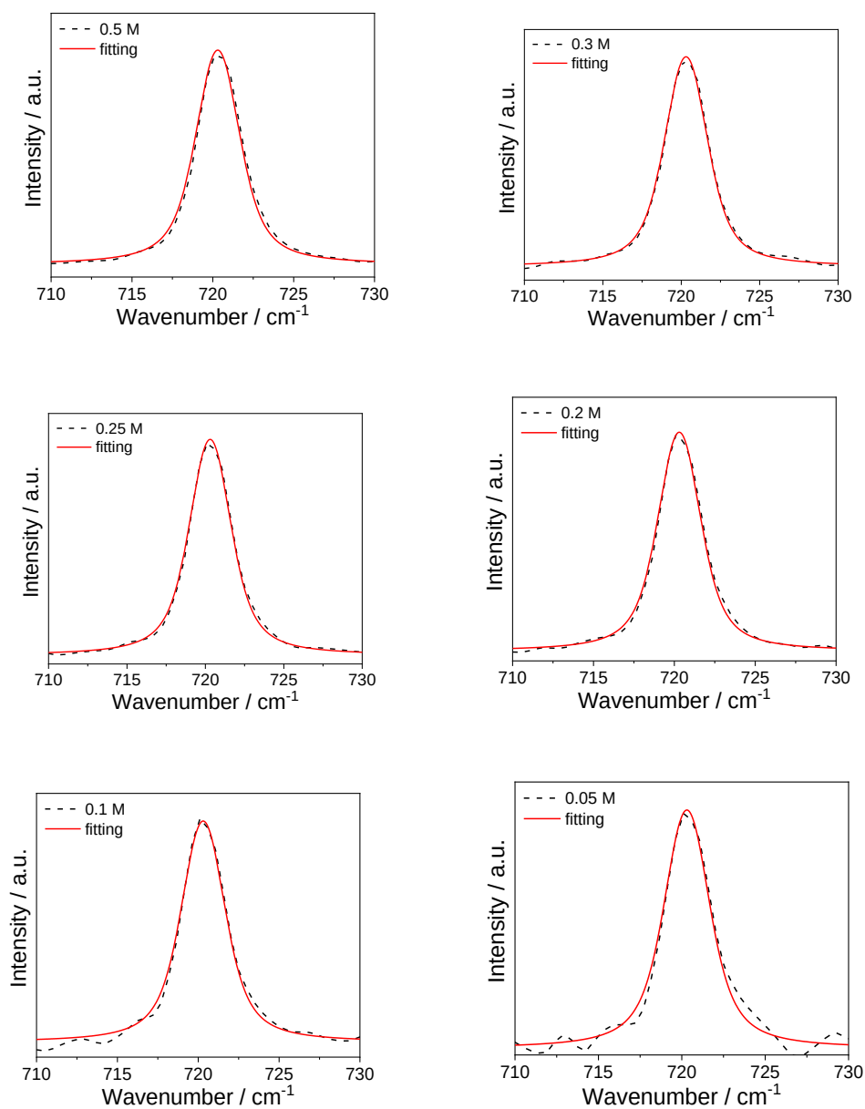
Figure 3-7. Raman spectra and voigt function fitting results of \text{Mg}[\text{B}(\text{HFIP})_4]_2/\text{triglyme} in several concentrations in the wave number between 710 and 730 \text{cm}^{-1} .
