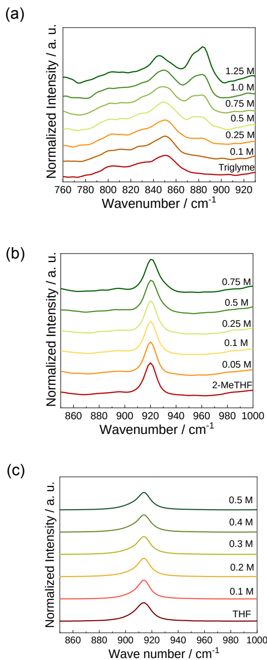
Figure 2-9. Raman spectra of (a) \text{Mg}(\text{TFSA})_2/\text{triglyme} with several concentrations in the wave number between 760 and 930 \text{cm}^{-1} (b) \text{Mg}(\text{TFSA})_2/2\text{-MeTHF} and (c) \text{Mg}(\text{BH}_4)_2/\text{THF} in the wave number between 850 and 1000 \text{cm}^{-1} .
