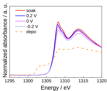
Figure 2-11. Mg K -edge XANES spectra obtained from the operando XAS measurements for the (a) 0.5 M Mg(TFSA) 2 /triglyme, (b) 0.5 M Mg(TFSA) 2 /2-MeTHF, and (c) 0.5 M Mg(BH 4 ) 2 /THF electrolytes. The potential is expressed as vs. Mg 2+ /Mg.
