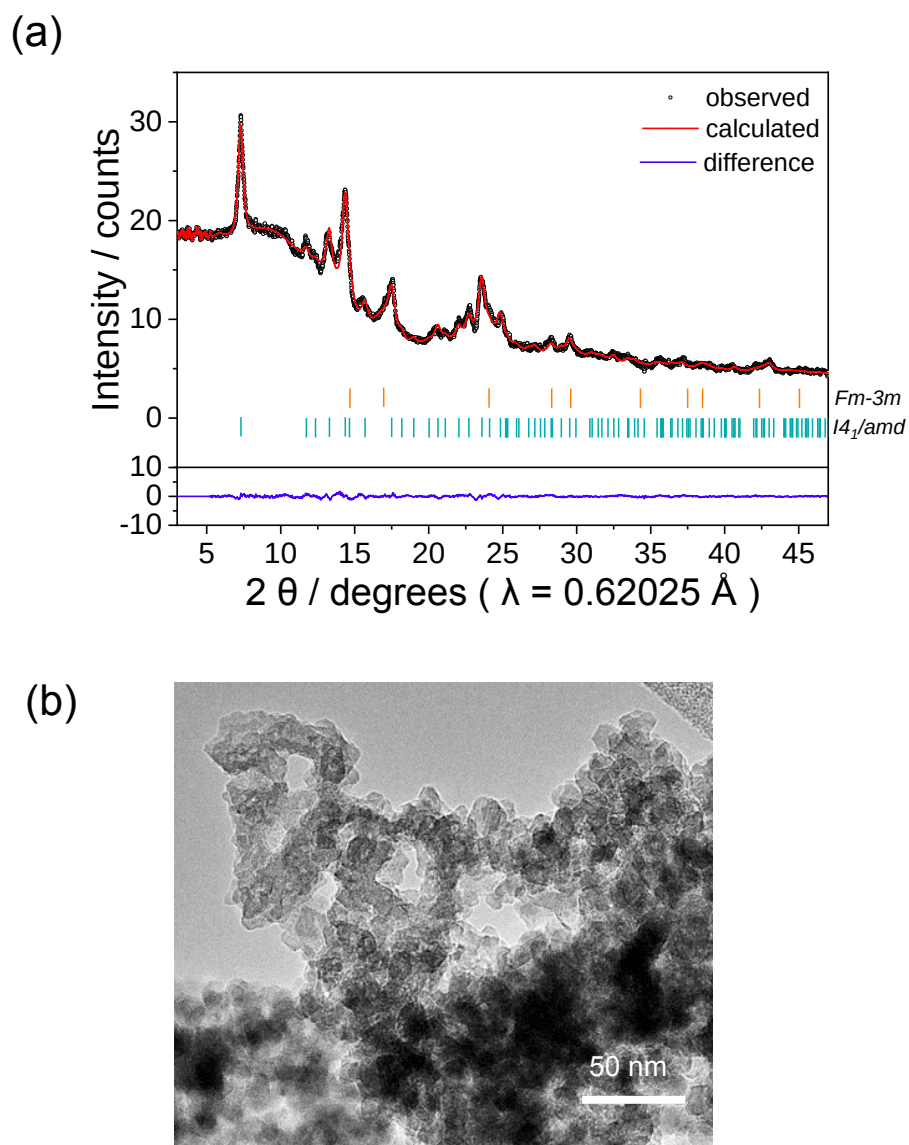
Figure 5-2. Characterization of \text{MgMn}_2\text{O}_4 cathode: (a) XRD pattern and Rietveld analytical fitting profile of the \text{Mg}_{1.04}\text{Mn}_2\text{O}_4 cathode sample and (b) TEM image of the \text{Mg}_{1.04}\text{Mn}_2\text{O}_4 powder.
