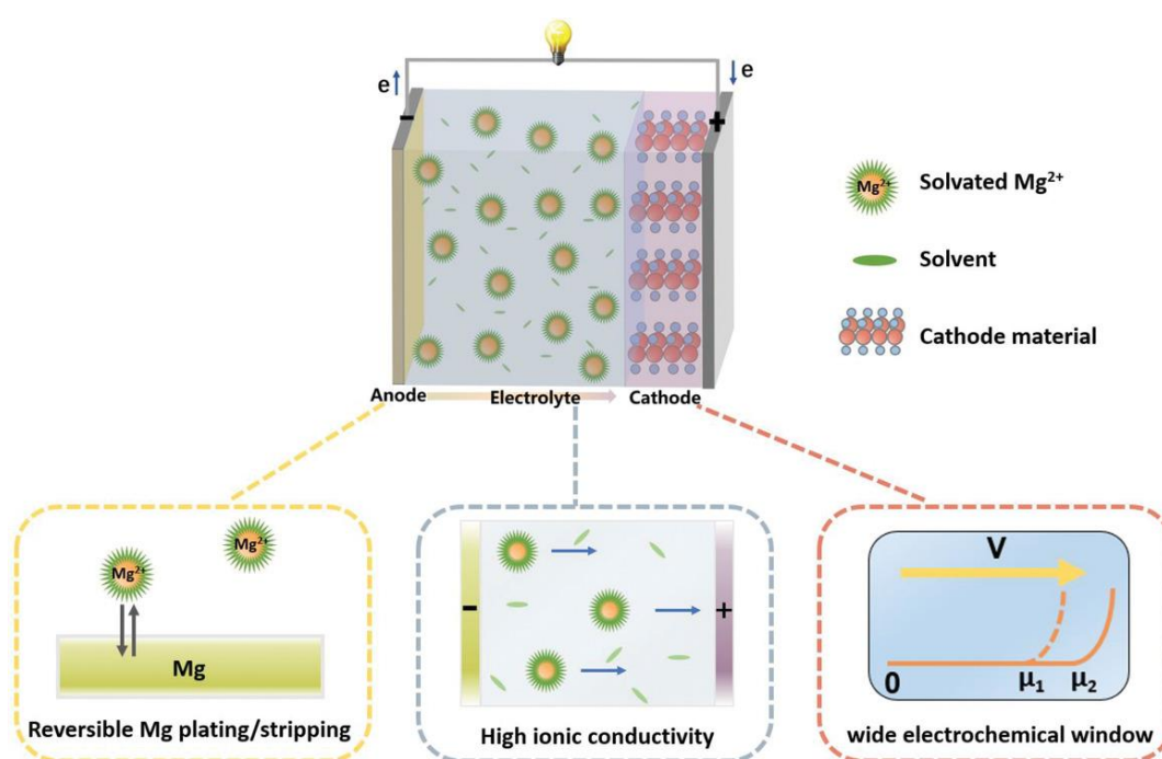
Figure. 1-3 Schematic illustration of main prerequisites for rechargeable magnesium battery electrolytes. 35
