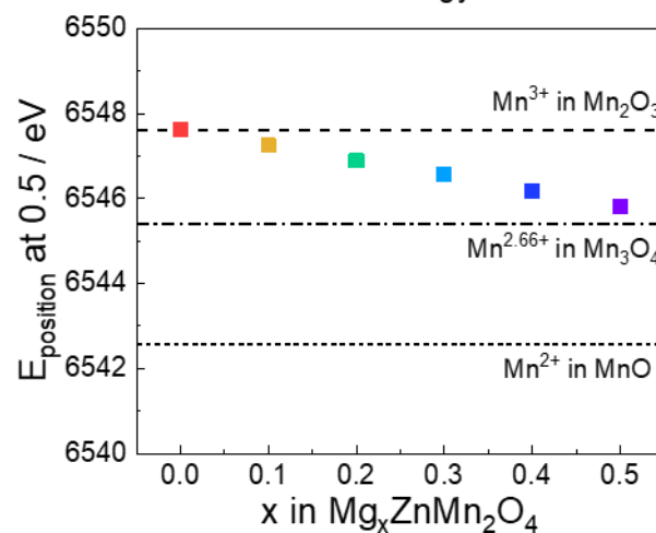
Figure 6-7. (a) Mn K -edge XANES of ZnMn 2 O 4 before and after Mg 2+ insertion and (b) energy at a normalized intensity of 0.5 in the XANES.
