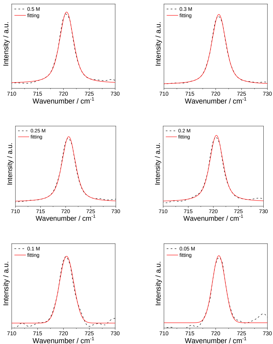
Figure 3-8. Raman spectra and Voigt function fitting results of \text{Mg}[\text{B}(\text{HFIP})_4]_2/2\text{-MeTHF} in several concentrations in the wave number between 710 and 730 \text{cm}^{-1} .
