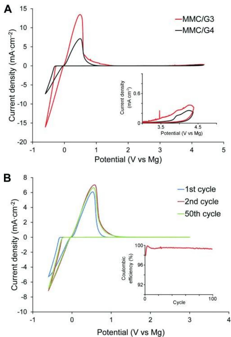
Figure. 1-9. (A) First cyclic voltammetry test of 0.75 M MMC/G3 and 0.75 M MMC/G4 on Pt electrode. (B) Selected cyclic voltammograms of 0.75 M MMC/G4 electrolyte on Pt electrode. 64
