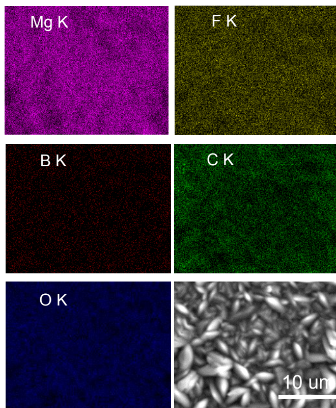
Figure 3-3. (a) SEM image, (b) EDX mapping and spectrum of Pt substrate after electrochemical measurements in 0.3 M \text{Mg}[\text{B}(\text{HFIP})_4]_2/\text{triglyme} .
