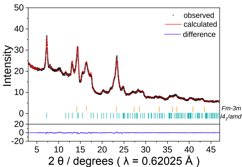
Figure 5-11. XRD pattern and Rietveld analytical fitting profile of the \text{Mg}_{1.54}\text{Mn}_2\text{O}_4 cathode sample.
