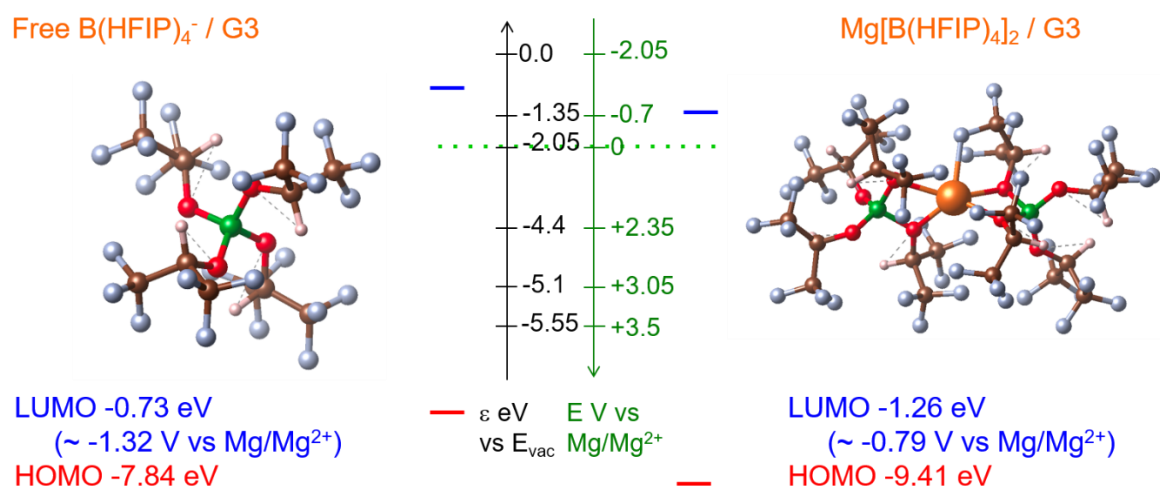
Figure 4-7. DFT cluster calculations of free [B(\text{HFIP})_4]^- and in contact [B(\text{HFIP})_4]^- .
