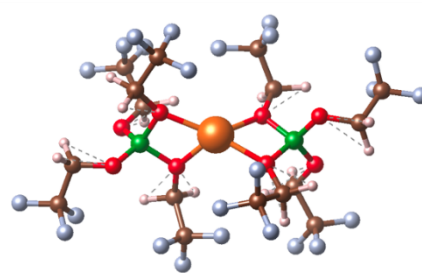
\text{Mg}[\text{B}(\text{TfE})_4]_2 / G3
