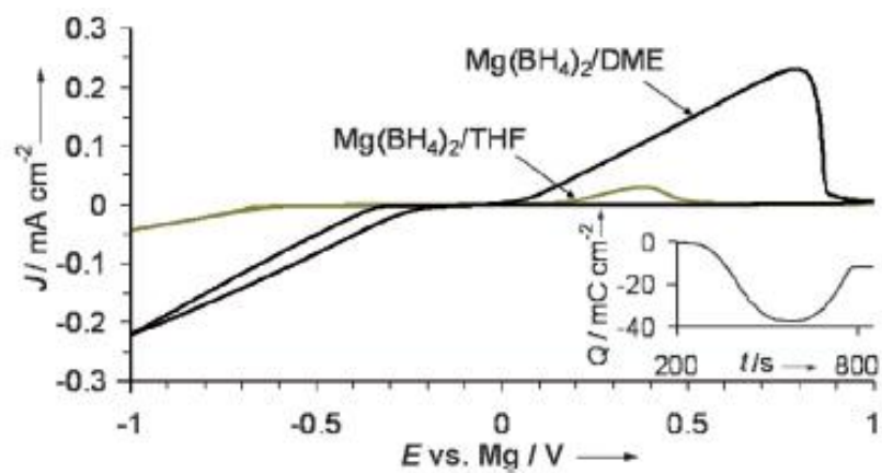
Figure. 1-5. Cyclic voltammetry of \text{Mg(BH}_4)_2/\text{glyme} and \text{Mg(BH}_4)_2/\text{THF} electrolytes. 59
