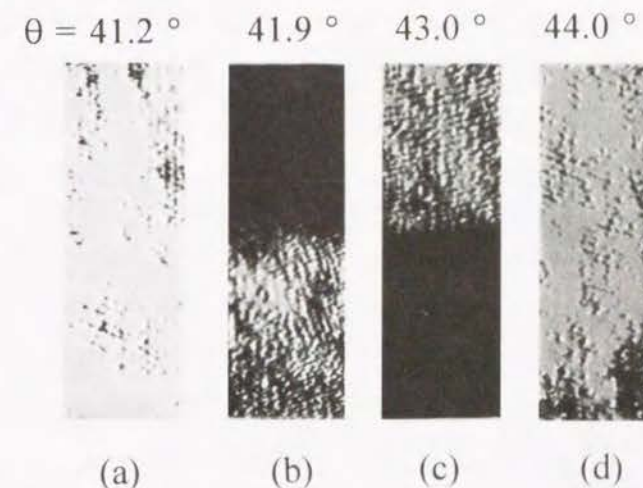
Figure 5-9. Surface plasmon microscopic image of 4 layers of PVO and 8 layers of P(VO-VC) LB film: (a) \theta = 41.2^\circ (b) \theta = 41.9^\circ (c) \theta = 43.0^\circ (d) \theta = 44.0^\circ
