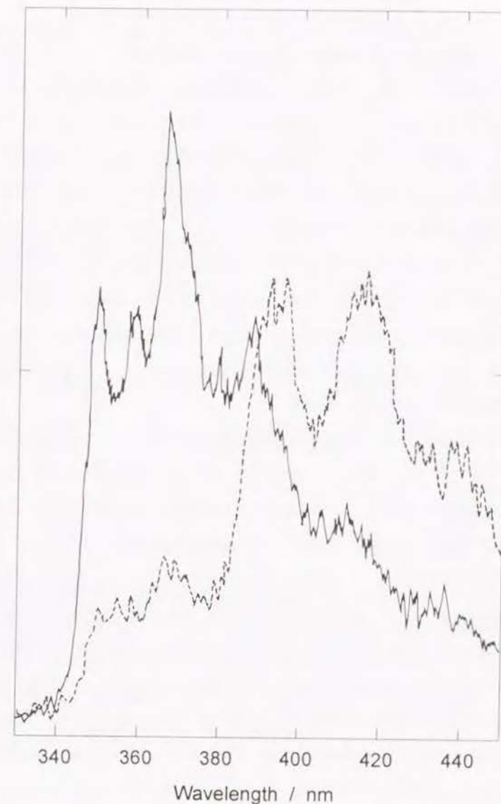
Figure 3-3. Spectral change of PDiPF(H)-P4A by heating up to 100^\circ\text{C} : (a) at room temperature (solid line) and (b) at 100^\circ\text{C} (dashed line).
