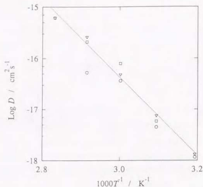
Figure 1-6. Arrhenius plot of diffusion constant of chromophores: (○) PVPe-P0A, (▽) PVPe-P4A, (□) PVPe-P8A.
