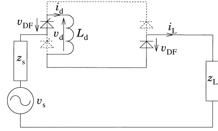
Fig. 4. Circuit diagram at charging mode of reactor.
