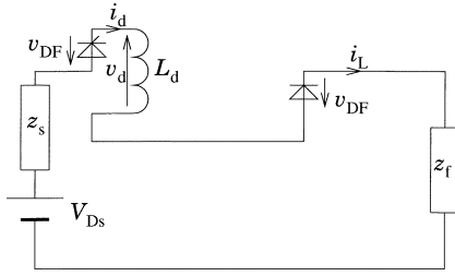
Fig. 9. Alternative circuit diagram at current limiting mode.
