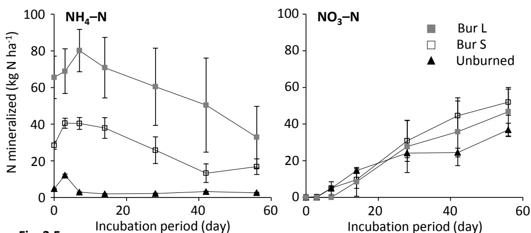
Fig. 3.5 The amount of NH 4 -N and NO 3 -N at a depth of 0–15 cm during the incubation experiment. Bars indicate standard error ( n = 3 ).
