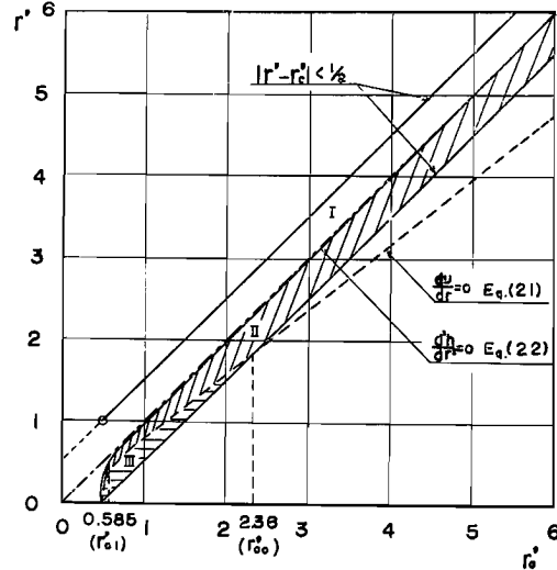
Fig. 2. Characteristic curves of dU/dr=0 [Eq. (21)] and d^2h/dr^2=0 [Eq. (22)] ( r'_c = r_c/B , r' = r/B ). Region I: dU/dr > 0 , d^2h/dr^2 > 0 , Region II: dU/dr > 0 , d^2h/dr^2 < 0 , Region III: dU/dr < 0 , d^2h/dr^2 < 0 .
