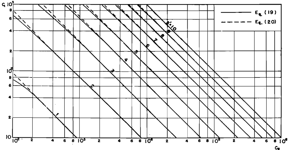
Fig. 1. An example of relation between C_1 and C_2 ( g=980 cm/sec 2 , i=2 \times 10^{-3} and B=25 cm).
