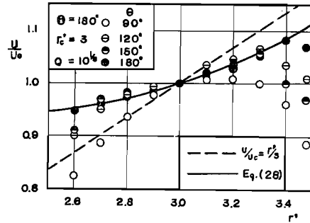
Fig. 10. Comparison between theoretical velocity profile and experimental data with constant discharge at different stations.
