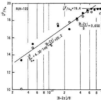
Fig. 3 Lateral distribution of depth-wise average velocity.
