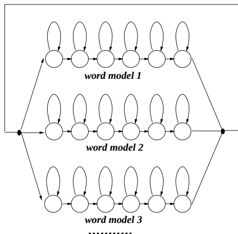
Figure 5.4: Word-concatenation model
