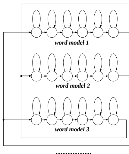
Figure 5.5: Word-pair model
