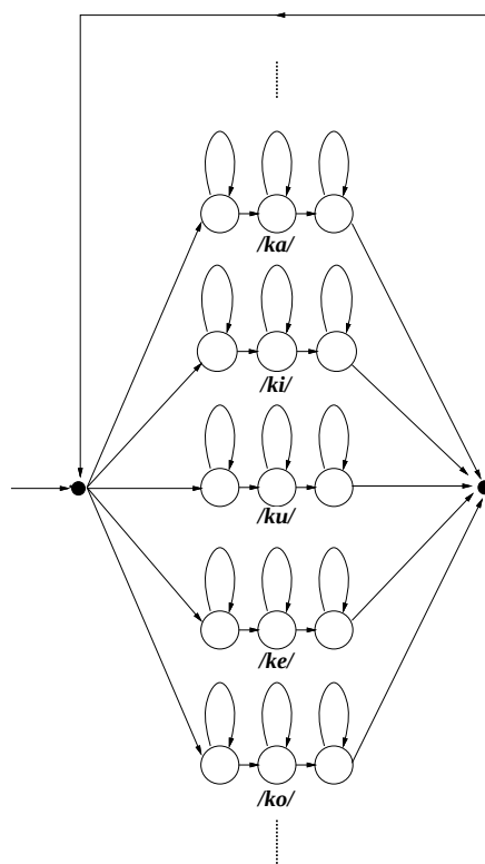
Figure 5.3: Syllable-concatenation model
