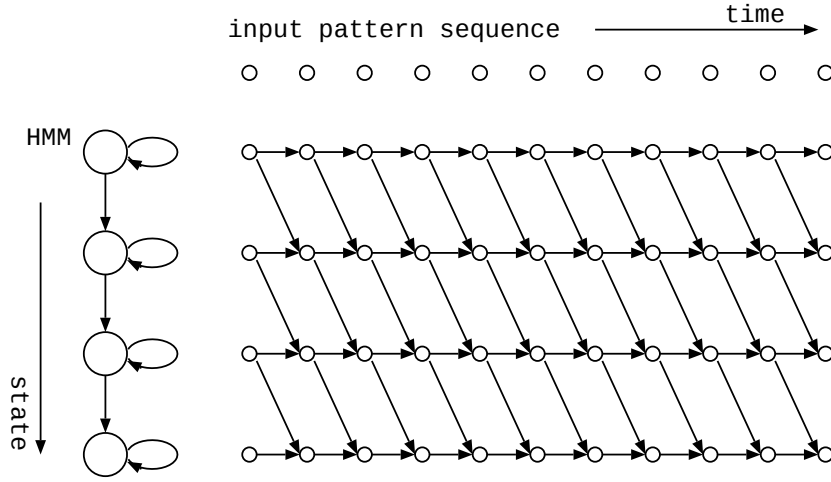
Figure 2.4: HMM trellis
