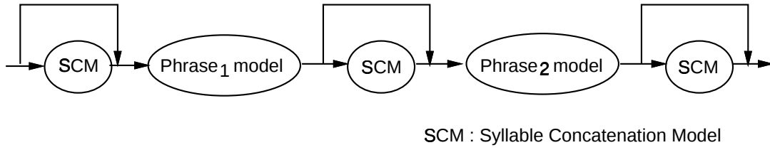
Figure 5.12: Sentence hypothesis model based on phrase spotting
