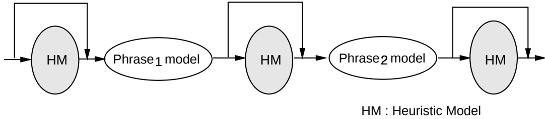
Figure 5.14: Island-driven search based on phrase spotting
