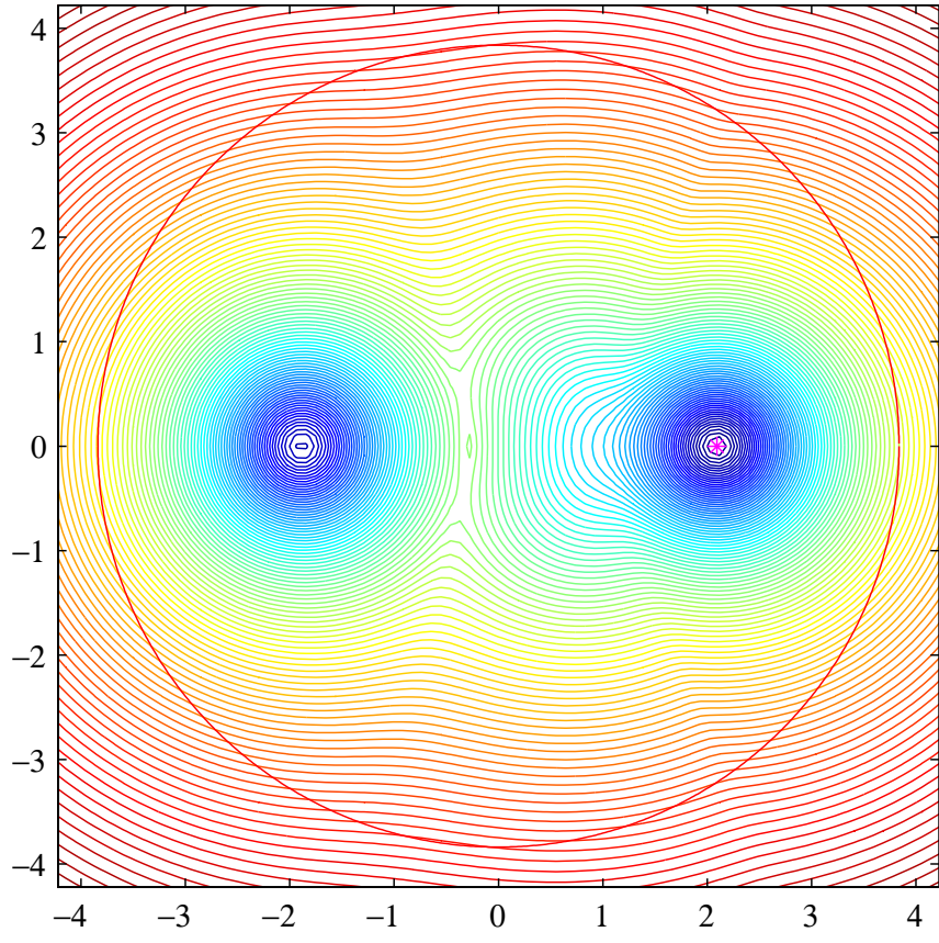
Figure 5: Contour plots of \log_{10}(\sigma_{\min}([A - zI \ B])) for the pair (31). The circle is of radius \gamma_l = 3.8390 . The mark * denote the location of the optimizer z^* = 2.0934 .
