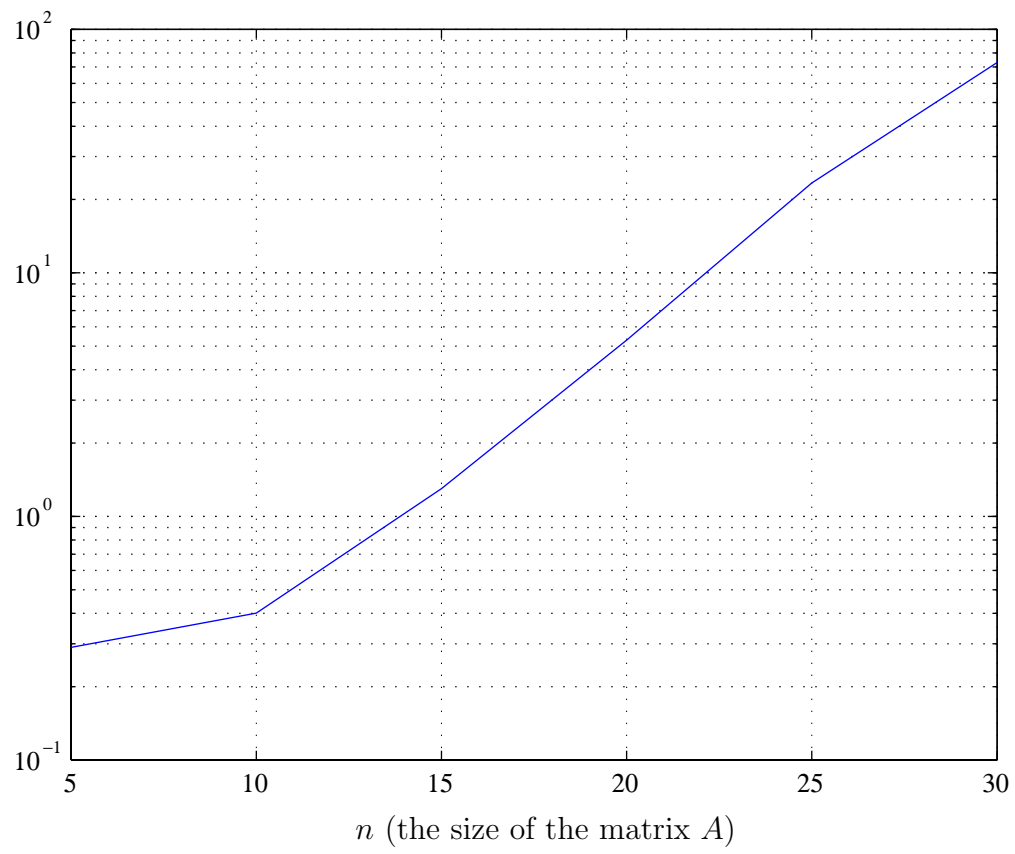
Figure 4: Average CPU time to compute \varepsilon_2^* in logarithmic scale.
