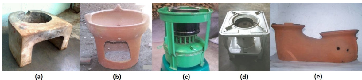
Figure 4.9 Stove types for WBT test (a. wood stove, b. charcoal stove, c. kerosene stove, d. JCS stove, e. improved wood stove-SAE stove)
