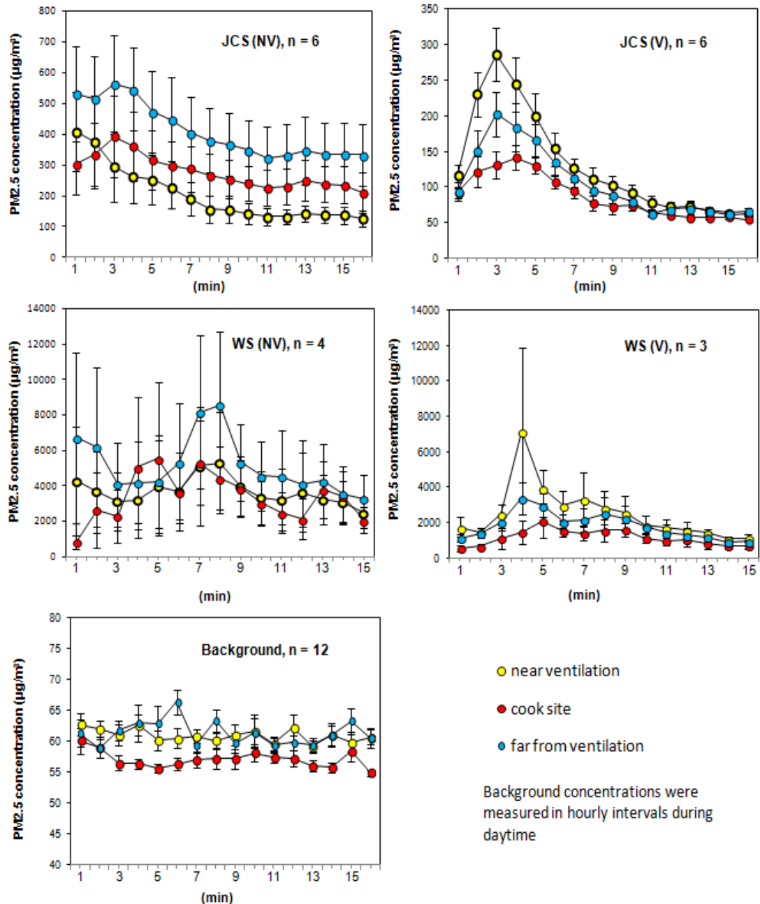
Figure 4.13 Average temporal PM 2.5 mass concentrations during stove combustion as well as background condition with and without ventilation.
