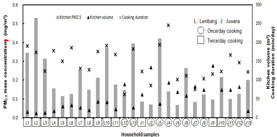
Figure 3.5 Indoor PM 2.5 concentrations in the household kitchens
