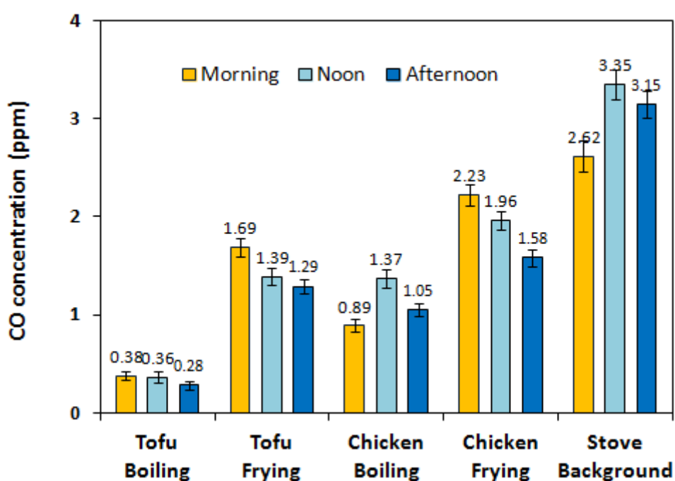
Figure 4.7 Average CO concentrations during cooking
