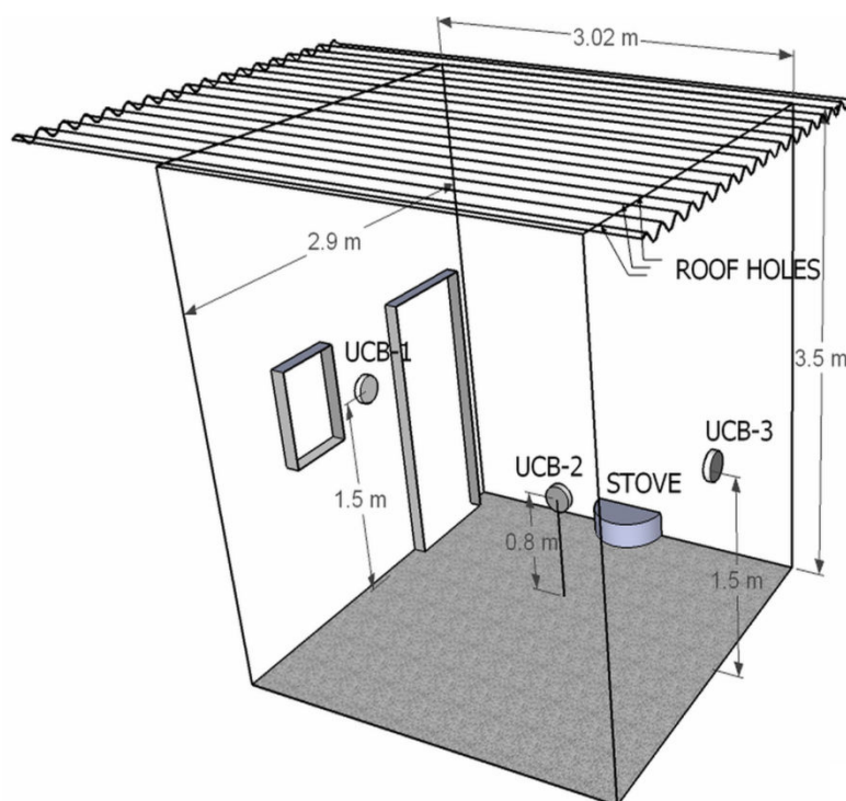
Figure 4.10 Schematic view of simulated kitchen
