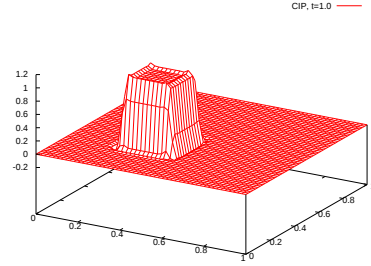
CIP t = 1.0
