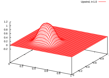
Upwind t = 1.0
