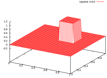
Upwind t = 0
