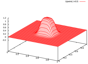
Upwind t = 0.5
