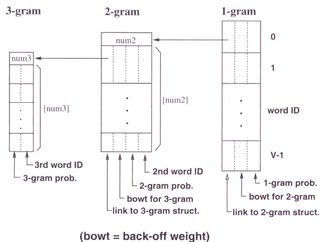
Figure 2.17: N-gram data structure
