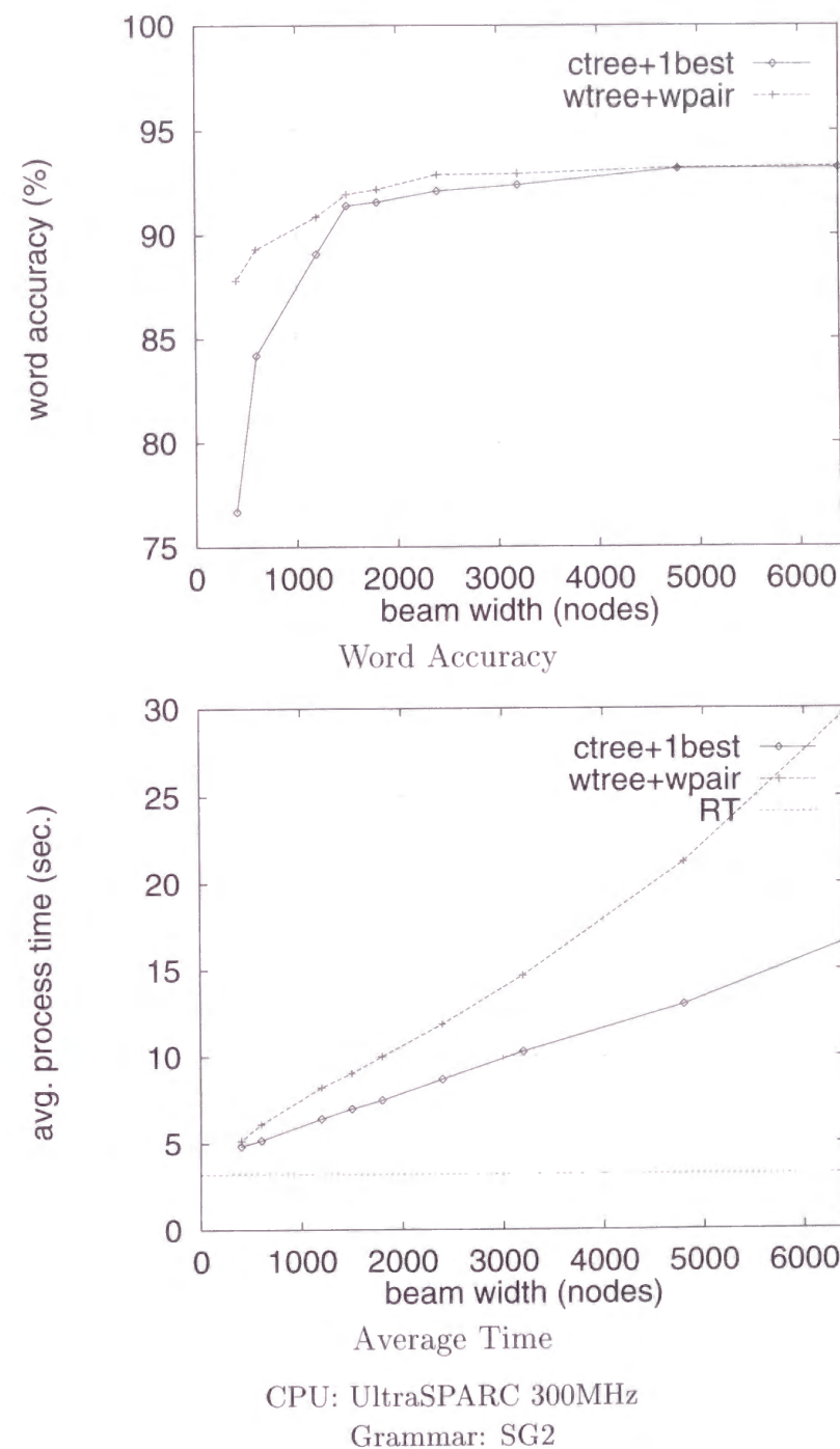
Figure 3.7: Comparison of static and dynamic expansion of category-pair network
