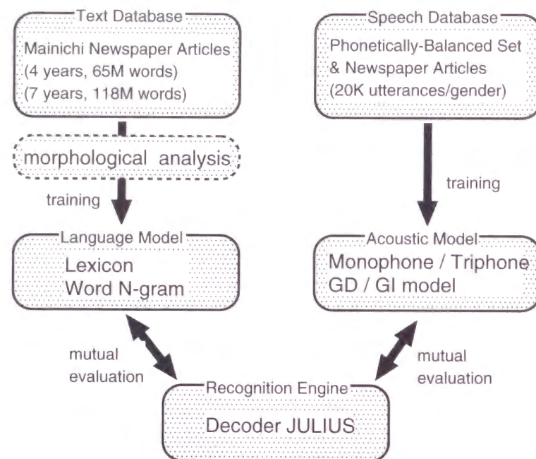
Figure 5.1: Platform of LVCSR
