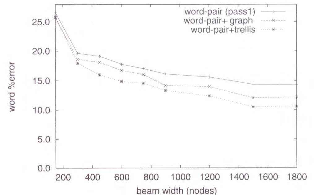
Figure 2.19: Comparison of trellis and graph (Word %Error)
