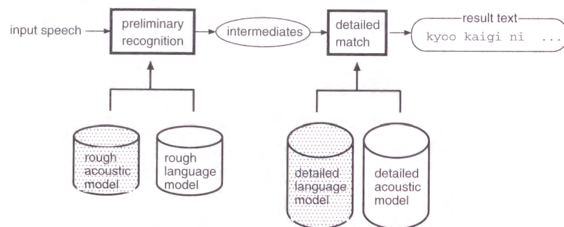
Figure 2.6: An LVCSR system using multi-pass search
