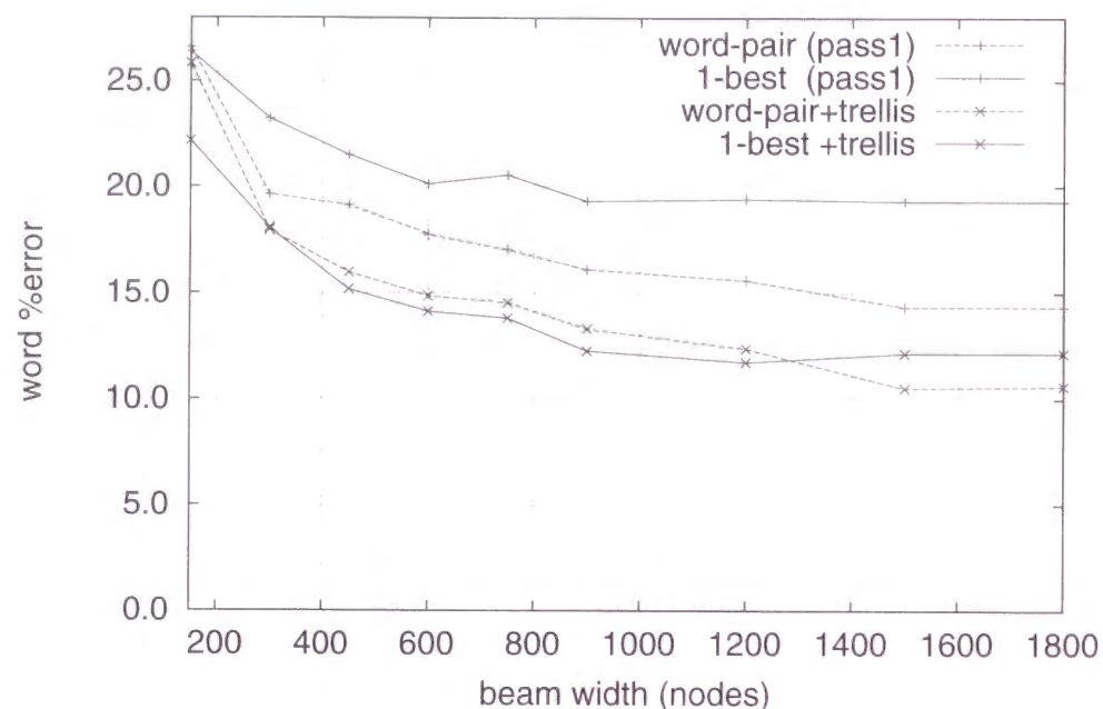
Figure 2.20: Comparison of word-pair and one-best (Word %Error)
