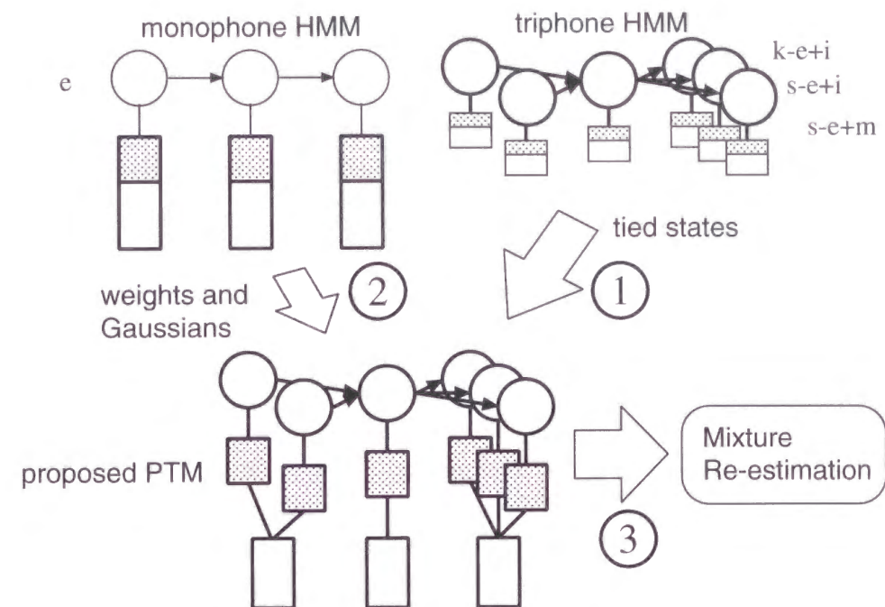
Figure 4.1: Building proposed PTM HMM
