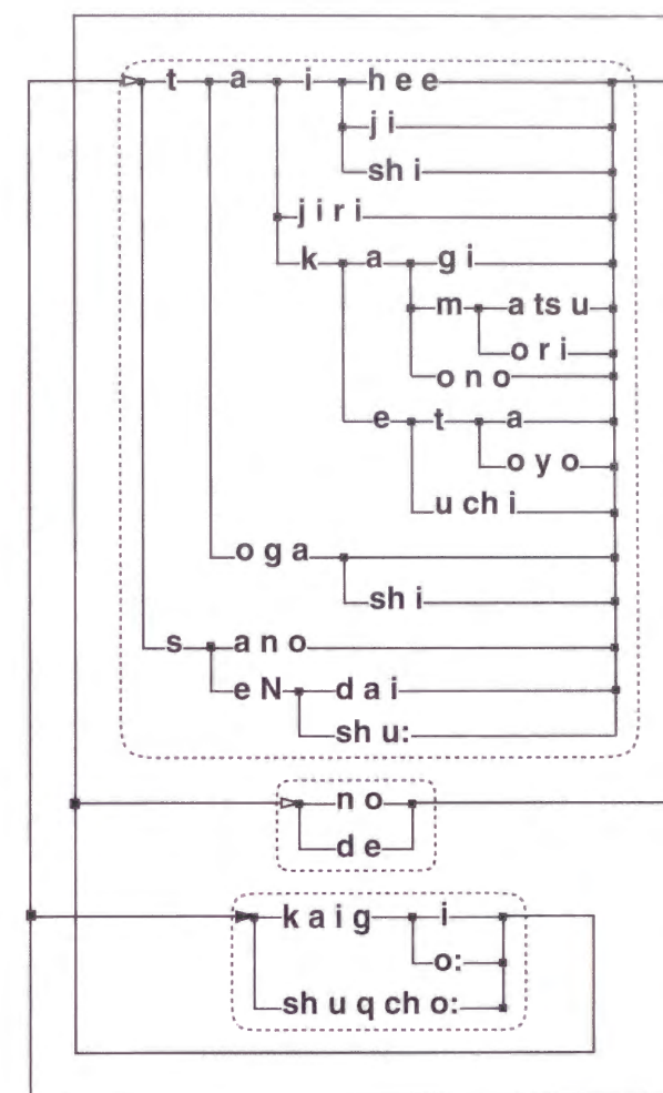
Figure 3.2: Tree-structured category-pair network
