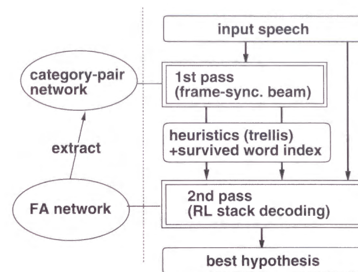
Figure 3.3: Overview of parsing algorithm
