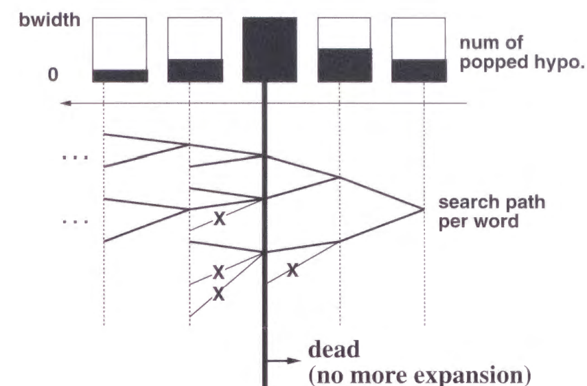
Figure 2.18: Enveloped best-first search
