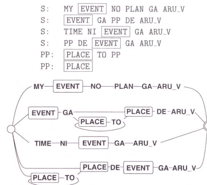
Figure 3.1: A typical recognition grammar and its expanded network
