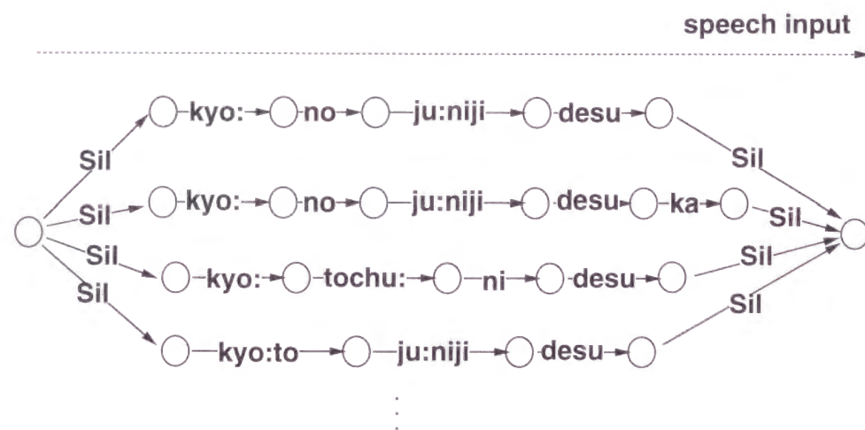
Figure 2.9: N-best candidates
