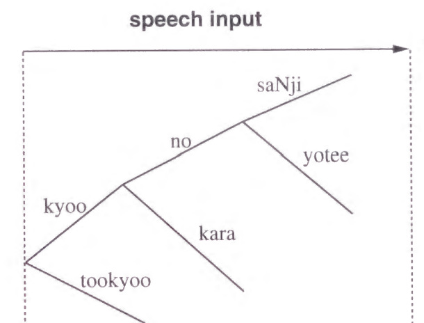
Figure 2.2: Frame asynchronous search
