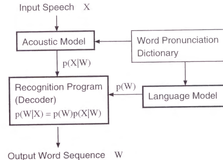
Figure 1.1: Continuous speech recognition
