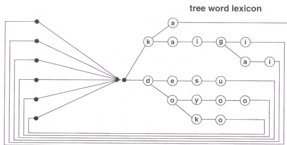
Figure 2.15: Word tree lexicon
