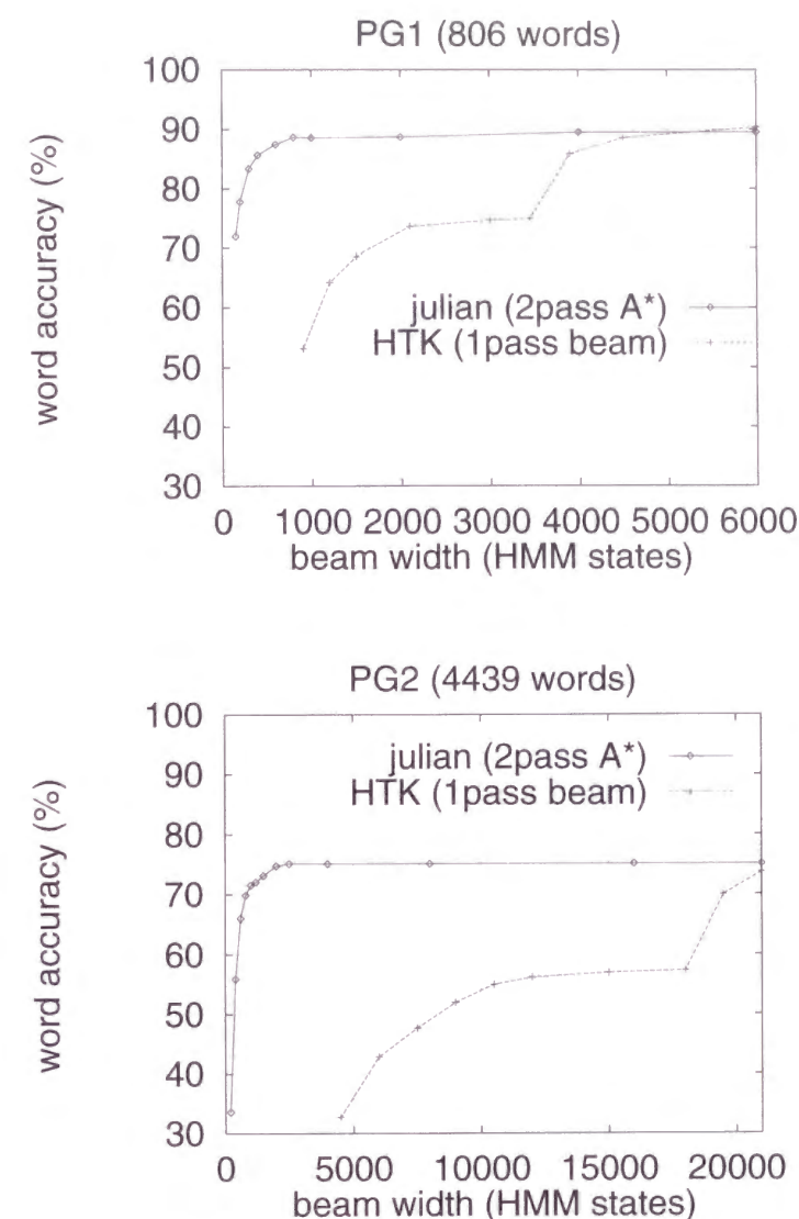
Figure 3.6: Comparison of search algorithms
