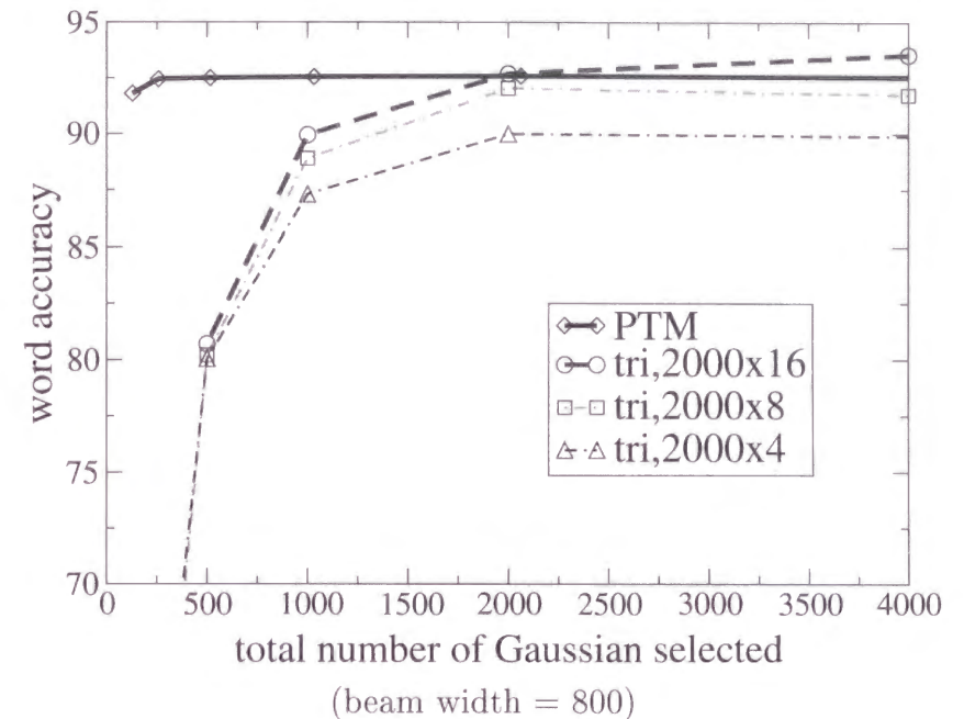
Figure 4.2: Accuracy decrease by Gaussian pruning
