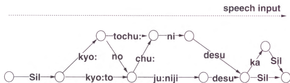
Figure 2.10: Word-graph form
