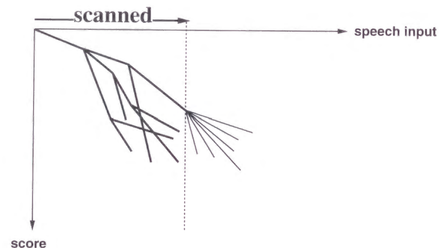
Figure 2.3: One-pass search
