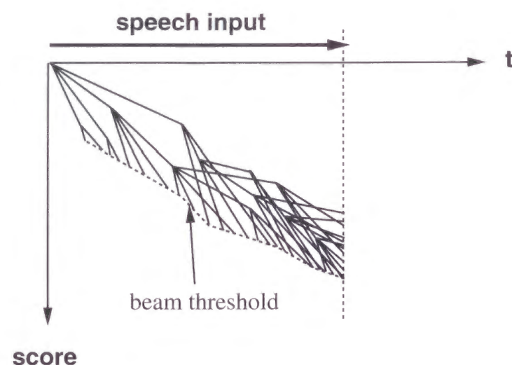
Figure 2.1: Frame synchronous search
