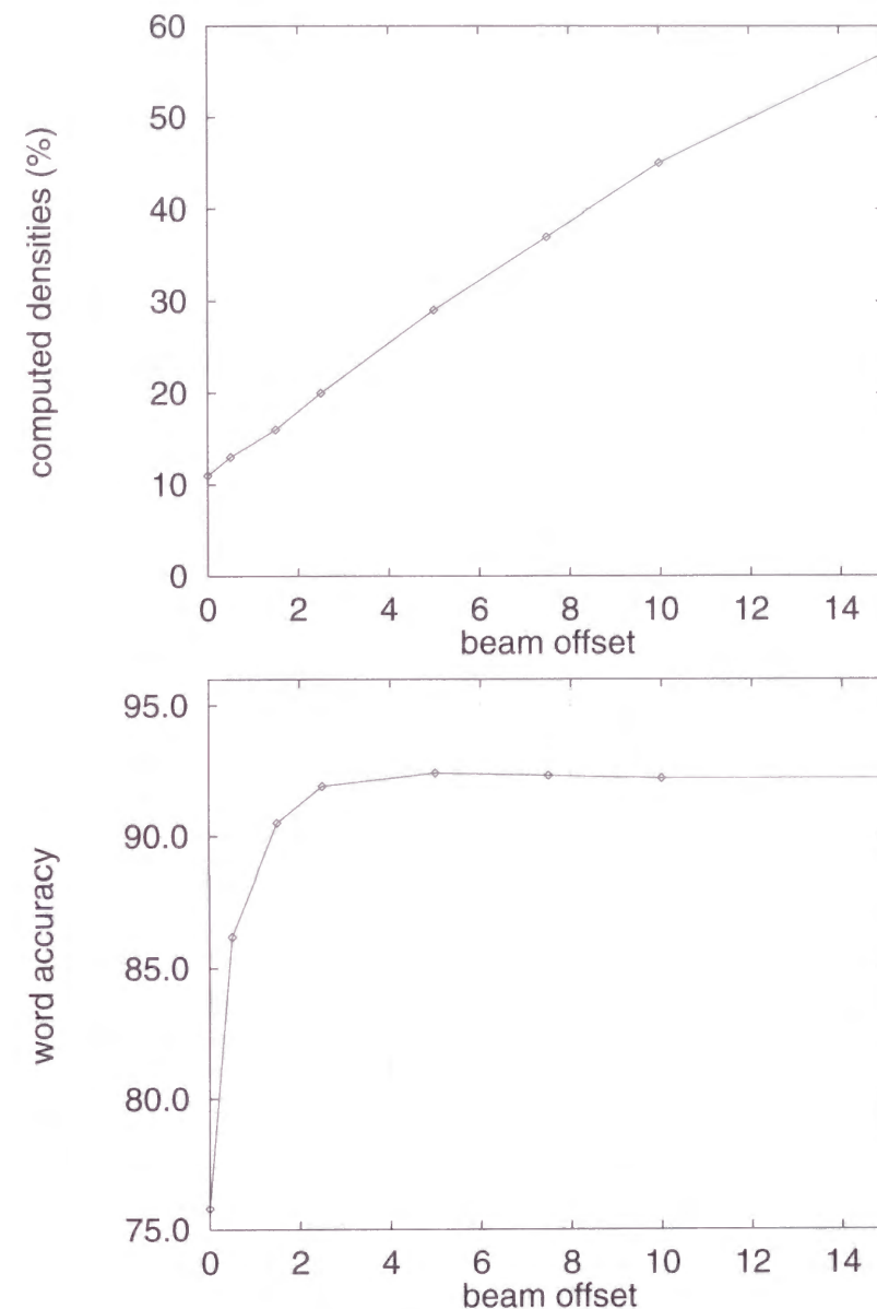
Figure 4.3: Beam pruning offset vs. performance
