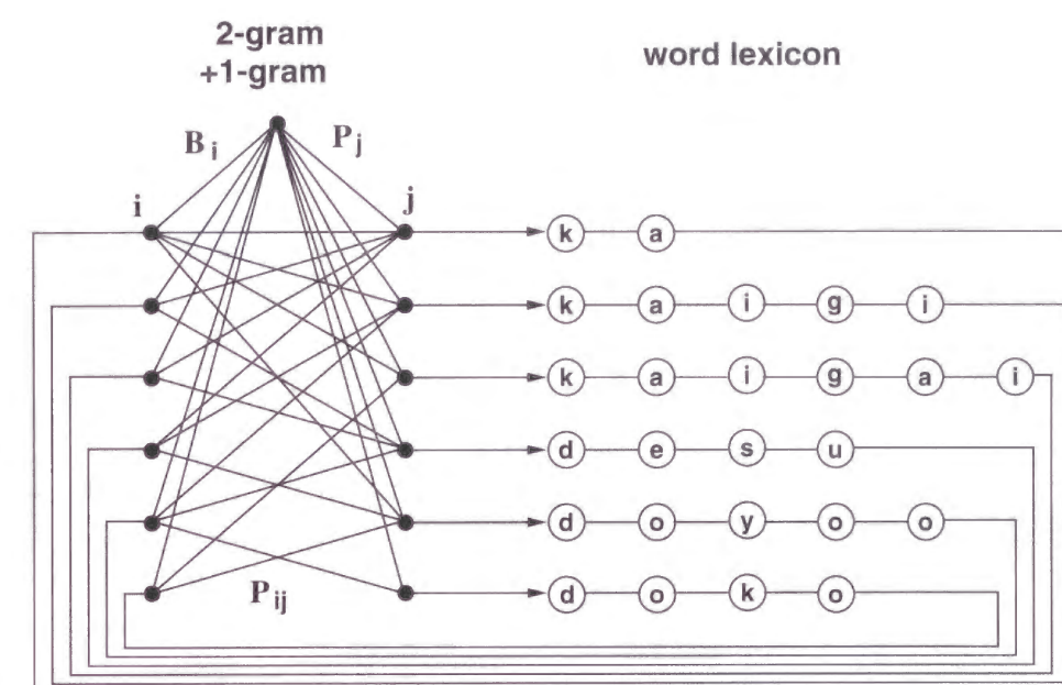
Figure 2.14: Word lexicon with back-off 2-gram
