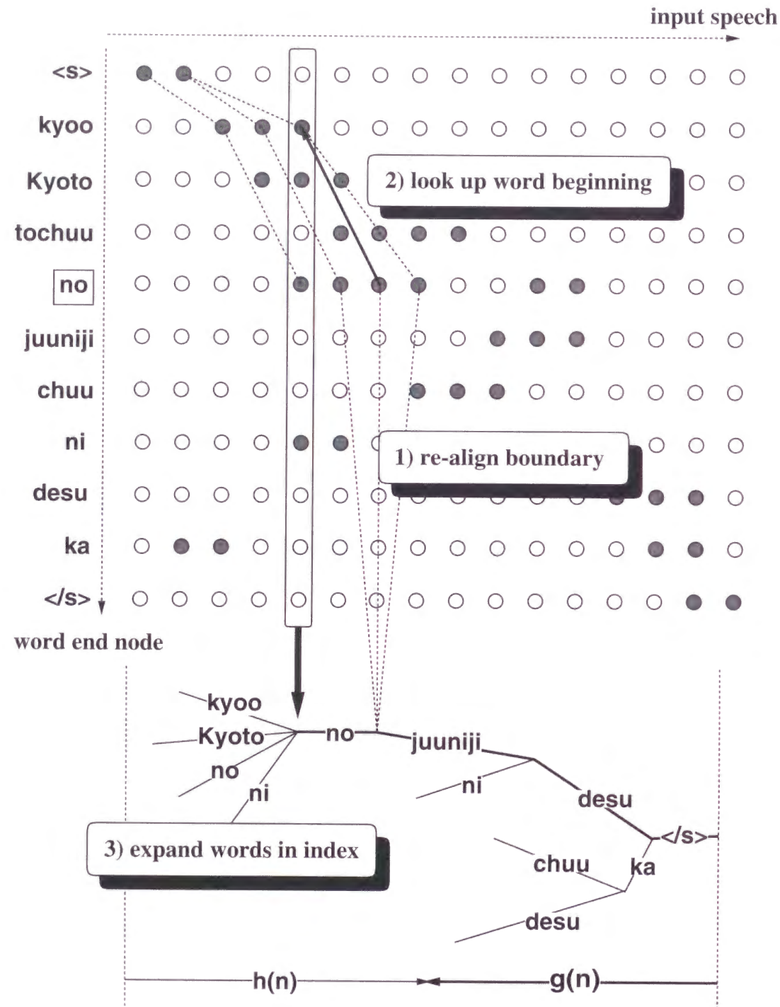
Figure 2.12: Word trellis index and its use on the second pass
