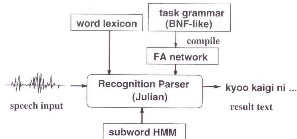
Figure 3.4: Recognition system based on CSR parser Julian
