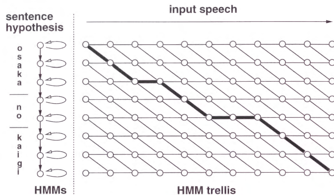
Figure 1.2: Viterbi algorithm on HMM trellis
