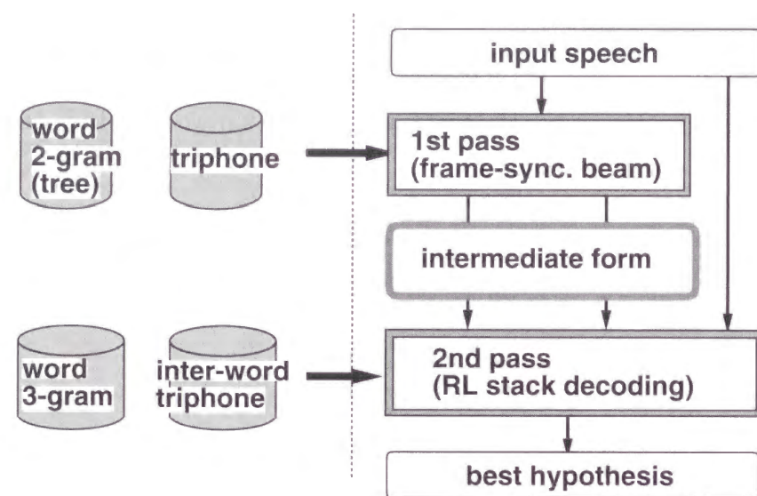
Figure 2.13: Overview of Julius
