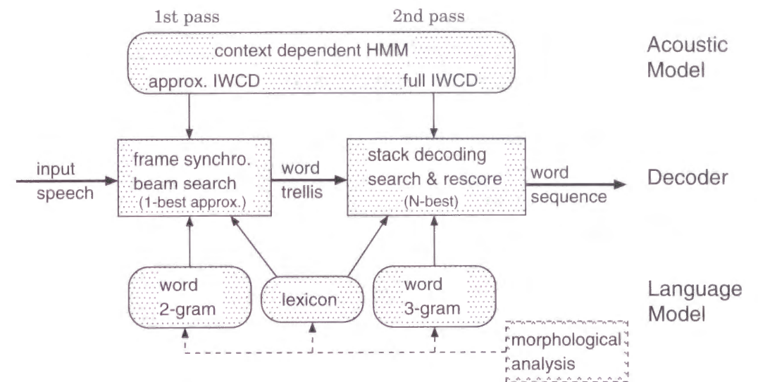
Figure 5.2: Block diagram of Japanese dictation system
