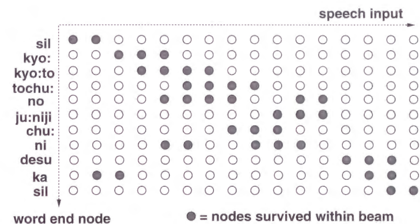
Figure 2.11: Trellis form
