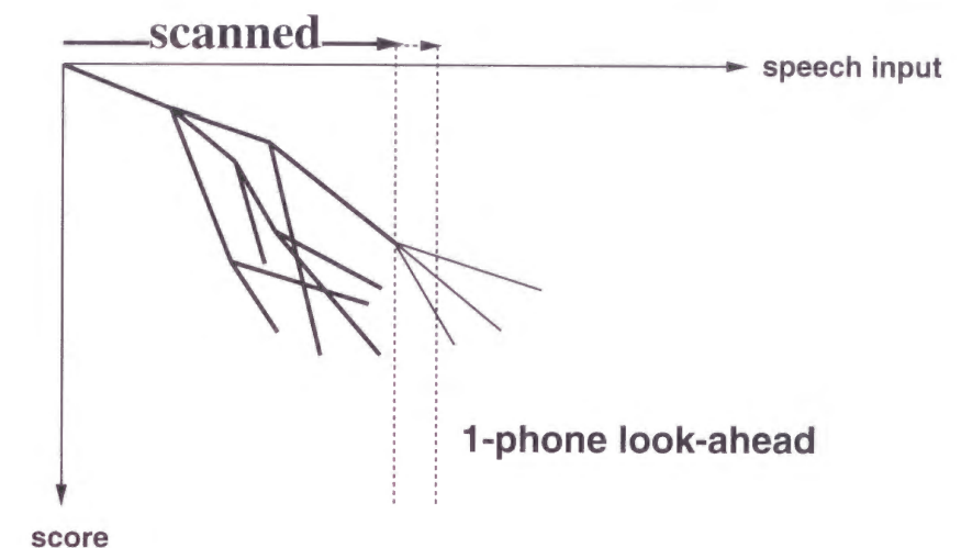
Figure 2.4: Fast match
