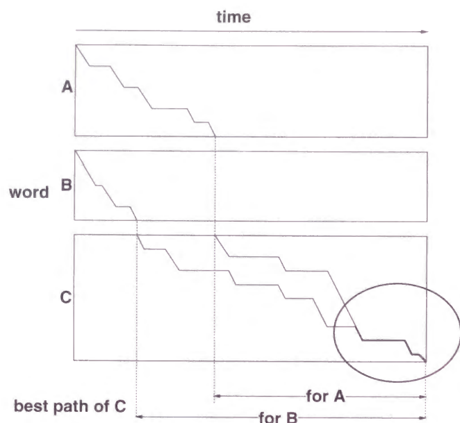
Figure 2.7: Word-pair approximation
