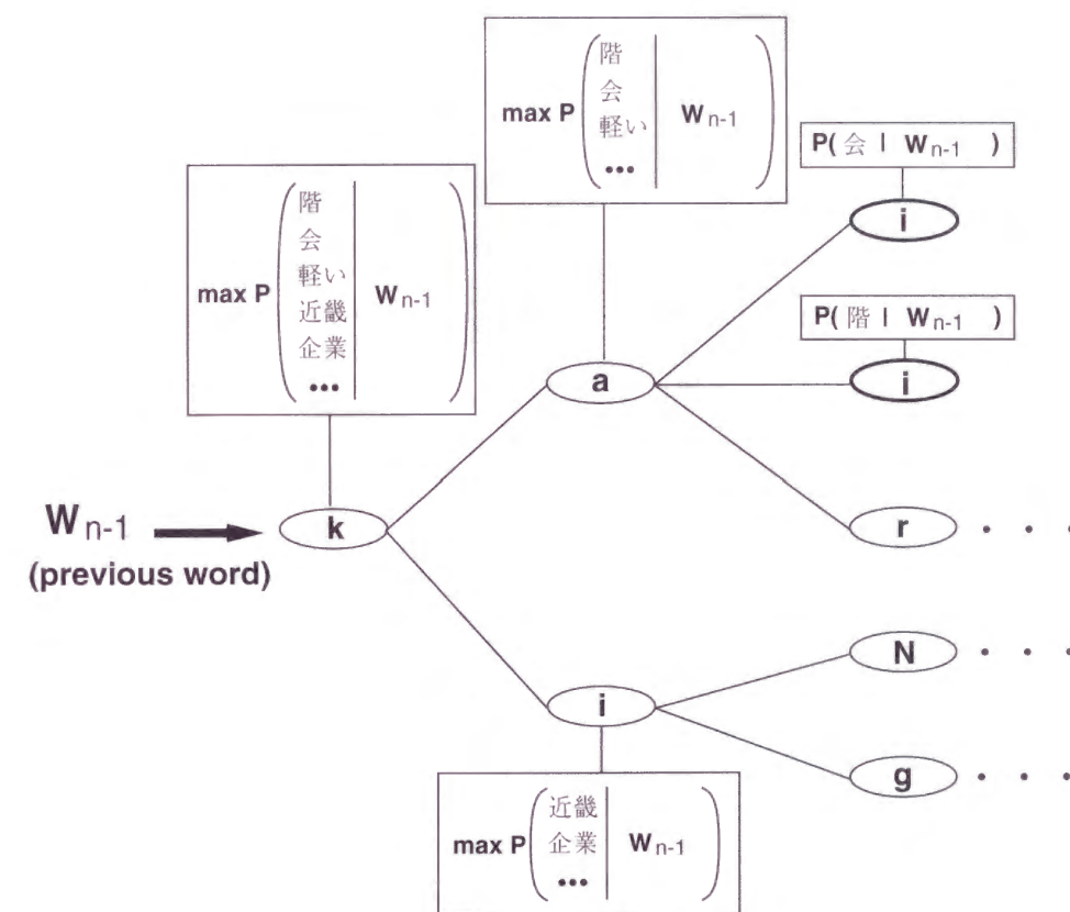
Figure 2.16: N-gram factoring
