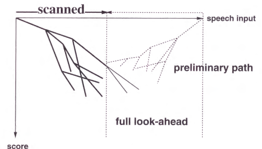
Figure 2.5: Multi-pass search
