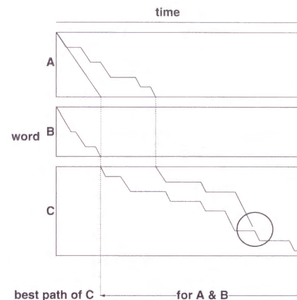
Figure 2.8: One-best approximation
