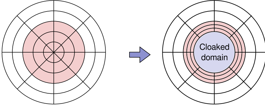
Figure 1.6: Pendry's construction of cloaking device - Red region is transformed.
