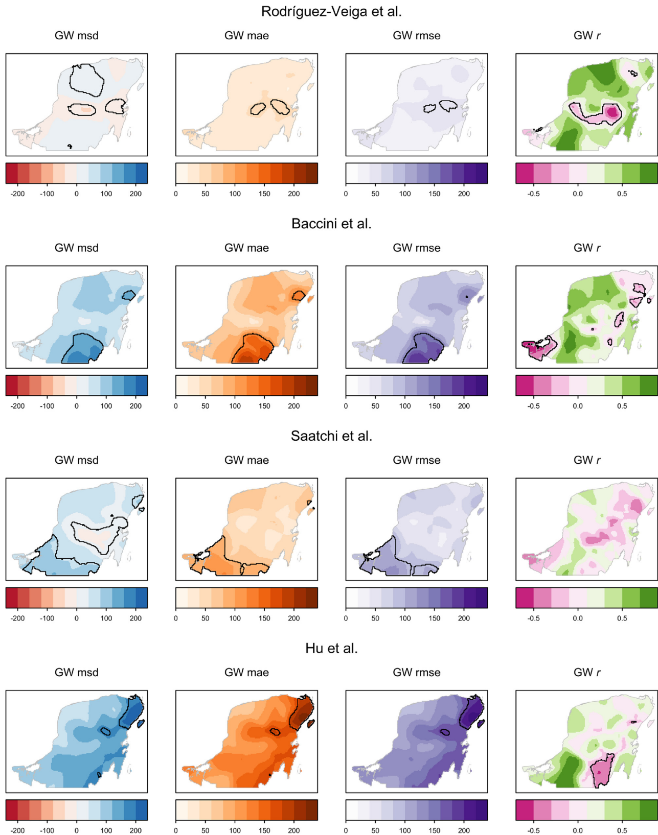
Fig. 6. Spatial distributions of GW msd, GW mae, GW rmse, and GW r for four forest aboveground biomass datasets of Rodríguez-Veiga et al. (2016); Baccini et al. (2012); Saatchi et al. (2011), and Hu et al. (2016) for study 2. Black polygons represent ‘significant’ ( p -values less than 0.01) areas by Monte Carlo permutation tests.
