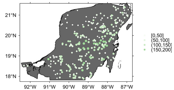
Fig. 4. The spatial distribution of in-situ reference sample points for forest aboveground biomass data (units: Mg ha -1 ) in the Yucatan peninsula, Mexico.
