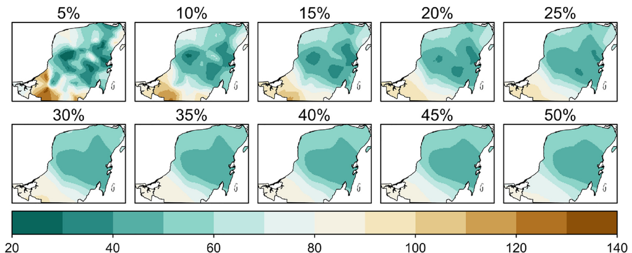
Fig. 7. Comparison of results of GW mae for Saatchi's aboveground biomass dataset with different adaptive kernel size between 5%–50% as an example.
