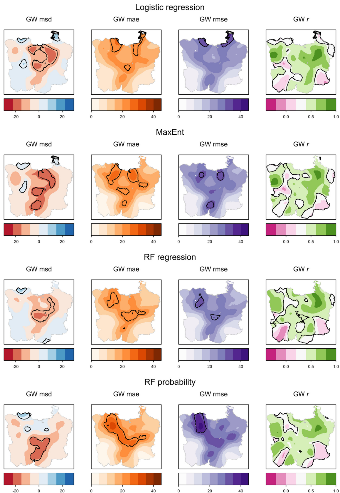
Fig. 5. Spatial distributions of GW msd, GW mae, GW rmse, and GW r for fractional impervious surface area predicted from logistic regression, MaxEnt, RF regression, and class probability of RF classifiers for study 1. Black polygons represent 'significant' ( p -values less than 0.01) areas by the Monte Carlo permutation tests.
