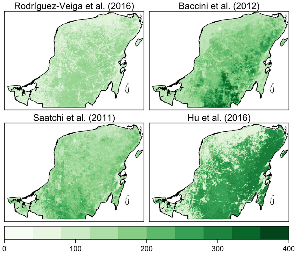
Fig. 3. Four aboveground biomass datasets (units: \text{Mg ha}^{-1} ) for the Yucatan peninsula, Mexico for study 2.
