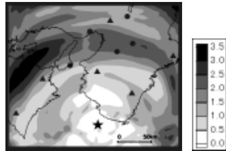
Fig. 10. Distribution map of the waveform difference (D) in the period range of 2-5s. Star indicates the location of epicenter. Circles and triangles are location of observatories of CEORKA and F-net.
