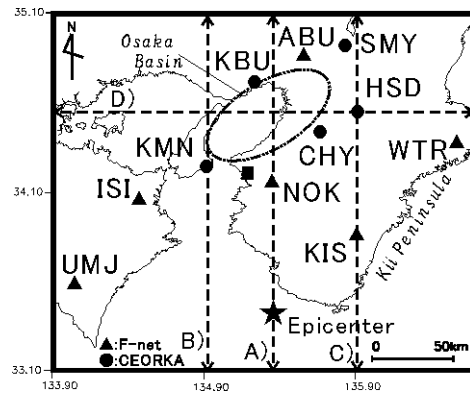
Fig.2. Map of analysis area. Triangles (F-net) and circles (CEORKA) are the locations of the rock site stations. Star and square show an epicenter of an earthquake M_w 4.3 and the location of Wakayama observatory. Broken lines of A)~D) indicate the location of model profiles shown in Fig. 4.
