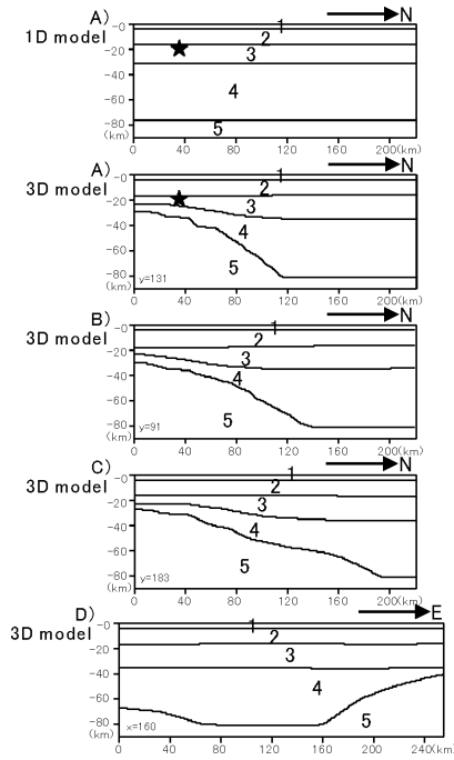
Fig. 4. Model profiles at the location of the broken lines of A)~D) in Fig. 2. Top figure is a profile of '1D model', the others are profiles of '3D model'. Profile A) crosses the hypocenter. Star shows the hypocenter of M_w 4.3 event.
