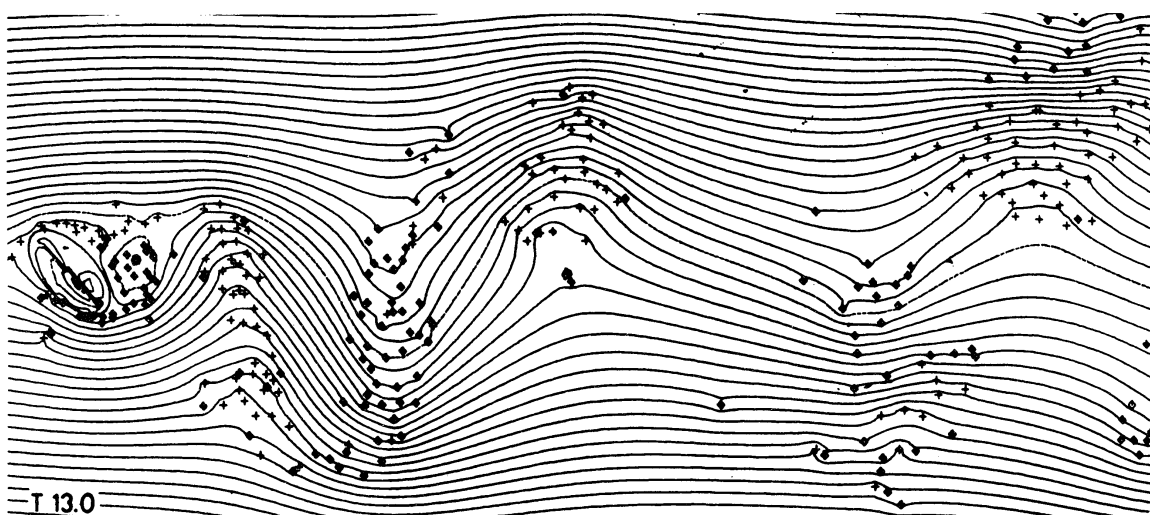
Fig.1 Vortex arrangements and stream lines ( 45^\circ ). Mark + and \times are vortex filaments with clockwise and counter-clockwise rotations respectively.
