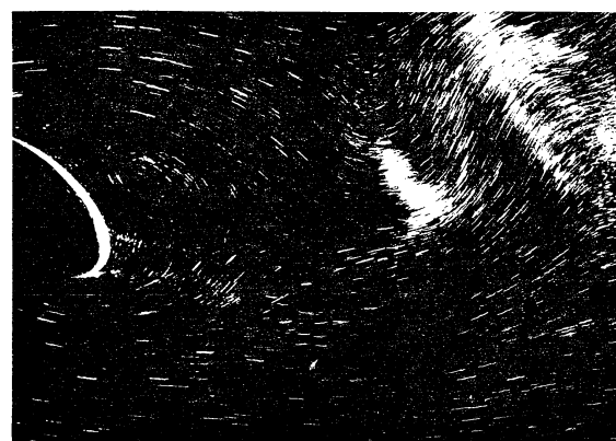
Fig.3 Stream lines ( 45^\circ ); Experiment, T = 7.8 .
