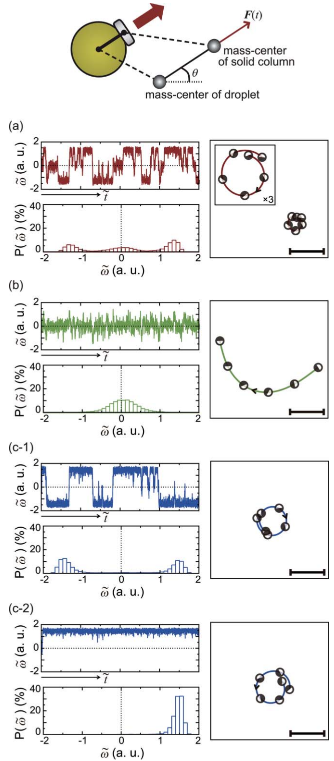
FIG. 5. Numerical simulation based on Eqs. (5)–(7). The top panel shows a frame format of the model. Left: Time traces of the angular velocity \tilde{\omega} and histograms of \tilde{\omega} ( 0 \leq \tilde{t} \leq 1000 ). Right: Trajectory of the centroid of the composite in \mathbf{r} space for a short period ( 400 \leq \tilde{t} \leq 405 ). The scales are the same on the four trajectories except for the inset. (a) \alpha = 2.4 , s = 0.3 . (b) \alpha = 1.8 , s = 0.3 . (c-1) \alpha = 2.7 , s = 0.5 . (c-2) \alpha = 2.7 , s = 0.3 . The other fixed parameters are \tilde{\eta}_1 = 1 , \beta = 1 , \tilde{F} = 0.1 . The initial values are \tilde{x}(0) = \tilde{y}(0) = 0 , \tilde{v}_x(0) = \tilde{v}_y(0) = 0 , \theta(0) = 0 , and \tilde{\omega}(0) = 0 .
