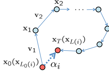
Fig. 5.6 Modifying the trajectory by loop closure. In step T , the robot detects a loop closure between x_T and x_0 . When the loop closure is detected, the robot estimates the relative pose \alpha between these local maps by feature point correspondence and modifies the trajectory by minimizing Eq. (5.6).
