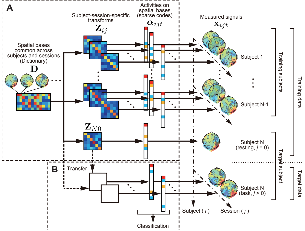
Fig. 4.2 The proposed method for multi-subject-session data analysis and subject-transfer decoding. (A) Measured signals are decomposed into three factors: dictionary (spatial bases) common across subjects and sessions \mathbf{D} , spatial transforms \mathbf{Z}_{ij} that modulate the common dictionary to be specific to subjects (indexed by i ) and sessions (indexed by j ), and sparse codes \alpha_{ijt} representing the use profile of the spatial bases. The dictionary and transforms are learned from the training data consisting of all sessions of training subjects and a resting session (indexed by j = 0 ) of a target subject (indexed by i = N ), in an unsupervised manner so that the signals in the training data can be well represented by a sparse combination of the spatial bases in the dictionary. (B) Subject-transfer decoding based on calibration using resting-state activities. For the target subject ( i = N ), the subject-session-specific transform for the resting-state activities, \mathbf{Z}_{N0} , is re-used as those for the task sessions, \mathbf{Z}_{Nj} ( j > 0 ). The two matrices \mathbf{D} and \mathbf{Z}_{N0} are obtained in the dictionary learning stage of (A) based on the training data, and are thus available before getting access to the EEG measurements of the target subject during the decoding task sessions. Using the EEG signals of the target subject during the decoding task, sparse codes \alpha are estimated and used for later classification.
