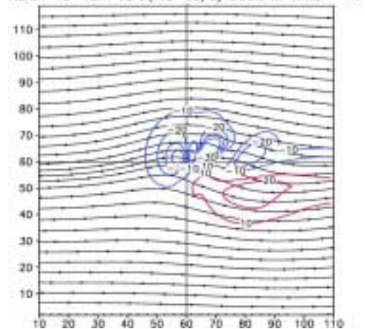
Fig.9(f) wind streamlines and vorticity at \tau = 17.0 on h5000m RUN3
