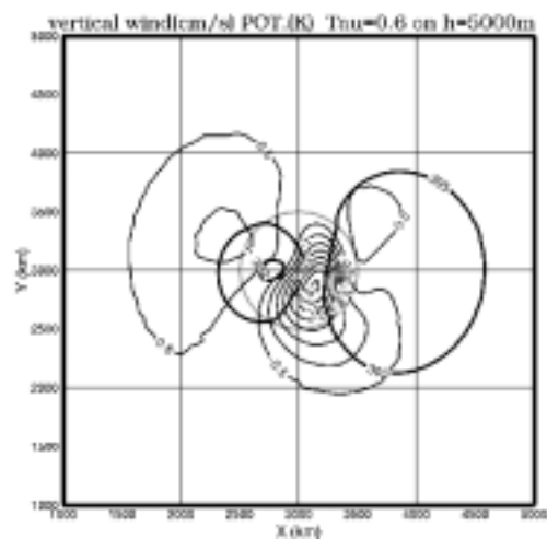
Fig.2(a) vertical wind and potential temperature distributions at \tau=0.6 , h=5000\text{m} , NO.01 U10m/s RUN1.
