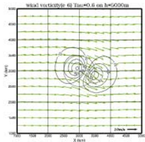
Fig.1(a) wind vector and vorticity distributions at
