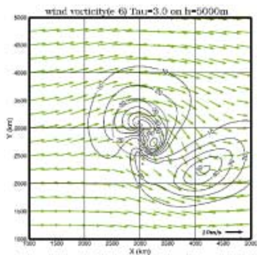
Fig.1(e) wind vector and vorticity distributions at \tau=3.0 , h=5000\text{m} , NO.01 U10m/s RUN1.
