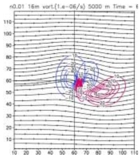
Fig.5(b) streamlines and vorticity at \tau = 1.2, N0.01, U16m on h5000m RUNs2
