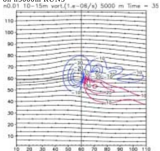
Fig.9(c) wind streamlines and vorticity at \tau=14.6 on h5000m RUN3
