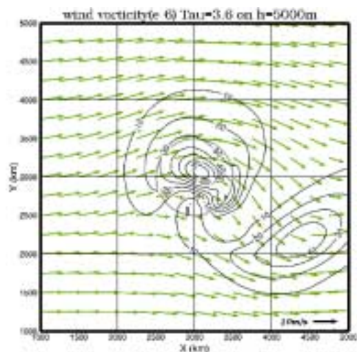
Fig.1(f) wind vector and vorticity distributions at \tau=3.6 , h=5000\text{m} , NO.01 U10m/s RUN1.
