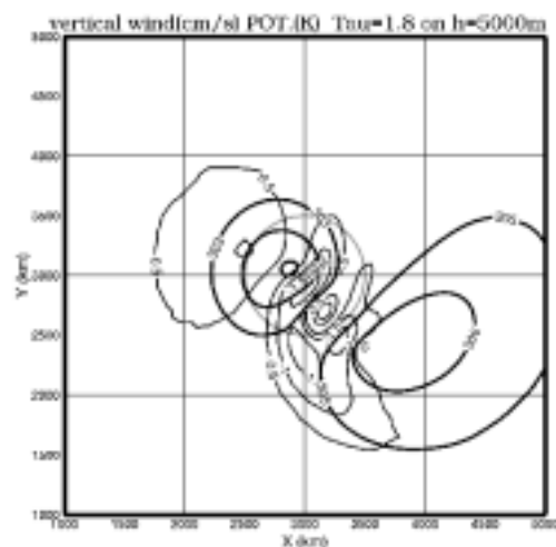
Fig.2(c) vertical wind and potential temperature distributions at \tau=1.8 , h=5000\text{m} , NO.01 U10m/s RUN1.
