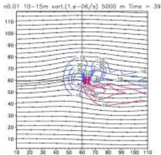
Fig.9(d) wind streamlines and vorticity at \tau = 15.4 on h5000m RUN3
