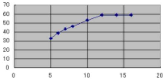
Fig.7(a) relation between cyclonic vorticity(row) and wind speed(column) at \tau = 0.6
