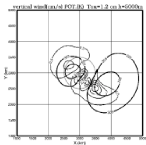
Fig.2(b) vertical wind and potential temperature distributions at \tau=1.2 , h=5000\text{m} , NO.01 U10m/s RUN1.
