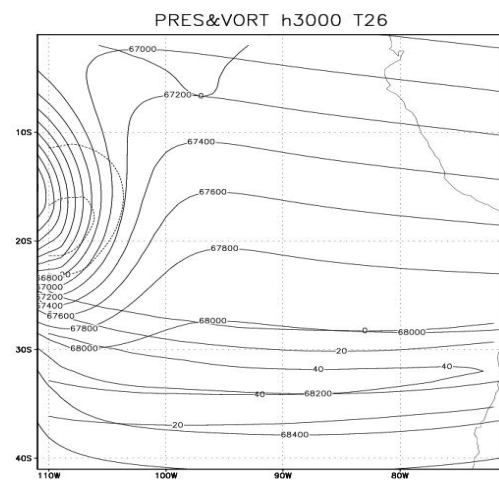
Fig.8(b) distributions of total pressure and vorticity at \tau = 12.5 , N0.01 U10m/s on h5000m
