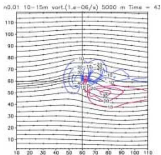
Fig.9(e) wind streamlines and vorticity at \tau = 16.2 ( U is nearly 15m/s) on h5000m RUN3
