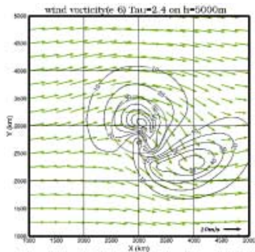
Fig.1(d) wind vector and vorticity distributions at \tau=2.4 , h=5000\text{m} , NO.01 U10m/s RUN1.
