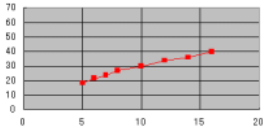
Fig.7(b) relation between cyclonic vorticity(row) and wind speed(column) at \tau = 3.0
