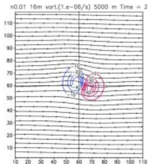
Fig.5(a) streamlines and vorticity at \tau = 0.6, N0.01, U16m on h5000m RUNs2
