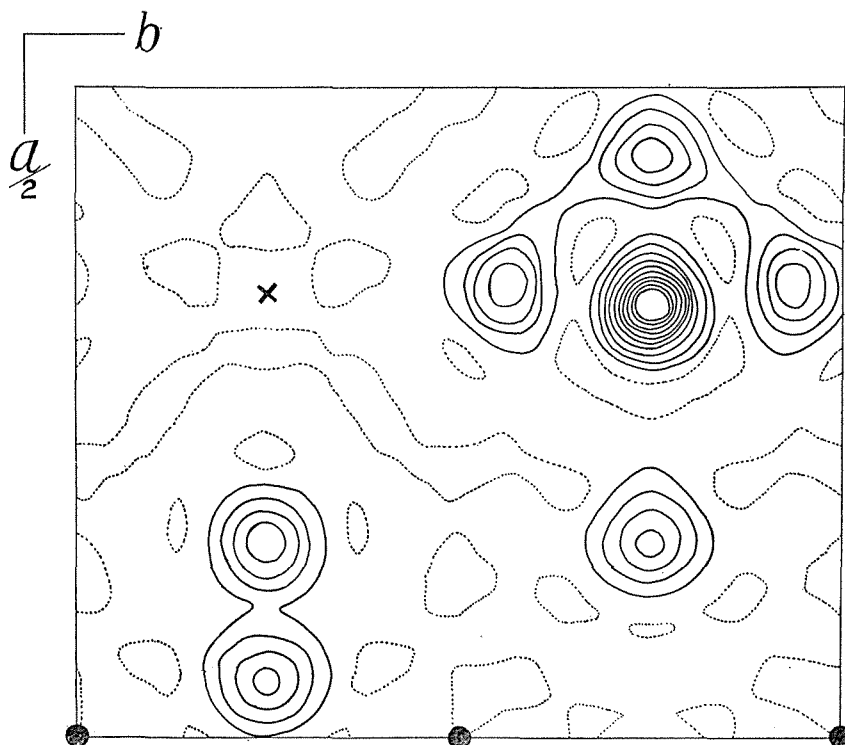
Fig. 4. The final difference synthesis projected on the (001) plane. Contours at 4\text{eA}^{-2} . Zero contours dotted. The positions of Pb and Cu atoms are marked by cross and solid circles respectively.
