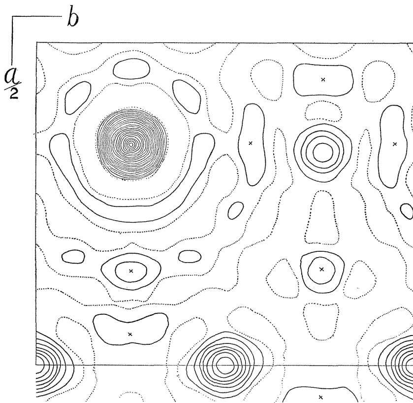
Fig. 2. Fourier map projected on the (001) plane. Contours at 10\text{e}\text{\AA}^{-2} . Zero contours dotted. The positions of O atoms and OH groups are indicated by crosses.
